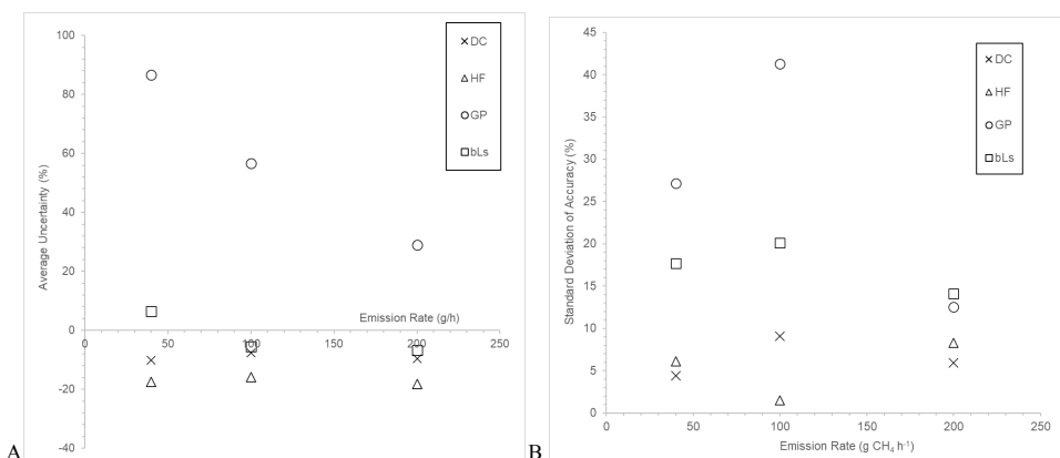
320 Figure 2 A) Average accuracy (% difference from known emission rate) of emission estimates from three repeat 325 measurements using each of the measurement methodologies at different known emission rates (~ 40, 100 and 200 g CH 4 h -1 ). B) The standard deviation of the uncertainties of repeated measurements against the emission rate of the experiment. Abbreviations as follows: DC – Dynamic chamber, HF – Hi Flow, GP – Gaussian Plume, bLS – Backwards Lagrangian stochastic method.
