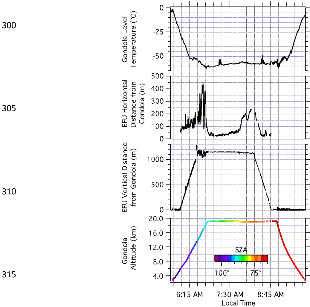
Figure 2: Summary of flight conditions of the 22 January 2021 WY933 zero pressure balloon flight. Altitude-adjusted solar zenith angle is displayed in rainbow.
