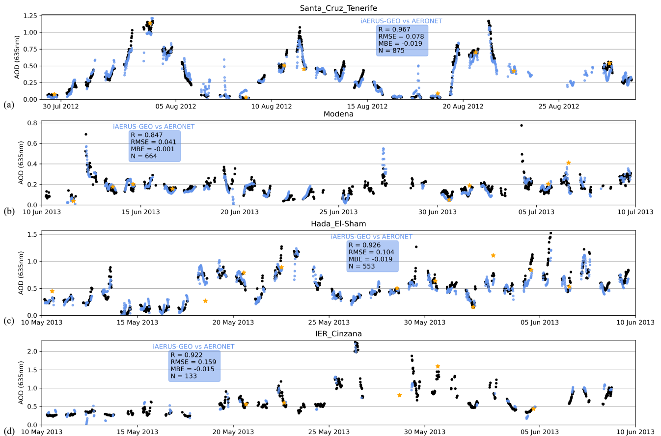
610 Figure 15. Time series of AOD from iAERUS-GEO (CM>2; in blue color), AERONET (in black color), and GRASP (in orange color) for sites (a) Santa_Cruz_Tenerife , (b) Modena , (c) Hada_El-Sham , and (d) IER_Cinzana during 1-month time periods in 2012 and 2013.
