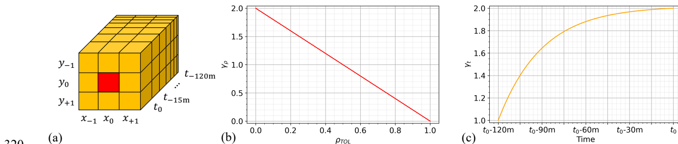
320 Figure 5. (a) Scheme of super-pixel with pixel to be processed in red color, (b) Weights depending on TOL reflectance when \max(\rho_{TOL}) = 1 and \min(\rho_{TOL}) = 0 , and (c) weights depending on acquisition time.
