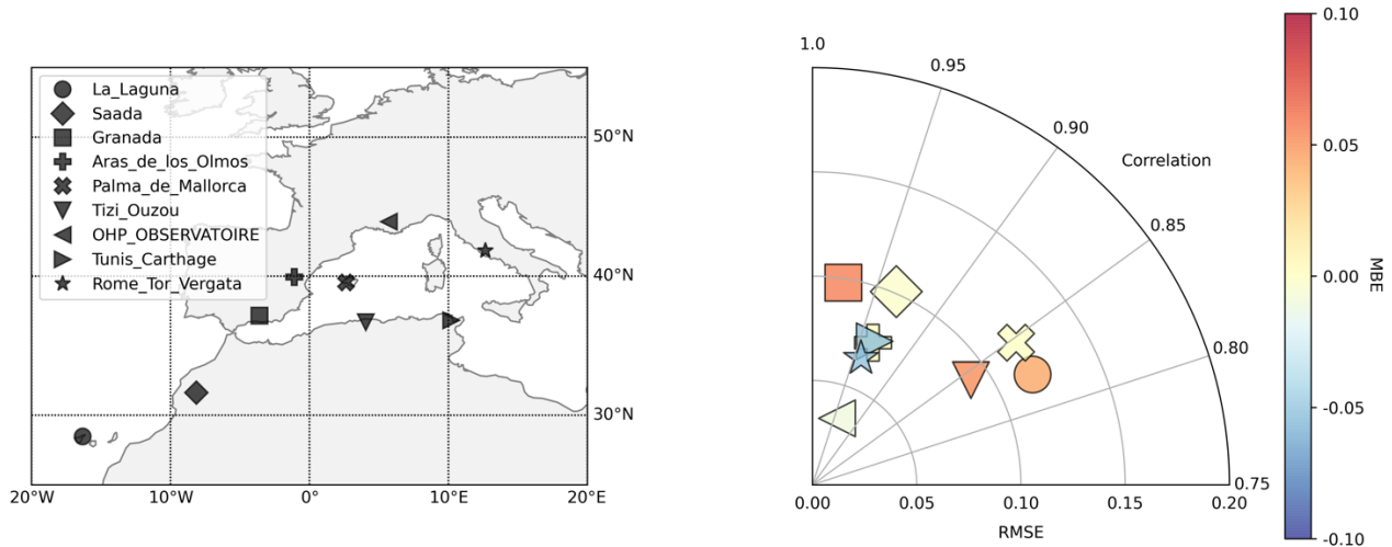
Figure 18. Assessment of iAERUS-GEO with AERONET during the dust event in July 2016. (left) Selected sites. (right) Average scores.
