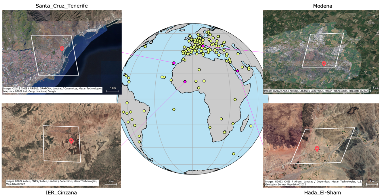
Figure 8. Location of AERONET sites used for the assessment of iAERUS-GEO. Sites for which times series are plotted in Sect. 4.4 are highlighted in pink color. The aerial view corresponding to these four sites is also shown, along with the location of the sunphotometer (red pin) and the approximate footprint of the corresponding SEVIRI pixel (white rhombus).
