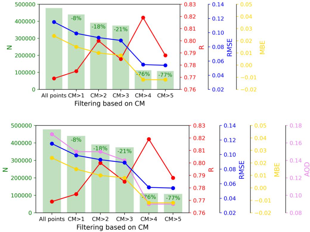
Figure 11. Variation of the averages scores (R, RMSE, MBE) obtained from the comparison to AERONET, average retrieved AOD , and the number of retrievals (N) according to an increasing filtering of iAERUS-GEO AOD-retrievals based on the confidence measure (CM).
