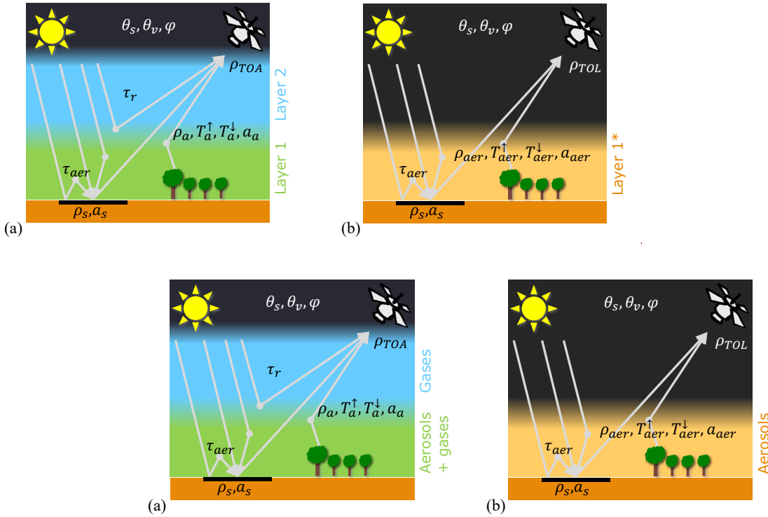
Figure 3. Atmosphere model and radiative parameters (a) before and (b) after correction for gas effects Rayleigh scattering and gas absorption . Subscripts “aer” and “a” are respectively used to distinguish between terms related to aerosols or to the whole atmosphere (aerosols plus gases). The aerosol layer is described by its optical properties and has not any actual height.
