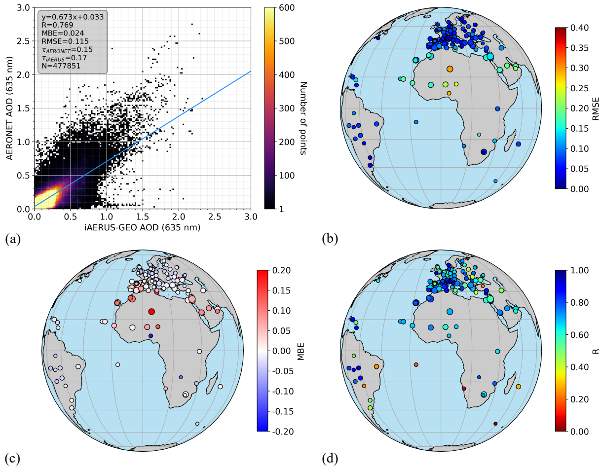
510 Figure 9. Assessment of iAERUS-GEO AOD retrievals from April 2012 to September 2013 with AERONET data. Comparison between the two data sets is illustrated by (a) a 2D histogram and maps showing the average (b) RMSE, (c) MBE, and (d) R obtained for each AERONET site. The size of dots in (b), (c), and (d) is proportional to the number of AOD retrievals.
