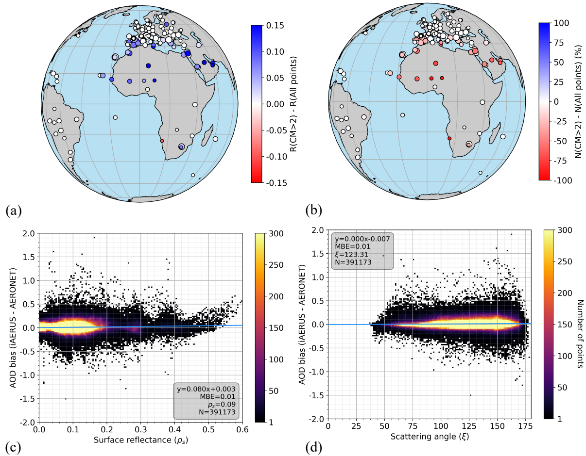
Figure 12. Evaluation of the AOD retrievals for the case “CM>2”. Score maps in (a) and (b) show the difference in R and N, with respect to the case with no filtering. 2D histograms in (c) and (d) show the relation between AOD bias and surface reflectance and scattering angle.
