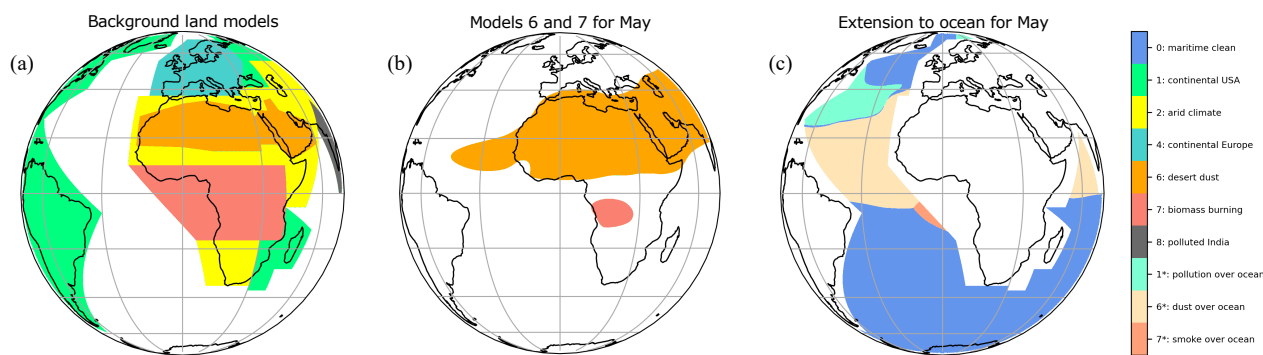
Figure C1. Construction of the aerosol model maps for May (Fig. 7) based on (a) the background land models superposed with (b) the extension of Models 6 and 7 beyond their initial boundaries and (c) the models for the remaining ocean pixels.
