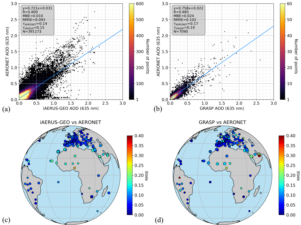
Figure 13. Assessment of two satellite AOD data sets with AERONET from April 2012 to September 2013. Comparison between iAERUS-GEO (CM>2) and AERONET is shown by (a) a 2D histogram and (c) a map showing the average RMSE per station. The same plots are given for the comparison between GRASP and AERONET in (b) and (d). Note the different color bar scale in (a) and (b).
