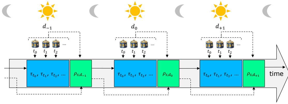
145 Figure 2. Nesting of daily and instantaneous processing during the days ( d_k ). Daily retrieval of surface BRDF ( \rho_s ) is shown with dashed lines and green color boxes. Instantaneous retrieval of AOD ( \tau ) at every time slot ( t_j ) is illustrated with solid arrows and blue color boxes.
