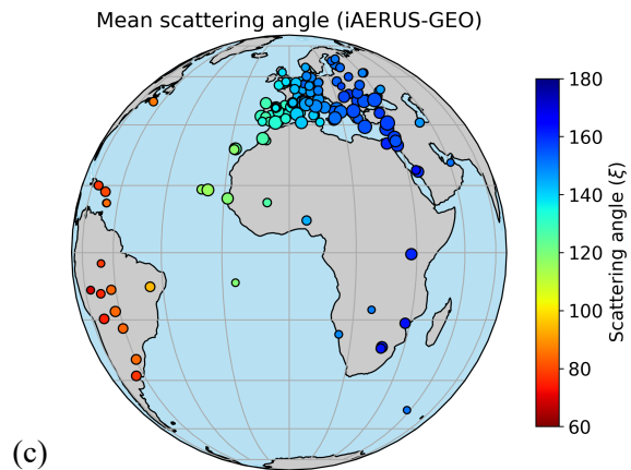
585 Figure 14. Comparison between iAERUS-GEO (CM>2) and GRASP by (a) a 2D histogram and (b) a map giving the average R for each AERONET site. The average scattering angle of the iAERUS-GEO retrievals considered in this comparison is given in (c).
