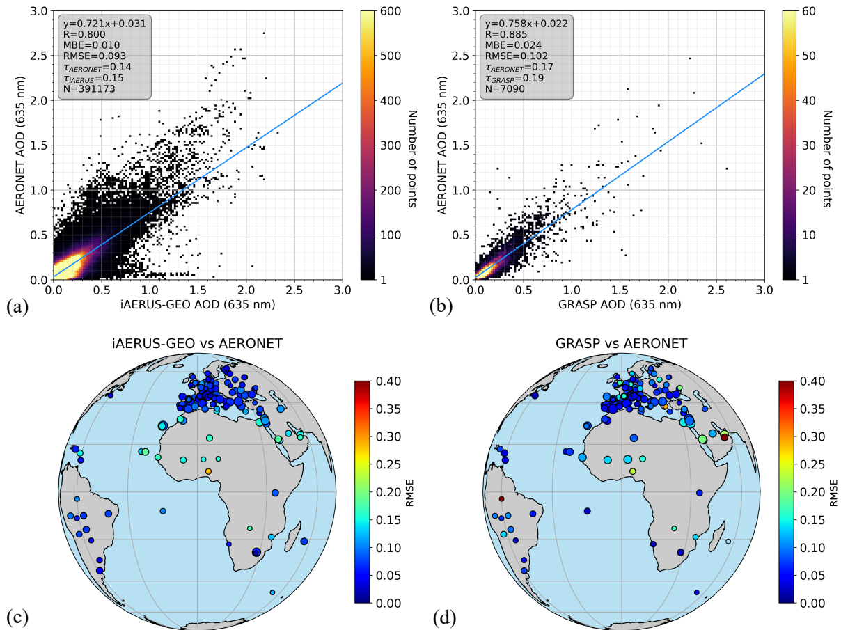
540 Figure 13. Assessment of two satellite AOD data sets with AERONET from April 2012 to September 2013. Comparison between iAERUS-GEO (CM>2) and AERONET is shown by (a) a 2D histogram and (c) a map showing the average RMSE per station. The same plots are given for the comparison between GRASP and AERONET in (b) and (d). Note the different color bar scale in (a) and (b).
