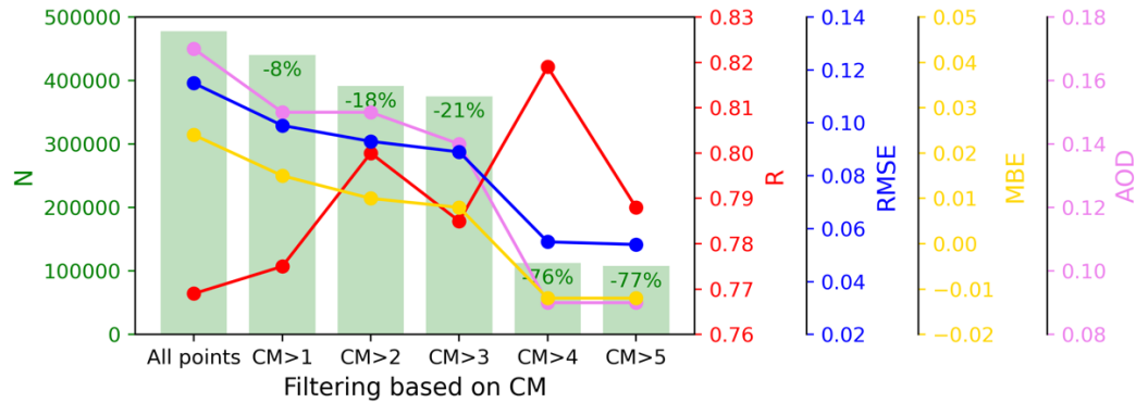
Figure 11. Variation of the averages scores (R, RMSE, MBE) obtained from the comparison to AERONET, average retrieved AOD, and number of retrievals (N) according to an increasing filtering of iAERUS-GEO retrievals based on the confidence measure (CM).
