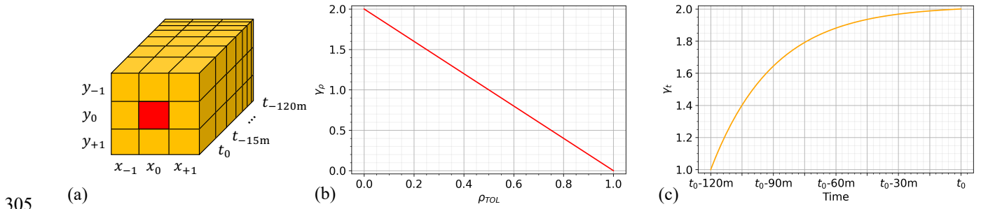
Figure 5. (a) Scheme of super-pixel with pixel to be processed in red color, (b) Weights depending on TOL reflectance when \max(\rho_{TOL}) = 1 and \min(\rho_{TOL}) = 0 , and (c) weights depending on acquisition time.
