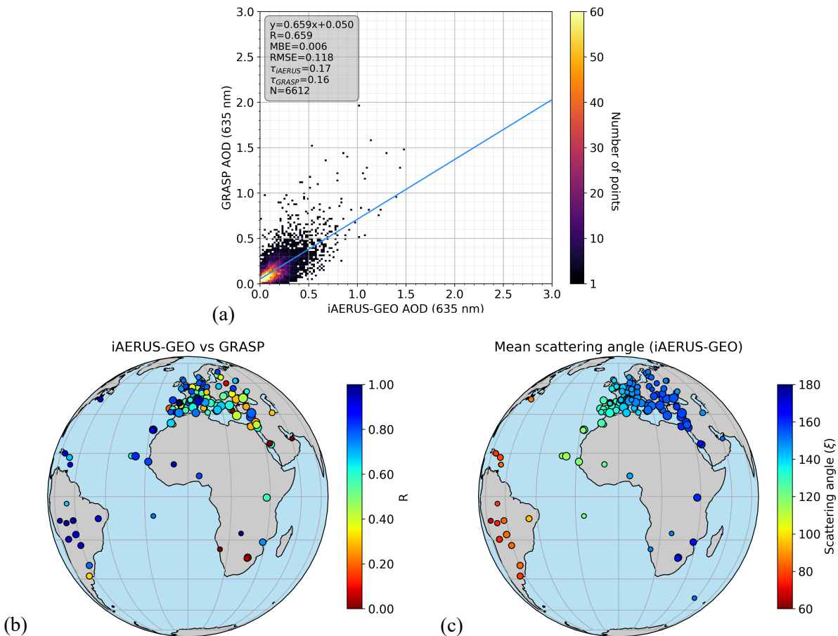
555 Figure 14. Comparison between iAERUS-GEO (CM>2) and GRASP by (a) a 2D histogram and (b) a map giving the average R for each AERONET site. The average scattering angle of the iAERUS-GEO retrievals considered in this comparison is given in (c).
