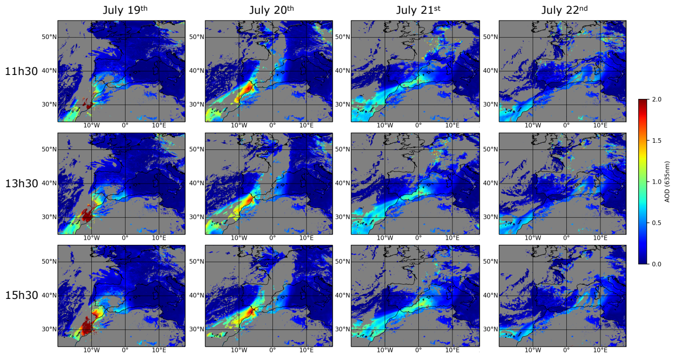
605 Figure 17. AOD from iAERUS-GEO at (top) 11:30 a.m., (middle) 1:30 p.m., and (bottom) 3:30 p.m. for four consecutive days in July 2016.
