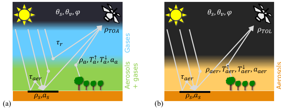
175 Figure 3. Atmosphere model and radiative parameters (a) before and (b) after correction for Rayleigh scattering and gas absorption. Subscripts aer and a are respectively used to distinguish between terms related to aerosols or to the whole atmosphere (aerosols plus gases). The aerosol layer is described by its optical properties and has not any actual height.
