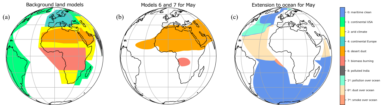
760 Figure C1. Construction of the aerosol model maps for May (Fig. 7) based on (a) the background land models superposed with (b) the extension of Models 6 and 7 beyond their initial boundaries and (c) the models for the remaining ocean pixels.
