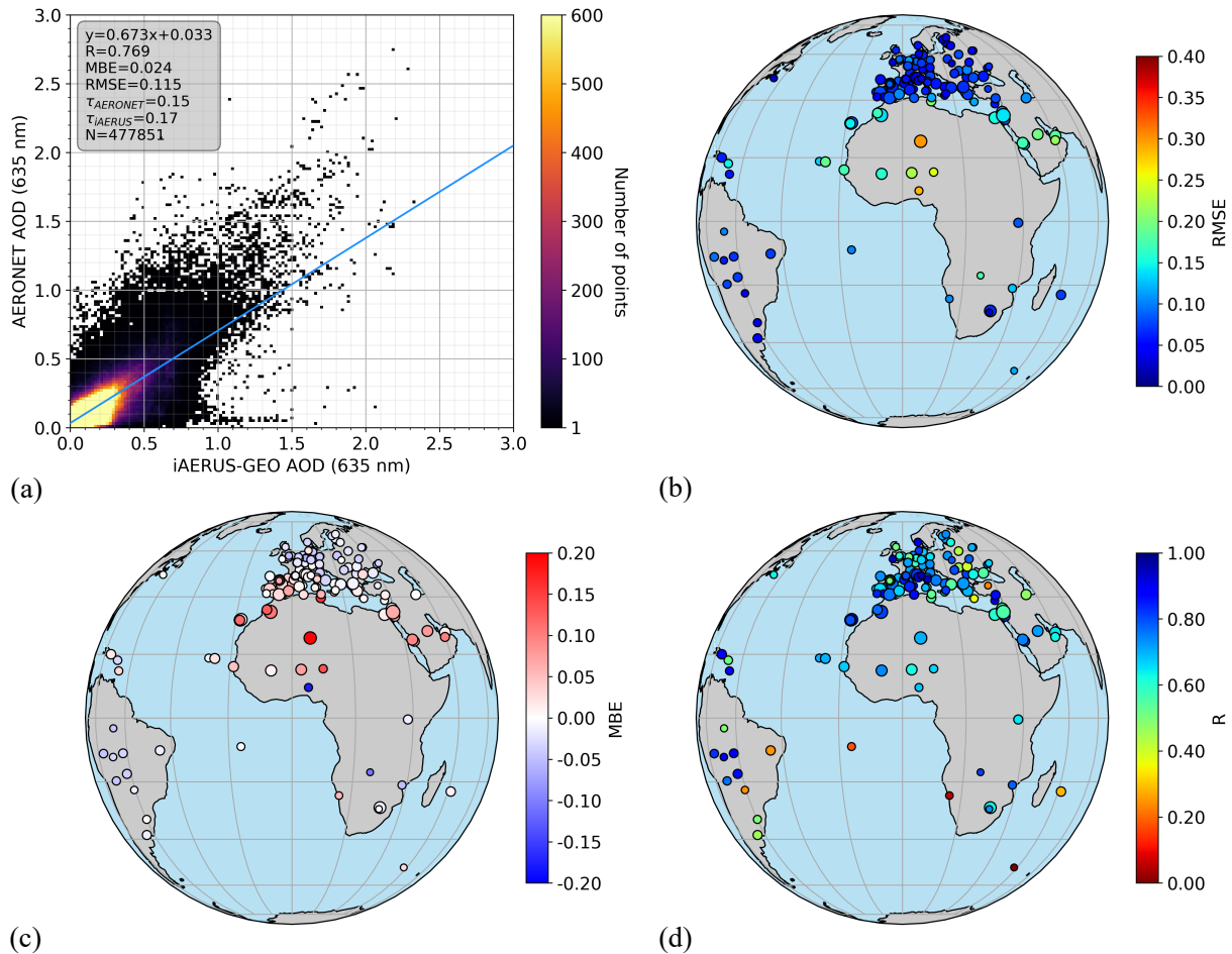
485 Figure 9. Assessment of iAERUS-GEO AOD retrievals from April 2012 to September 2013 with AERONET data. Comparison between the two data sets is illustrated by (a) a 2D histogram and maps showing the average (b) RMSE, (c) MBE, and (d) R obtained for each AERONET site. The size of dots in (b), (c), and (d) is proportional to the number of AOD retrievals.
