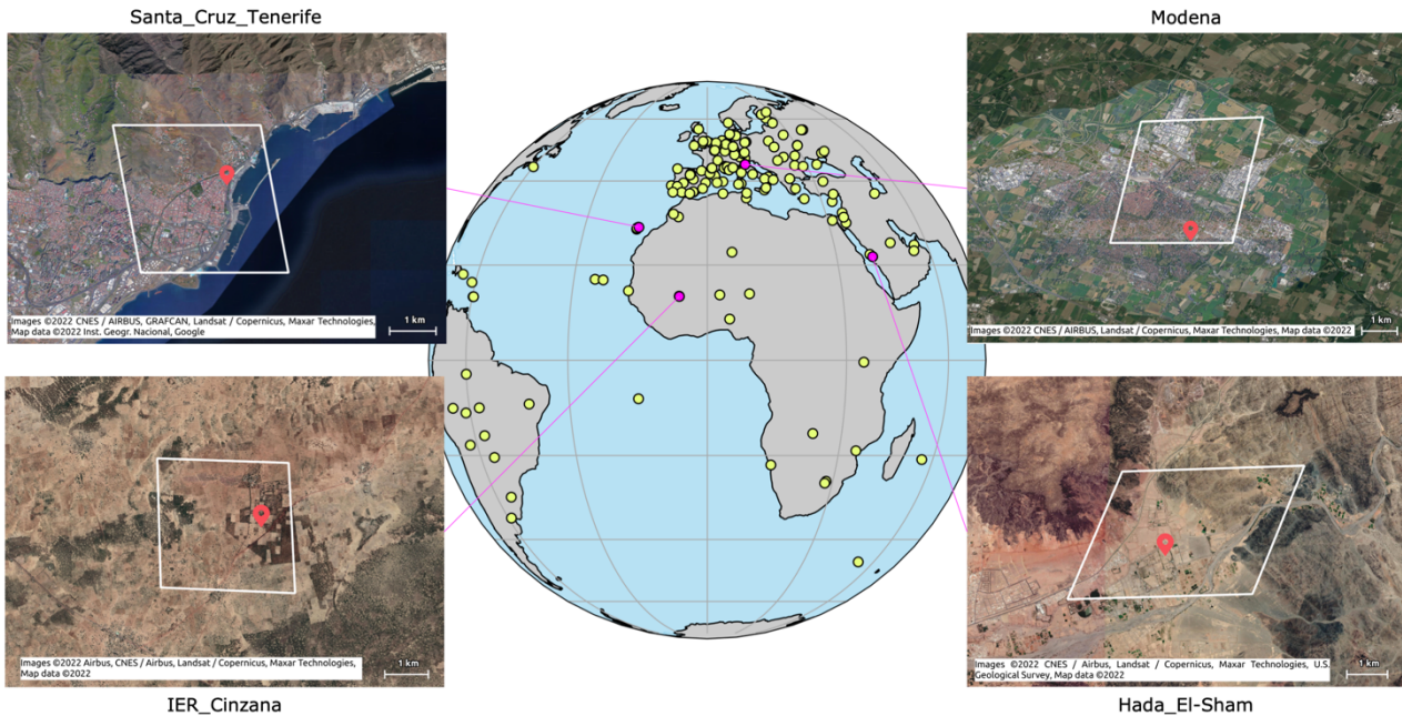
440 Figure 8. Location of AERONET sites used for the assessment of iAERUS-GEO. Sites for which times series are plotted in Sect. 4.4 are highlighted in pink color. The aerial view corresponding to these four sites is also shown, along with the location of the sunphotometer (red pin) and the approximate footprint of the corresponding SEVIRI pixel (white rhombus).
