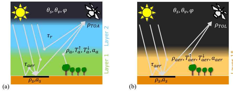
170 Figure 3. Atmosphere model and radiative parameters (a) before and (b) after correction for gas effects. Subscripts “aer” and “a” are respectively used to distinguish between terms related to aerosols or to the whole atmosphere (aerosols plus gases).
