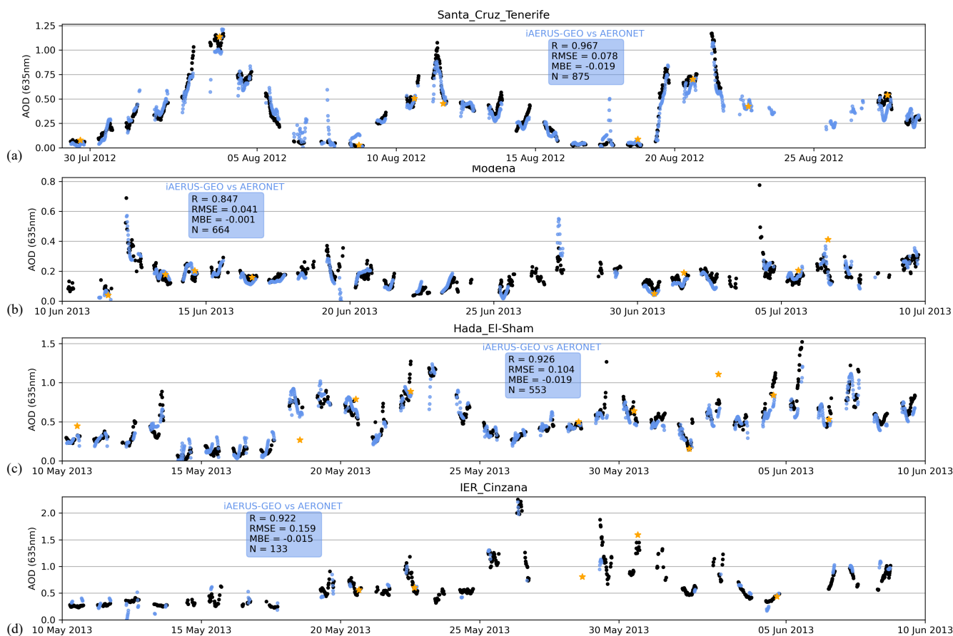
Figure 15. Time series of AOD from iAERUS-GEO (CM>2; in blue color), AERONET (in black color), and GRASP (in orange color) for sites (a) Santa_Cruz_Tenerife , (b) Modena , (c) Hada_El-Sham , and (d) IER_Cinzana during 1-month time periods in 2012 and 2013.
