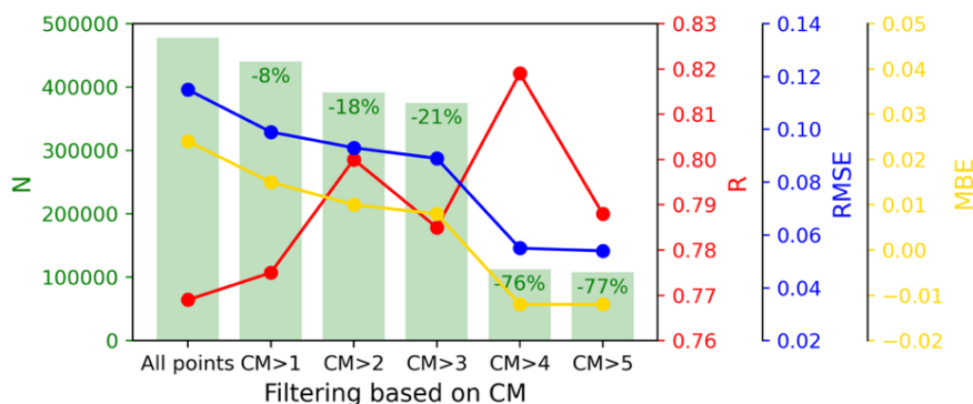
Figure 11. Variation of the averages scores (R, RMSE, MBE) obtained from the comparison to AERONET and the number of retrievals (N) according to an increasing filtering of iAERUS-GEO AOD retrievals based on the confidence measure (CM).
