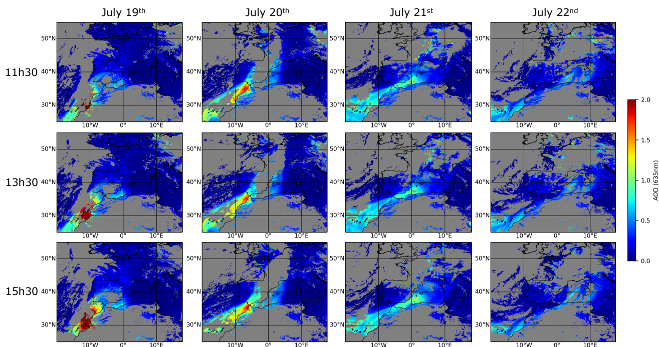
Figure 17. AOD from iAERUS-GEO at (top) 11:30 a.m., (middle) 1:30 p.m., and (bottom) 3:30 p.m. for four consecutive days in July 2016.
