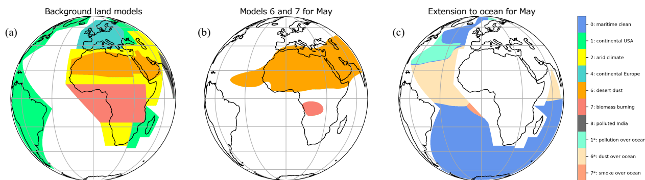
730 Figure C1. Construction of the aerosol model maps for May (Fig. 7) based on (a) the background land models superposed with (b) the extension of Models 6 and 7 beyond their initial boundaries and (c) the models for the remaining ocean pixels.
