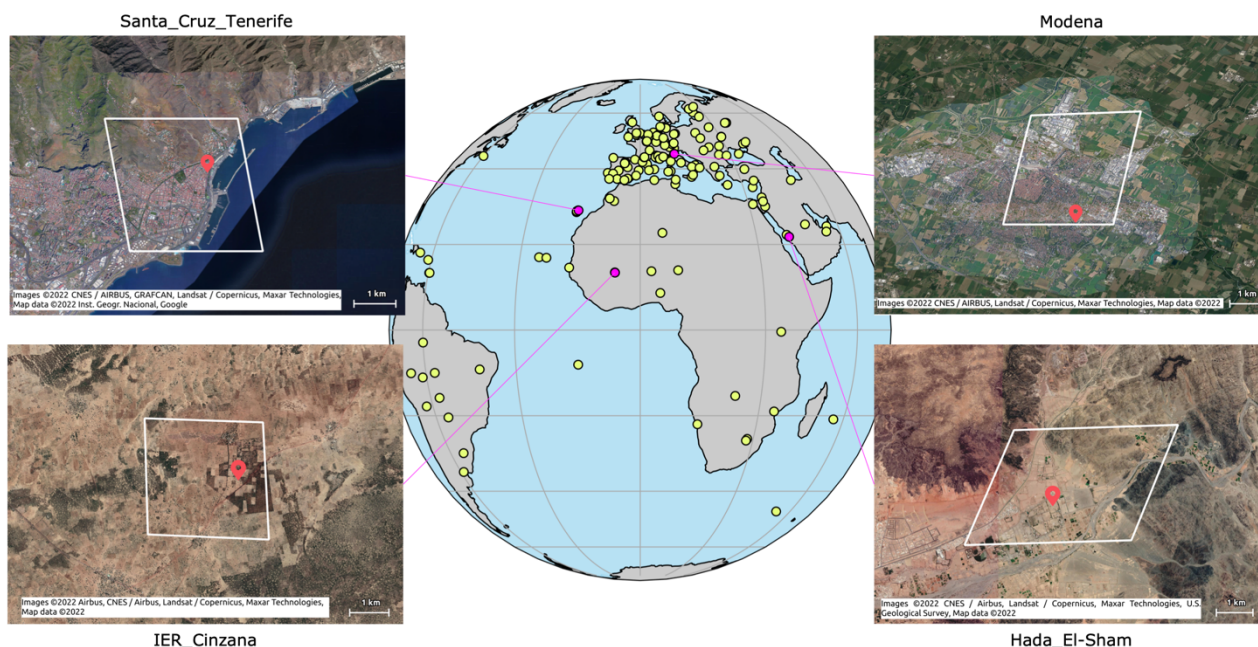
420 Figure 8. Location of AERONET sites used for the assessment of iAERUS-GEO. Sites for which time series are plotted in Sect. 4.4 are highlighted in pink color. The aerial view corresponding to these four sites is also shown, along with the location of the sunphotometer (red pin) and the approximate footprint of the corresponding SEVIRI pixel (white rhombus).
