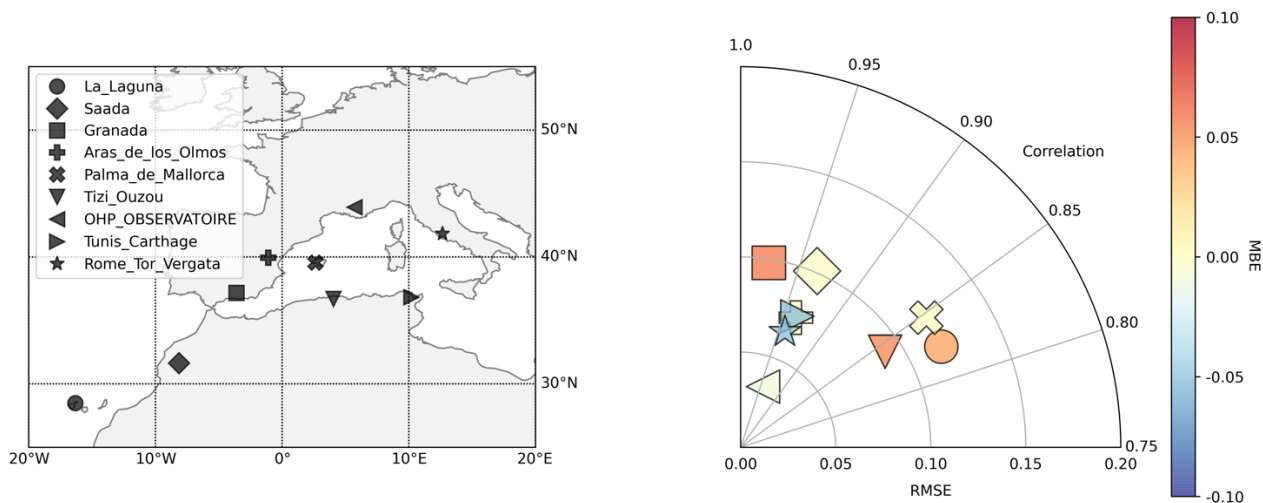
Figure 18. Assessment of iAERUS-GEO with AERONET during the dust event in July 2016. (left) Selected sites. (right) Average scores.
