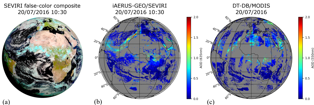
Figure 16. (a) Color composite of SEVIRI radiance images acquired at 10:30 a.m. on July 20 th , 2016. (b) Map of AOD retrieved by iAERUS-GEO from SEVIRI on the same date and time. (c) Map of AOD retrieved by DT-DB from MODIS-Terra on the same date.
