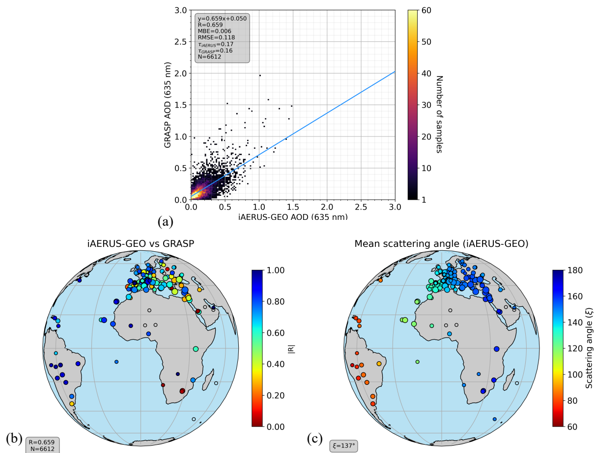
530 Figure 14. Comparison between iAERUS-GEO (CM>2) and GRASP by (a) a 2D histogram and (b) a map giving the average R for each AERONET site. The average scattering angle of the iAERUS-GEO retrievals considered in this comparison is given in (c).
