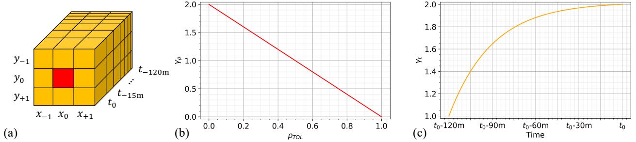
295 Figure 5. (a) Scheme of super-pixel with pixel to be processed in red color, (b) Weights depending on TOL reflectance when \max(\rho_{TOL}) = 1 and \min(\rho_{TOL}) = 0 , and (c) weights depending on acquisition time.
