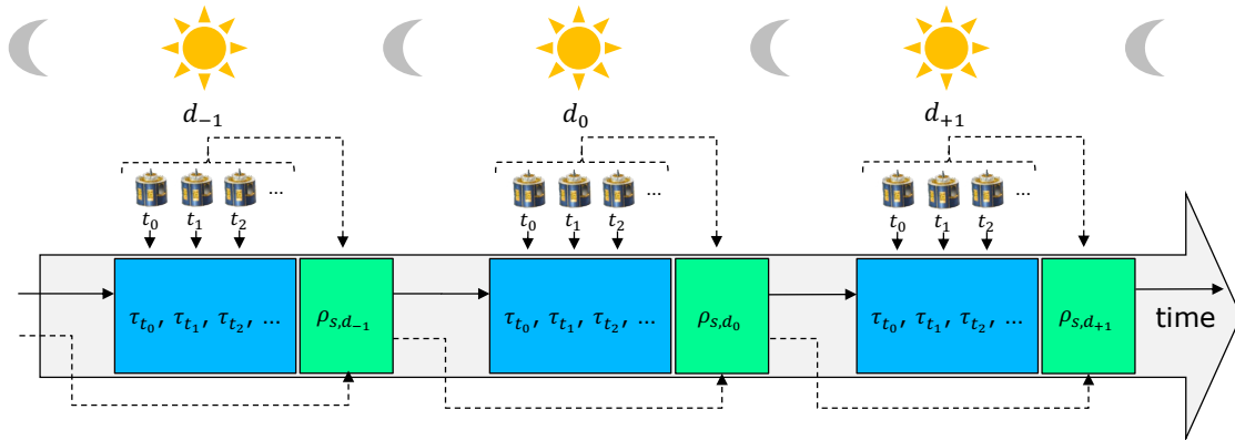
Figure 2. Nesting of daily and instantaneous processing during the days ( d_k ). Daily retrieval of surface BRDF ( \rho_s ) is shown with dashed lines and green color boxes. Instantaneous retrieval of AOD ( \tau ) at every time slot ( t_j ) is illustrated with solid arrows and blue color boxes.
