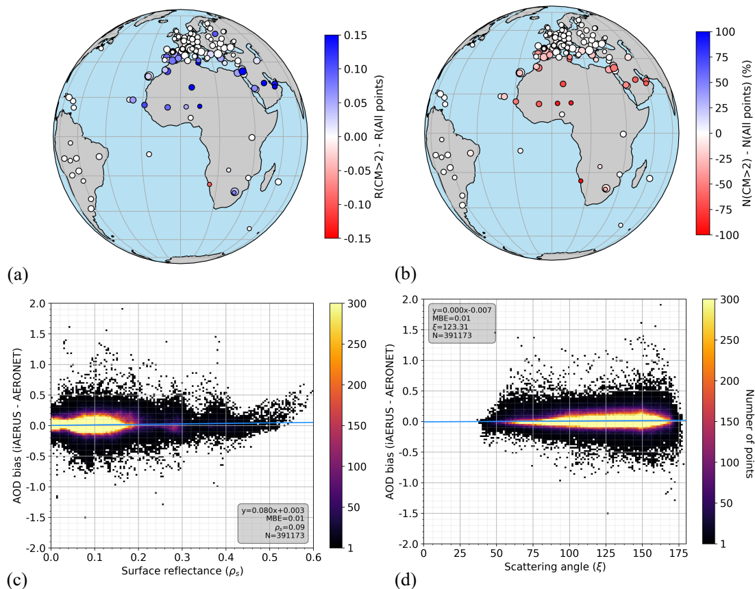
500 Figure 12. Evaluation of the AOD retrievals for the case “CM>2”. Score maps in (a) and (b) show the difference in R and N, with respect to the case with no filtering. 2D histograms in (c) and (d) show the relation between AOD bias and surface reflectance and scattering angle.
