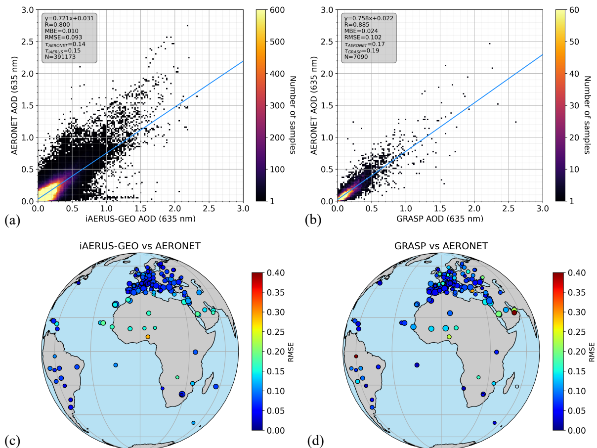
515 Figure 13. Assessment of two satellite AOD data sets with AERONET from April 2012 to September 2013. Comparison between iAERUS- GEO (CM>2) and AERONET is shown by (a) a 2D histogram and (c) a map showing the average RMSE per station. The same plots are given for the comparison between GRASP and AERONET in (b) and (d). Note the different color bar scale in (a) and (b).
