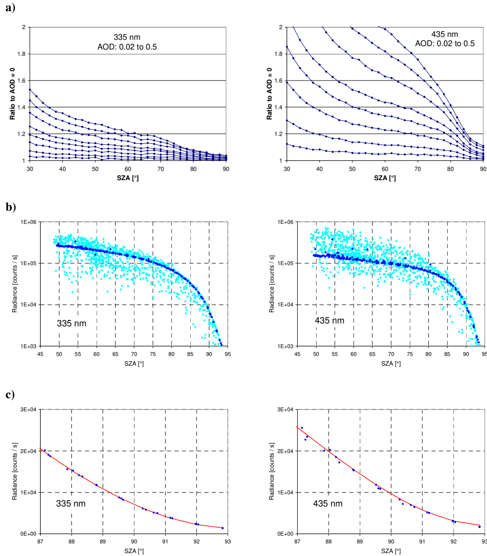
460 Fig. 1 a) Ratio of the simulated zenith radiance for different aerosol optical depths to the radiance for an atmosphere without aerosols as function of the SZA for 335 nm (left) and 435 nm (right). Data are taken from Fig. 5 in Wagner et al. (2015). In that study simulations were only performed for SZA up to 90°. AOD values are 0.02, 0.05, 0.1, 0.15, 0.2, 0.3, 0.4, 0.5. At 90° SZA, the variation of the radiance is smallest (about 4 % at 335 nm and 11 % at 435 nm). b) 465 measured zenith radiances from 19 September to 18 October 2022 in Mainz, Germany, for all sky conditions (light blue) and clear sky conditions (dark blue). c) radiances during cloud-free conditions together with a fitted polynomial (for SZA between 85° and 93°). Note that in Fig. 1b a logarithmic y-axis is used, because the data span more than two orders of magnitude.
