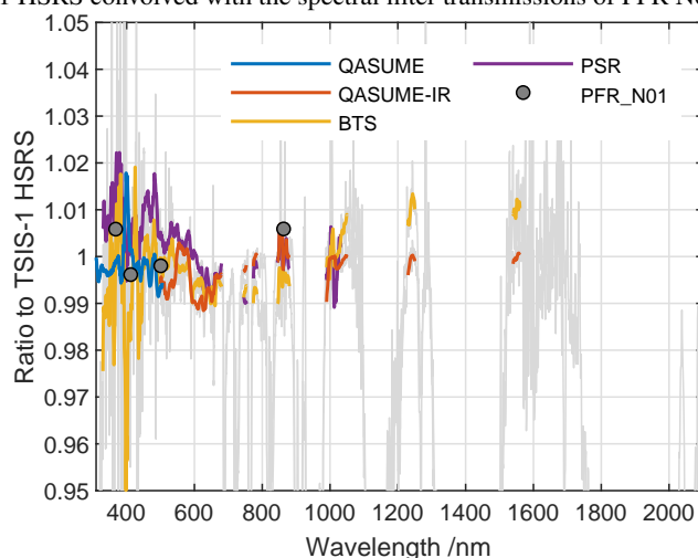
Figure 3. Spectral ratio of the zero airmass extrapolated ToA solar spectra from QASUME (blue), QASUME-IR (red), PSR (violet), and BTS (yellow) relative to the TSIS-1 HSRS solar spectrum convolved with the respective line spread functions of the spectroradiometers. The coloured lines are a 10 nm moving average of the spectral ratios in spectral regions with no or only weak atmospheric trace gas absorption, while the gray line represents the full spectral ratio of BTS to TSIS-1 HSRS. The gray circles represent the ratios of the spectral solar irradiances of PFR N01 with TSIS-1 HSRS convolved with the spectral filter transmissions of PFR N01.
