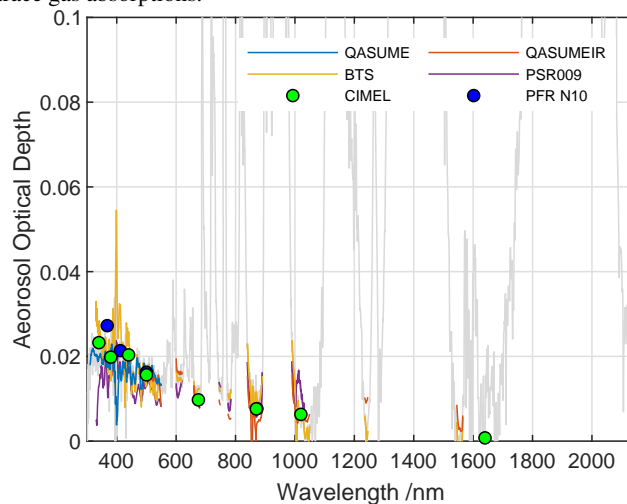
Figure 7. Spectral Aerosol Optical Depth from QASUME (blue), QASUME-IR (red), BTS (yellow), PSR (violet) from measurements obtained on 13 September 2022 at 16:00 UTC. The circles are from the PFR (blue), and CIMEL (green) sunphotometers. The gray curve represents the complete spectral optical depth over the whole spectral interval measured by the spectroradiometers, including spectral regions also contaminated by unaccounted trace gas absorptions.
