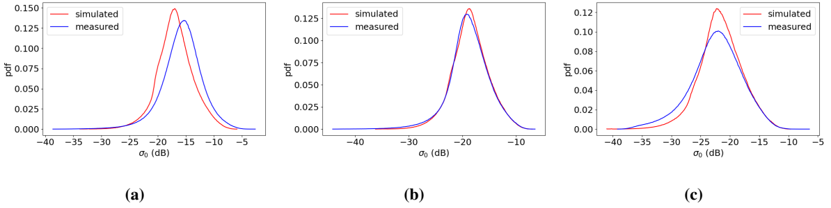
Figure 6. C-band measured \sigma^0 and simulated \sigma^0 PDF distribution per incidence angle, data from 1 Dec - 31 Dec 2022 ascending orbits: (a) HH incidence 34^\circ , (b) HH incidence 38^\circ , (c) HH incidence 44^\circ .
