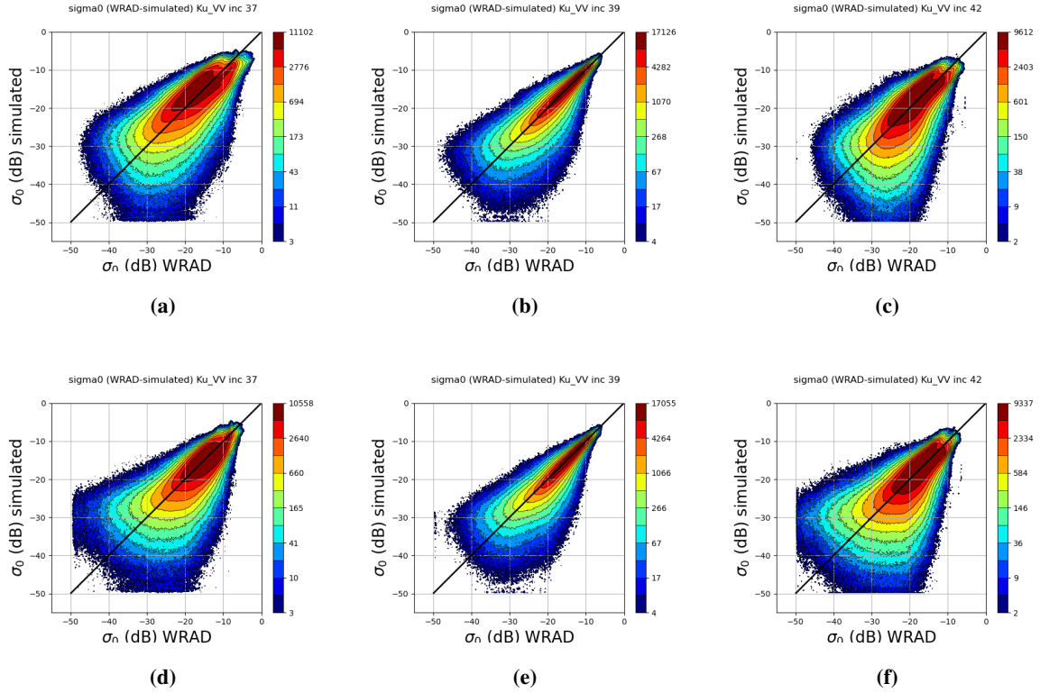
Figure 8. Ku-band VV polarization, measured \sigma^\circ and simulated \sigma^\circ joint distribution per incidence angle, data from 1 Dec - 31 Dec 2022 ascending orbits, upper panel is original distribution, the lower panel is HOC calibrated: (a) original at incidence 37^\circ , (b) original at incidence 39^\circ , (c) original at incidence 42^\circ , (d) HOC calibrated at incidence 37^\circ , (e) HOC calibrated at incidence 39^\circ , (f) HOC calibrated at incidence 42^\circ .
