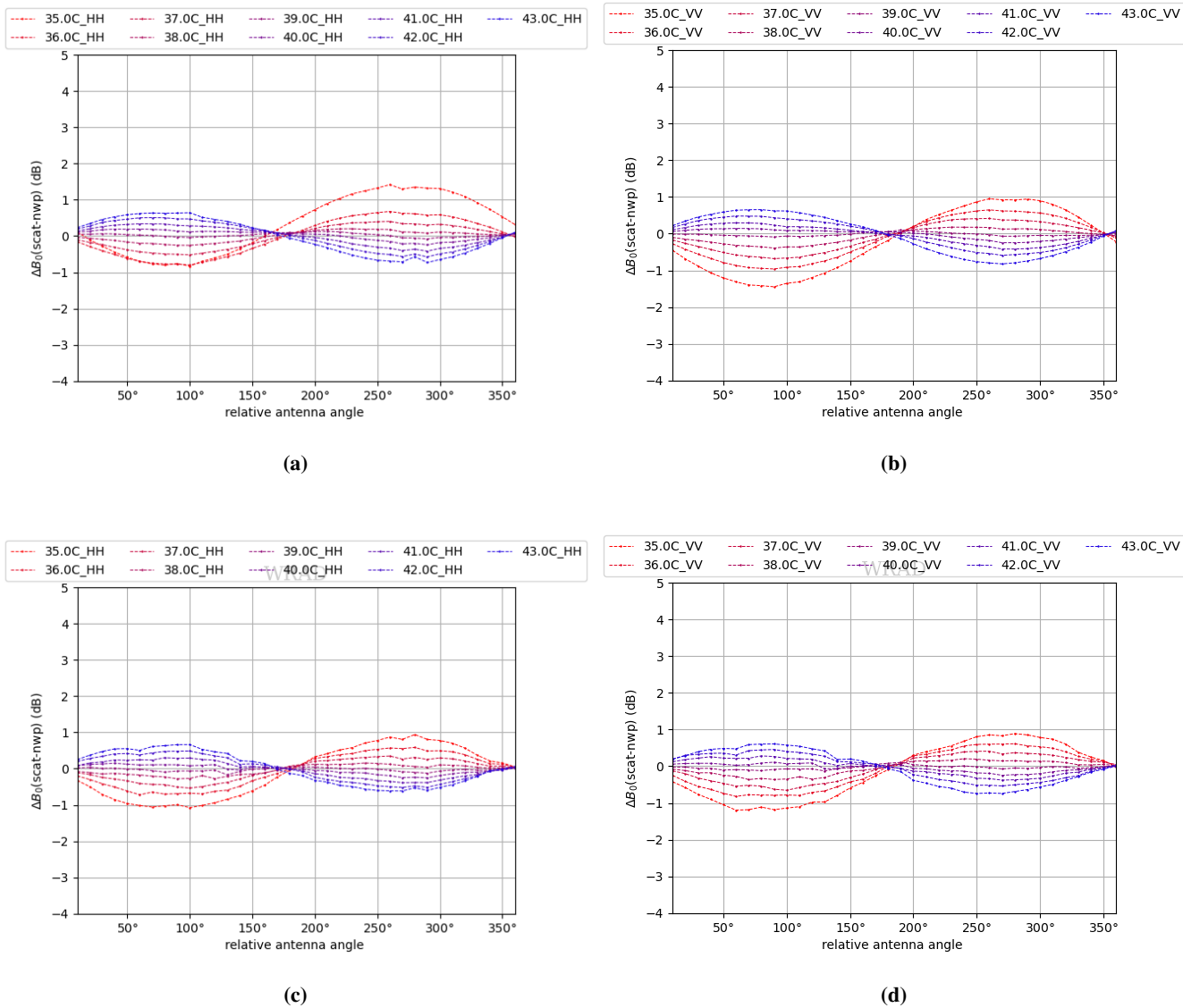
Figure 14. C-band NOCant, ascending orbits, data from 10 Dec - 19 Dec 2022: (a) NOCant HH without HOC, (b) NOCant VV without HOC, (c) NOCant HH after HOC, (d) NOCant VV after HOC.
