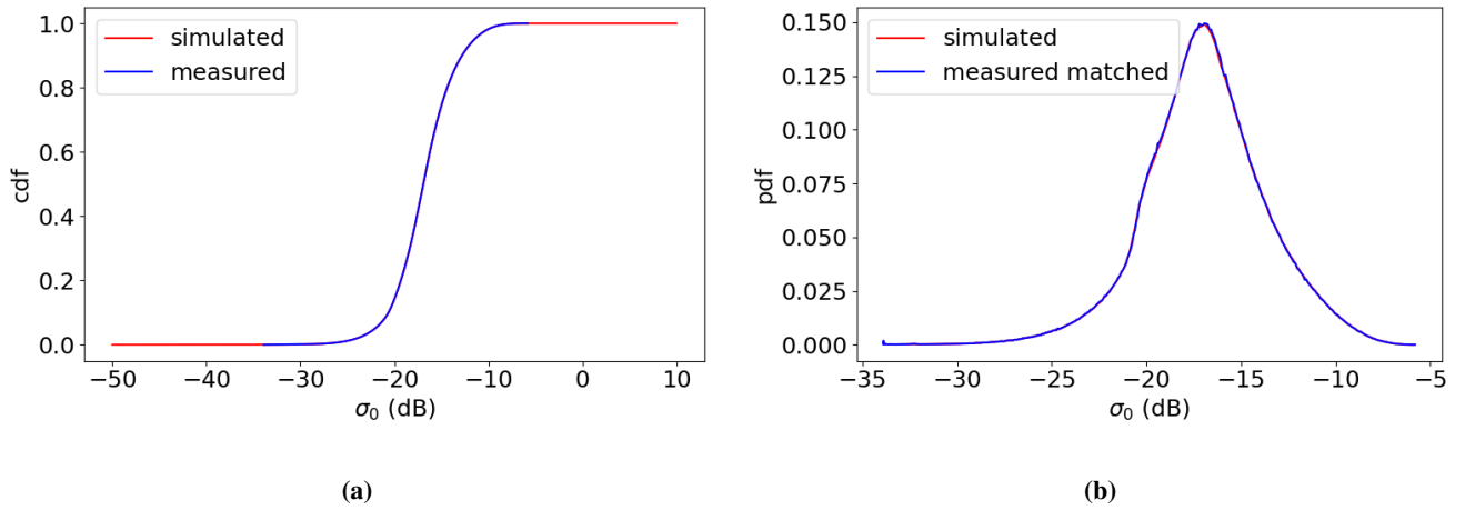
Figure 7. C-band HH measured \sigma^0 and simulated \sigma^0 matched CDF and PDF distribution at incidence 34^\circ (the other incidence angles are the same pattern, thus not shown here), data from 1 Dec - 31 Dec 2022 ascending orbits, (a) matched CDF; (b) matched PDF.
