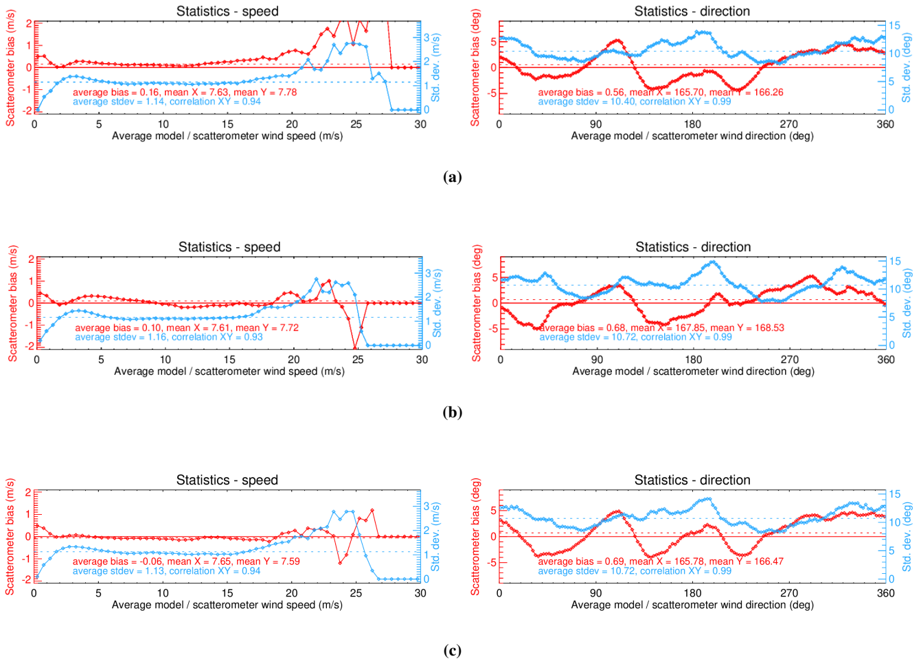
Figure 20. Ku-band wind speed/direction bias and their corresponding SDD as a function of wind speed/direction, data from 1 Dec to 10 Dec 2022, ascending orbits (a) NOCant; (b) HOC; (c) HOC&NOCant.
