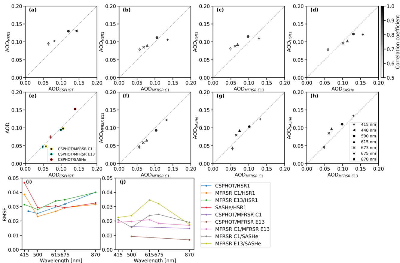
510 Figure 11: Mean AOD (black) of collocated (a) CSPHOT and HSR1, (b) MFRSR C1 and HSR1, (c) MFRSR E13 and HSR1, (d) SASHe and HSR1, (f) MFRSR C1 and MFRSR E13, (g) MFRSR C1 and SASHe, and (h) MFRSR E13 and SASHe. The shading indicates the correlation coefficient. Mean AOD of collocated CSPHOT with MFRSR C1 (yellow outline), MFRSR E13 (light blue outline), and SASHe (red outline) are shown in (e). The wavelengths considered include 415 (plus sign), 440 (left pointing triangle), 500 (circle), 615 (triangle), 673 (x-mark), 675 (star), and 870 (diamond) nm. The 1:1 line is indicated by the dotted gray line. Root mean square error (RMSE) are shown for (i) HSR1 AOD and other instruments, and (j) other instruments between each other.
