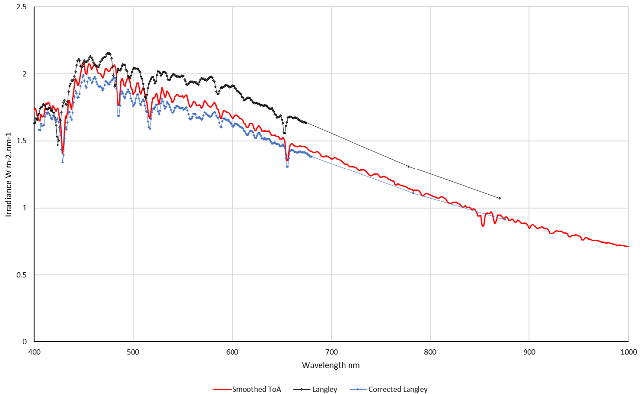
Figure 14: Extra-terrestrial spectral irradiance from SMARTS2 (red), the Langley intercept values as calculated from the original HSR1 measurements (black), and the Langley intercept values adjusted according to the post-deployment calibration check with wavelengths adjusted to match the SMARTS2 spectral features (blue).
