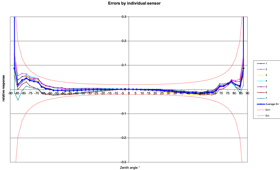
135 Figure 3: Cosine curve for the 7 sensors of the HSR1. Heavy blue line shows an average of these, and the red lines show 2% design limits.
