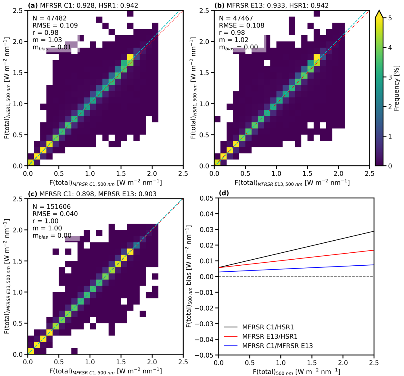
Figure 6: Frequency histogram for F_{total} at 500 nm ( \text{W m}^{-2} \text{ nm}^{-1} ) of collocated (a) MFRSR C1 and HSR1, (b) MFRSR E13 and HSR1, and (c) MFRSR C1 and MFRSR E13. The mean values are given above each plot. The sample size ( N ), root mean squared error (RMSE), correlation coefficient ( r ), regression line slope ( m ), and bias regression line slope ( m_{bias} ) are shown in the top left of each plot. The 1:1 line is indicated by the dotted red line and the regression line is indicated by the dashed light blue line. (d) The regression lines of the bias are shown for MFRSR C1 and HSR1 (black), MFRSR E13 and HSR1 (red), and MFRSR C1 and MFRSR E13 (blue). The zero line is indicated by the dashed gray line.
