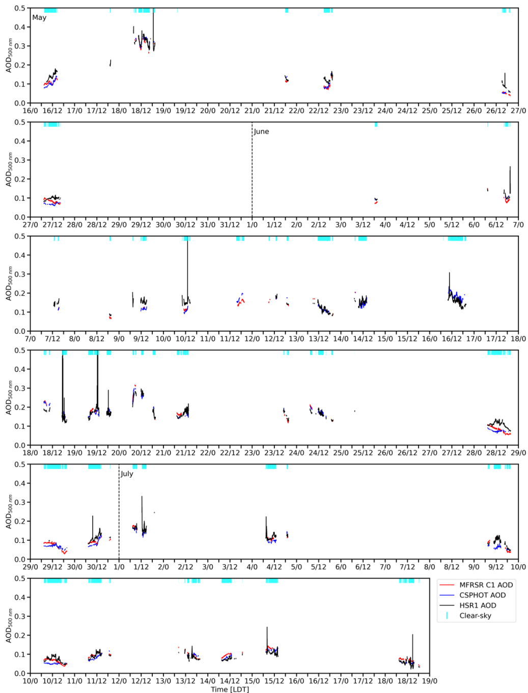
255 Figure 5: Time series (in LDT) of the AOD at 500 nm. The MFRSR C1 AOD (red), CSPHOT AOD (blue), and HSR1 AOD (black) are shown for clear-sky periods only. The light blue vertical lines indicate clear-sky periods. The dashed vertical black lines indicate the start of each month and the x-axis tick marks indicate the day and hour.
