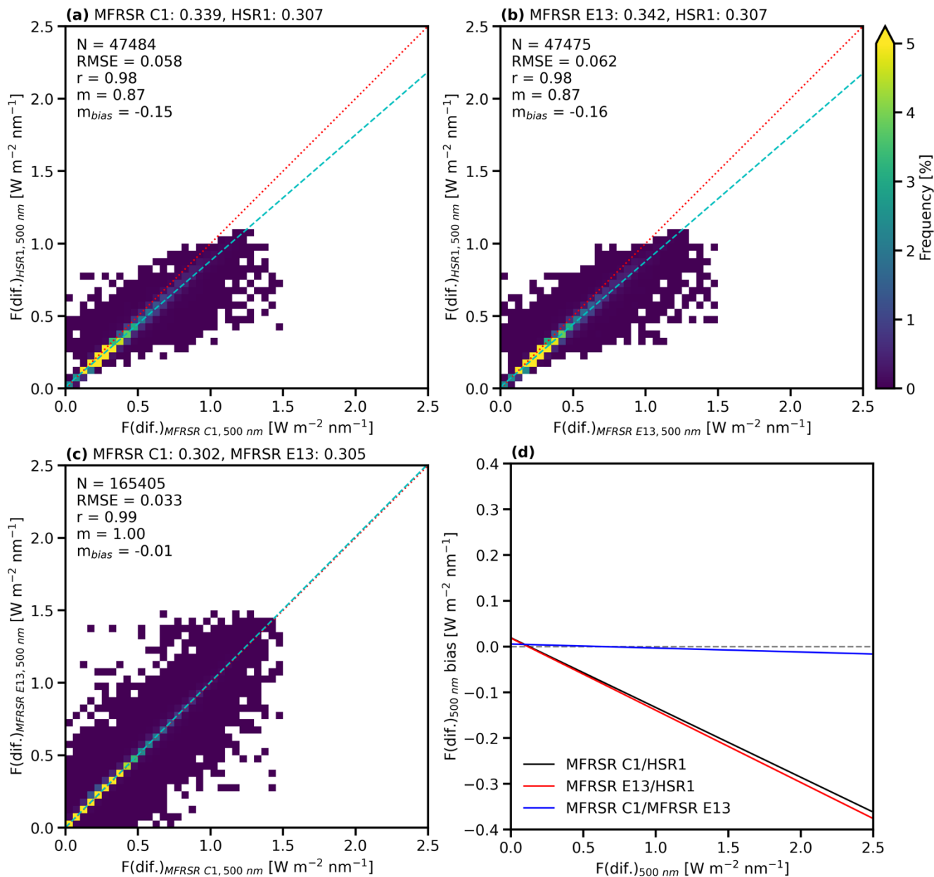
Figure 7: The same as Figure 6 but for F_{diffuse} at 500 nm.
