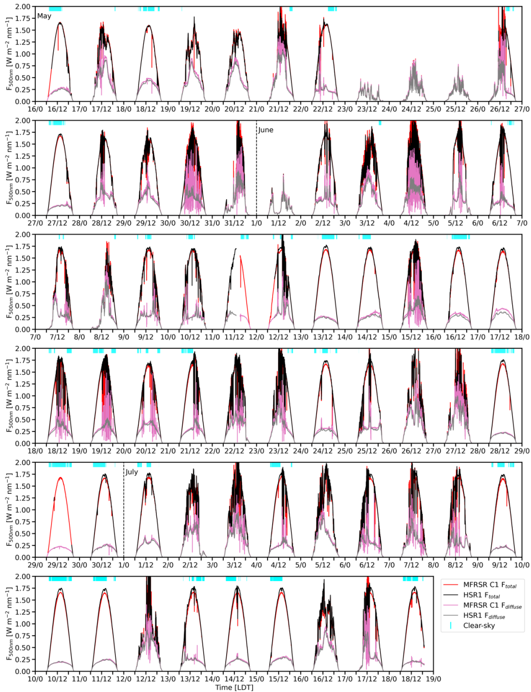
250 Figure 4: Time series in LDT of the F_{total} and F_{diffuse} at 500 nm ( \text{W m}^{-2} \text{nm}^{-1} ). The MFRSR C1 F_{total} (red), HSR1 F_{total} (black), MFRSR C1 F_{diffuse} (pink), and HSR1 F_{diffuse} (gray) are shown. The light blue vertical lines indicate clear-sky periods. The dashed vertical black lines indicate the start of each month and the x-axis tick marks indicate the day and hour.
