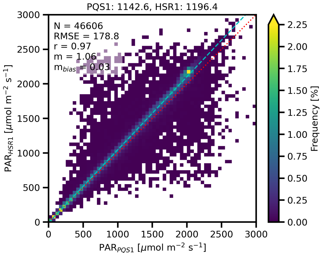
815 Figure B1: Frequency histogram for collocated PAR ( \mu\text{mol m}^{-2} \text{s}^{-1} ) between the PQS1 and the HSR1. The mean values are given above the plot and the sample size ( N ), root mean square error (RMSE), correlation coefficient ( r ), regression line slope ( m ), and bias regression line slope ( m_{bias} ) are shown in the top left. The 1:1 line is indicated by the dotted red line and the regression line is indicated by the dashed light blue line.
