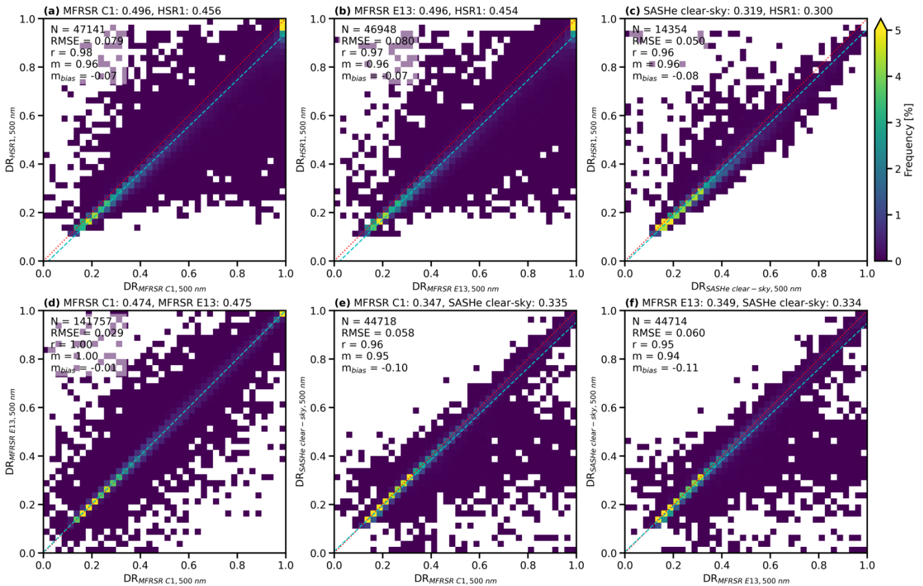
510 Figure 11: Frequency histogram for the diffuse ratio at 500 nm of collocated (a) MFRSR C1 and HSR1, (b) MFRSR E13 and HSR1, (c) SASHe and HSR1, (d) MFRSR C1 and MFRSR E13, (e) MFRSR C1 and SASHe, and (f) MFRSR E13 and SASHe. The 515 mean values are given above each plot. The sample size (N), root mean square error (RMSE), correlation coefficient (r), regression line slope (m), and bias regression line slope ( m_{bias} ) are shown in the top left of each plot. The 1:1 line is indicated by the dotted red line and the regression line is indicated by the dashed light blue line. Note that SASHe diffuse ratios are limited to clear-sky conditions.
