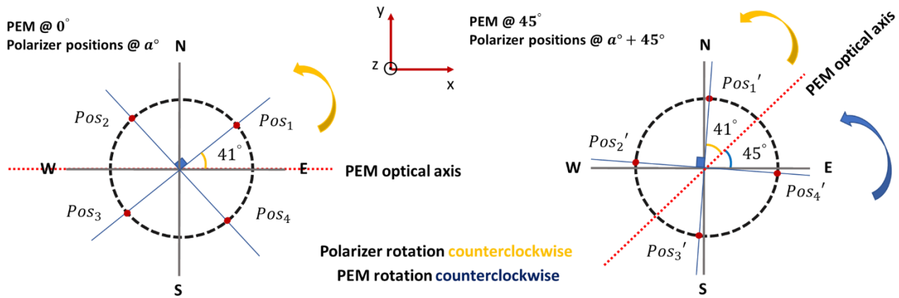
725 Figure 2: SolPol assembly positioning as seen from the incoming sunlight reference frame. Left arrangement: The initial sequence begins with the PEM and linear polarizer at the rest position of 0^\circ , then the polarizer rotates by 90^\circ starting from 41^\circ ( Pos_1 ), to 131^\circ ( Pos_2 ), 221^\circ ( Pos_3 ) and 311^\circ ( Pos_4 ) counter-clockwise. A complete polarizer rotation with the PEM at 0^\circ provides measurements of the U Stokes parameter. Right arrangement: assembly rotation by 45^\circ and subsequent similar rotation of the polarizer by 90^\circ intervals from Pos_1' to Pos_4' . This configuration provides measurements of the Q Stokes parameter.
