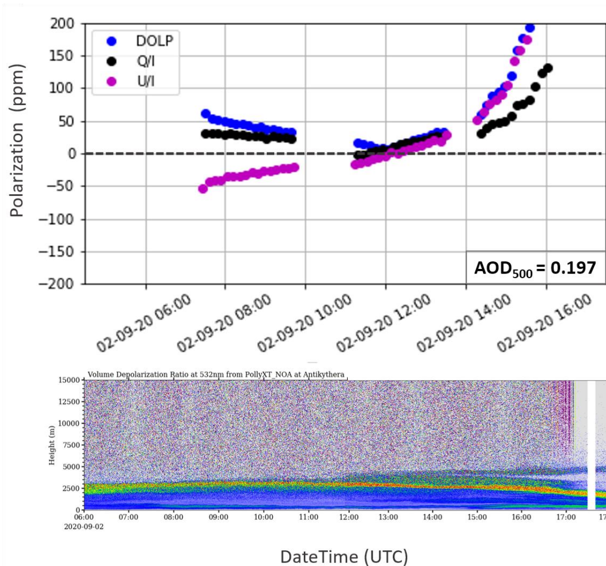
770 Figure 6: Top panel: Daily progression of linear polarization (in ppm) for the measurements on 02/09//2020, at the PANGEA observatory in Antikythera, expressed through the normalized Q/I (black dots), U/I (purple dots) Stokes parameters and DOLP (blue dots). The increase in linear polarization is exhibited before 08:00 and after 14:00 UTC when the instrument viewing angle increases significantly with respect to the zenith. Bottom panel: Time-height plot of the Volume Linear Depolarization Ratio ( \delta_v ) at 532 nm, as retrieved from the Polly XT lidar at PANGEA for the same day. High \delta_v values (>15%) are indicative of dust particle presence and larger concentrations of dust are denoted with dark orange hues.
