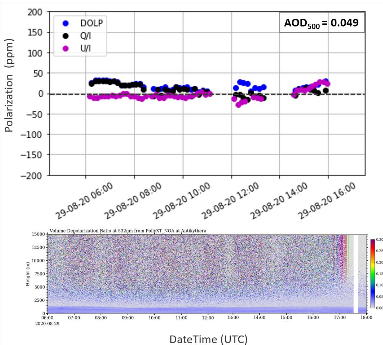
760 Figure 5: Top panel: Daily progression of linear polarization (in ppm) for the measurements on 29/08/2020, at the PANGEA observatory in Antikythera, expressed through the normalized Q/I (black dots), and U/I (purple dots) Stokes parameters and DOLP (blue dots). All values do not exceed the 50 ppm threshold regardless of the instrument viewing angle. Bottom panel: Time-height plot of the Volume Linear Depolarization Ratio ( \delta_v ) at 532 nm with the altitude, as retrieved from the Polly XT lidar at PANGEA for the same day. Low \delta_v values denote that there is low concentration of depolarizing particles for the total duration of the SolPol measurement.
