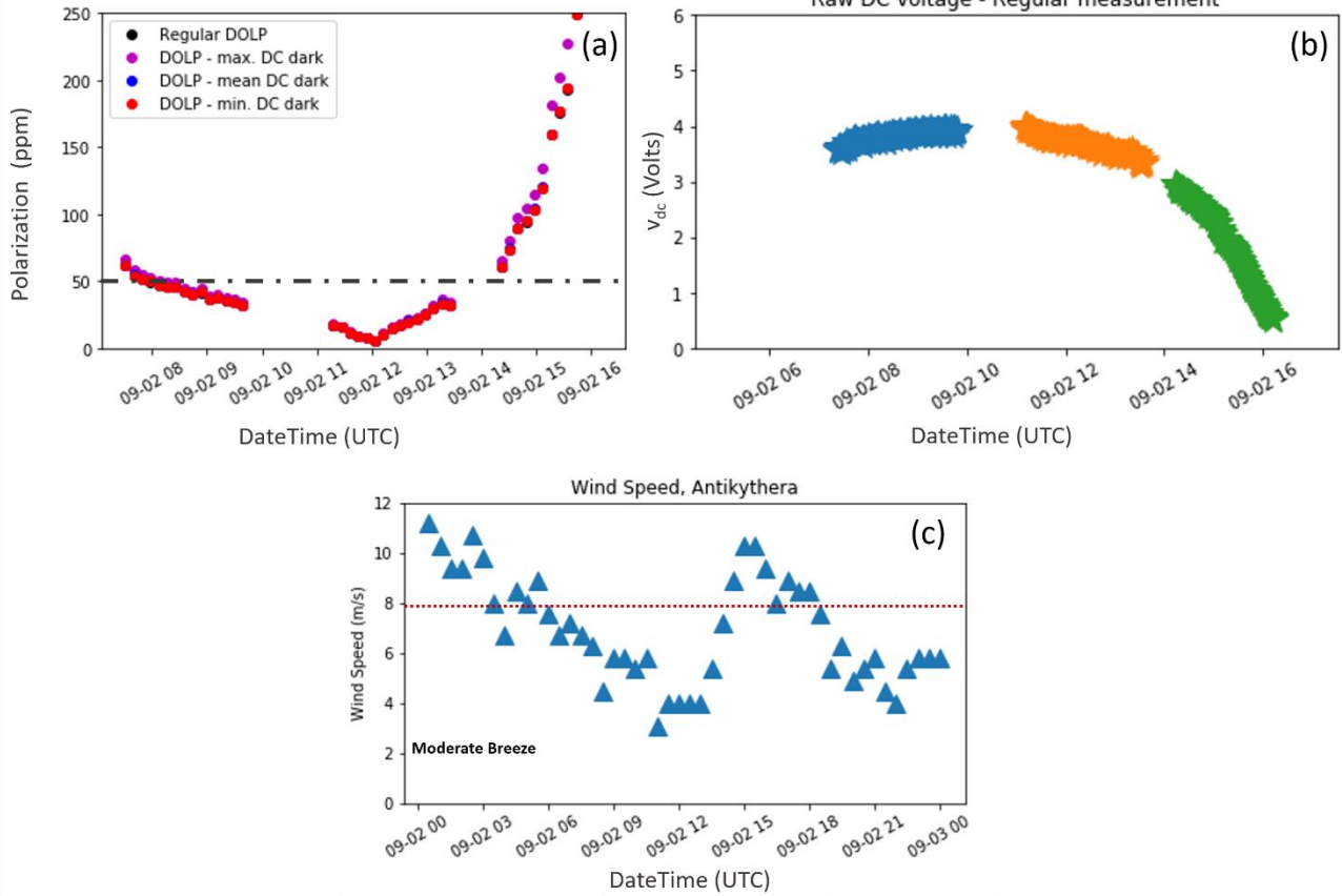
815 Figure A2: SolPol daily measurement on 02/09/2020, spanning from 07:00 to 16:00 UTC at the PANGAEA observatory, Antikythera. The specific day is affected by a persistent dust outbreak above the station, has zero percent cloud-cover and consists of a typical dust-driven measurement for the instrument. In panels: (a) the DOLP is plotted in parts per million in polarization for four test cases: calculated without subtracting the dark DC voltage for the specific day (black dots), by subtracting the maximum value (purple dots), average (blue dots) and minimum (red dots) values of the dark DC voltage output. The dash-dotted grey line signifies the instrument noise level at 50 ppm, (b) the total incoming sunlight intensity, v_{dc} in Volts as recorded by the lock-in amplifier. Different colours signify the corresponding measurement subsets within the day. (c) The recorded wind speed in m/s for 30-minute averages for the specific day. During the SolPol measurement moderate winds were blowing over the station. 820
