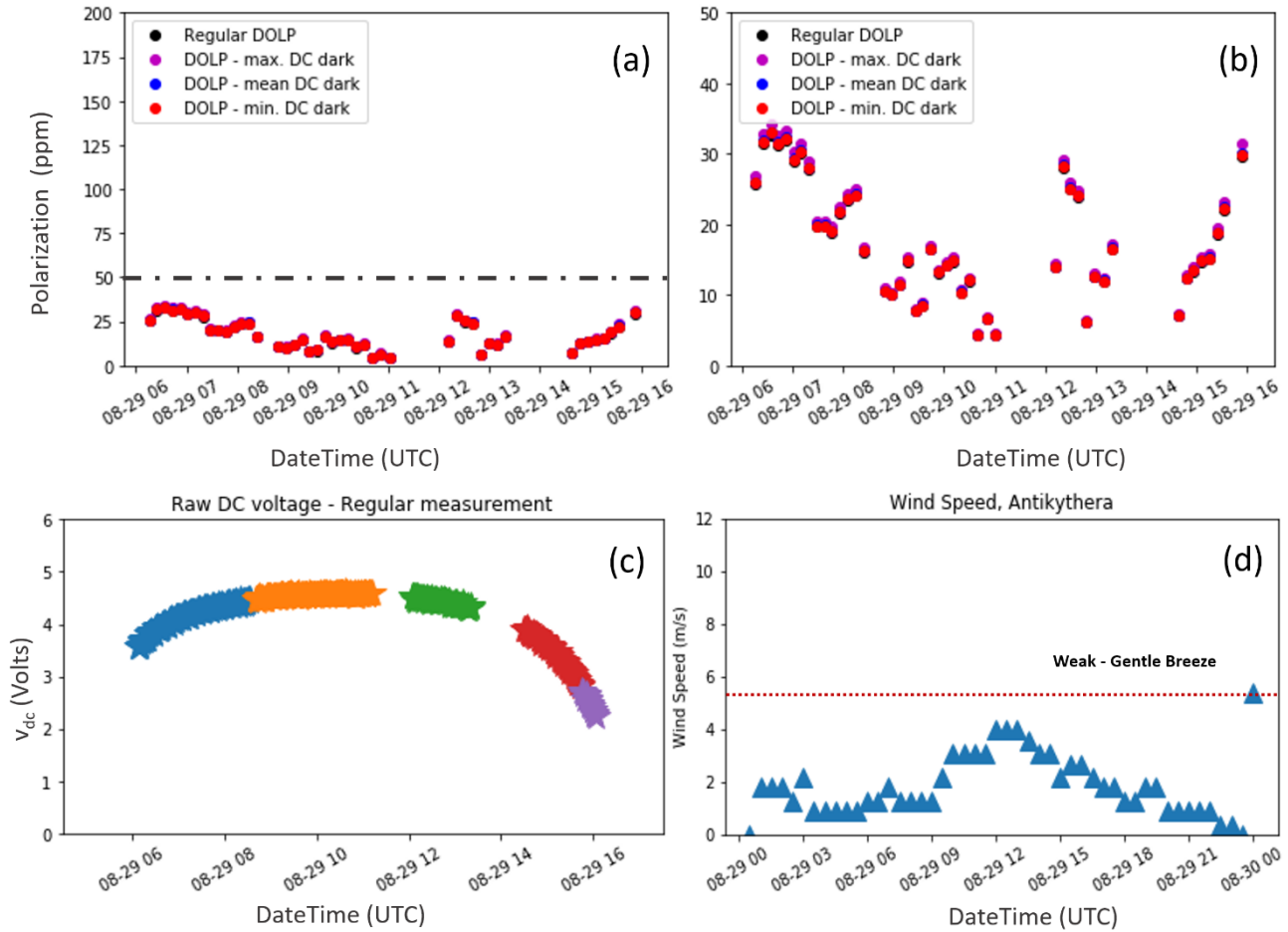
740 Figure 3: SolPol measurement on August 29 th 2020, spanning from 06:00 to 16:00 UTC at the PANGEA observatory, Antikythera. The day is labelled as “clean day” due to the very low aerosol content; zero percent cloud-cover and the acquired measurements consist a “background reference measurement” for the instrument. In panels: (a) the Degree of Linear Polarization (DOLP) plotted in parts per million (ppm) for four different test cases: calculated without subtracting the dark DC voltage for the specific day (black dots), by subtracting the maximum value (purple dots), average (blue dots) and minimum (red dots) values of the dark DC voltage output. The dash-dotted grey line signifies the instrument noise level at 50 ppm, (b) a zoomed representation of (a), (c) the total 745 incoming sunlight intensity, v_{dc} in Volts as recorded by the lock-in amplifier. Different colours signify the corresponding measurement subsets within the day and (d) the recorded wind speed in m/s for 30-minute averages on the specific day. During the SolPol measurements generally low-winds were blowing over the station.
