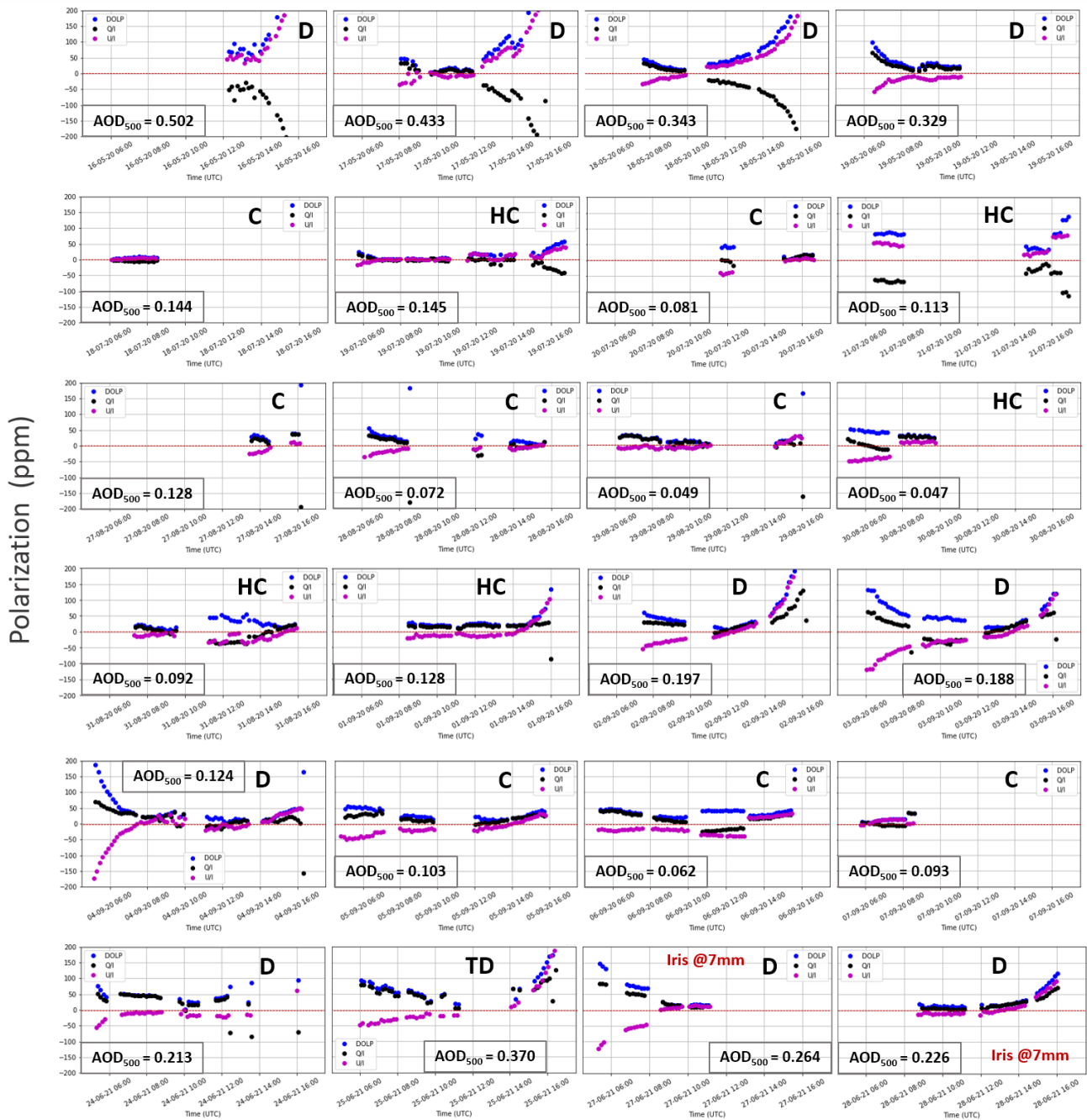
750 Figure 4: Complete SolPol linear polarization measurements acquired between May 2020 to June 2021 at the PANGEA observatory, Antikythera. Each daily observation consists of the normalized Q/I (black dots), U/I (purple dots) and DOLP (blue dots) in ppm with time, while labels D: stands for dust driven days with various loads, C: for clean days with low aerosol content, HC: for half-clean days where dust outbreaks occurred at some point within the day, and TD: is a dedicated test day with alternating iris sizes. Mean AOD level 1.5 values are provided for each day by AERONET ( https://aeronet.gsfc.nasa.gov/ , last visited: 12/12/2022). DOLP values during clean (C) days determine the instrument noise level for the polarization measurements, while during dust events (D) the DOLP values peak early in the morning and in the afternoon, reaching polarization values of more than 200 ppms per case. 755
