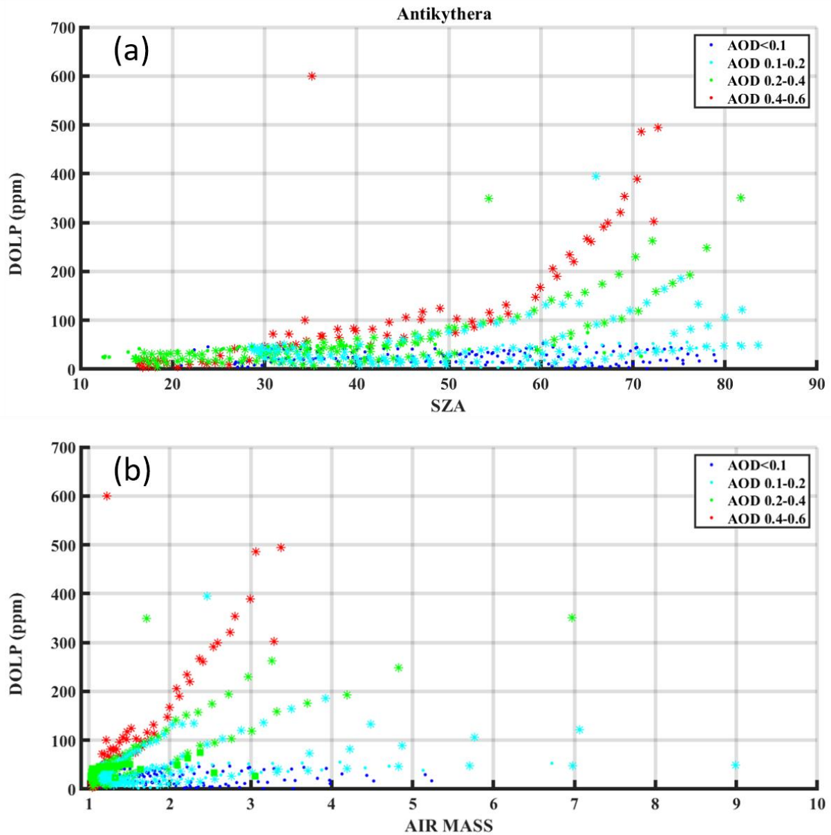
785 Figure 8: (a) DOLP as a function of the AOD with respect to the SZA, for the all the SolPol measurements in 2020 and 2021, at the 790 PANGEA observatory. Star markers denote dust days (D), circle markers denote clean days (C) and the colour scale refers to different AOD ranges. For small AOD values ( < 0.1 ), the linear polarization values are within the clean day threshold, while for AODs between 0.1-0.2, the DOLP values begin to exhibit the increasing trend with increasing SZAs, due to the potentially small concentration of preferentially oriented particles along the instrument line of sight. Significant linear polarization values are observed for all the dust days and the trend intensifies further for AODs towards the range between 0.4-0.6. (b) DOLP as a function of the airmass for the same AOD ranges. A linear correlation is observed between DOLP and the airmass for AOD values above 0.1, for the dust cases. For larger AODs, the DOLP values surpass the noise threshold for even smaller airmasses.
