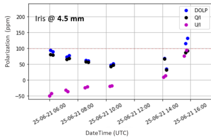
Figure 10: Alternating iris size tests for the quantification of diffuse light contribution to the linear polarization observations under the 25/06/2021 dust layer, with an AOD of 0.370 at 500 nm. Top panels present the normalized Q and U Stokes parameters, DOLP and the different colour arrows denote the respective iris size for each measurement set, along with the AOD progression within the day from AERONET.
