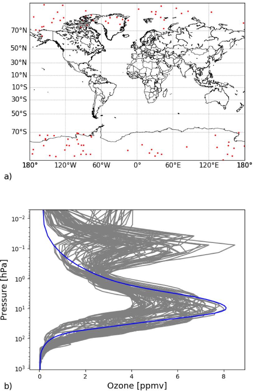
Figure 2. a) Spatial and b) vertical distribution of 87 ozone profiles from ozone subset which present double peak of ozone in the vertical distribution. These profiles have a second maximum of ozone quantity ( higher than 3 ppmv) above 0.9hPa. The mean ozone profile is represented by blue line.
