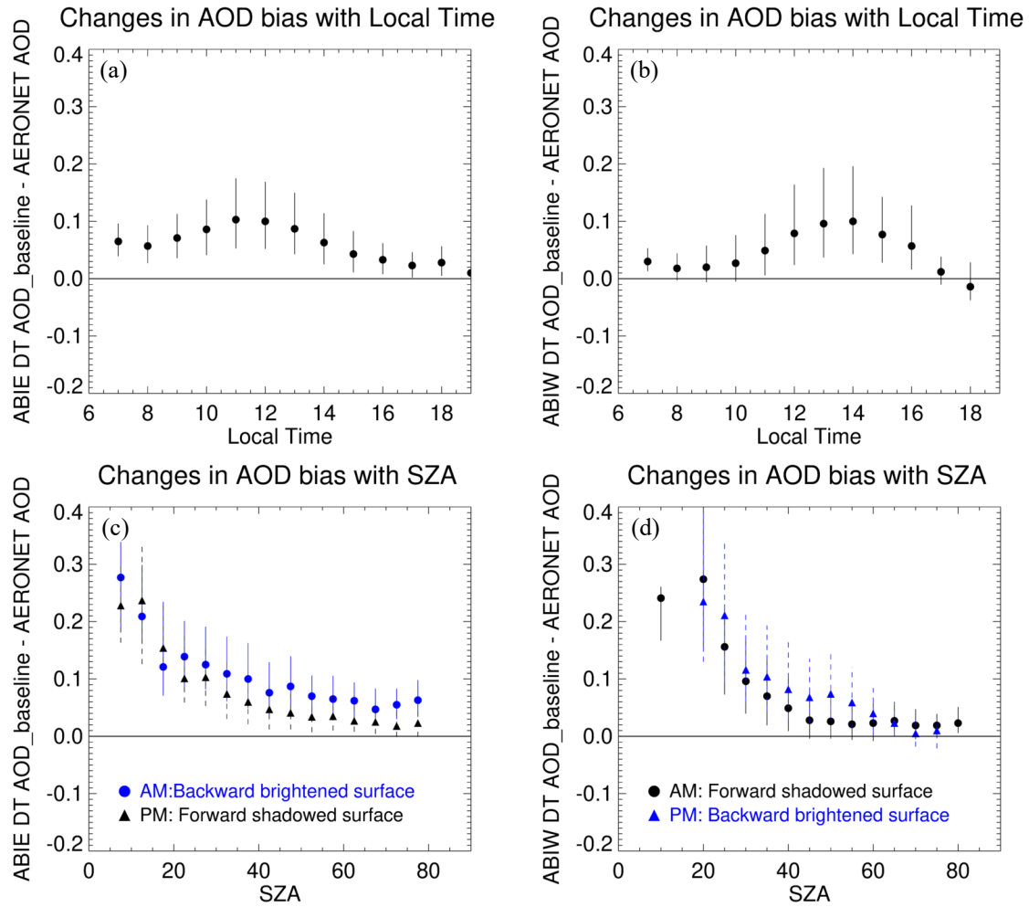
Figure 4 Bias of DT AOD compared to AERONET values. The DT AODs are retrieved from (a, c) GOES 16 ABI (ABIE) and (b, d) GEOS 17 ABI (ABIW) from August to September 2019. The biases are then calculated using data from all available AERONET site and aggregated for each (a, b) local solar time and (c, d) SZA. The symbol represents the median value and vertical bar displays the range between the 1st and the 3rd quartile of the AOD bias at each bin. In the bottom panels, the biases derived for morning and afternoon are differentiated by symbol [Circle: AM, Triangle: PM]. The blue represents backward scattering direction, while black indicates forward scattering direction.
