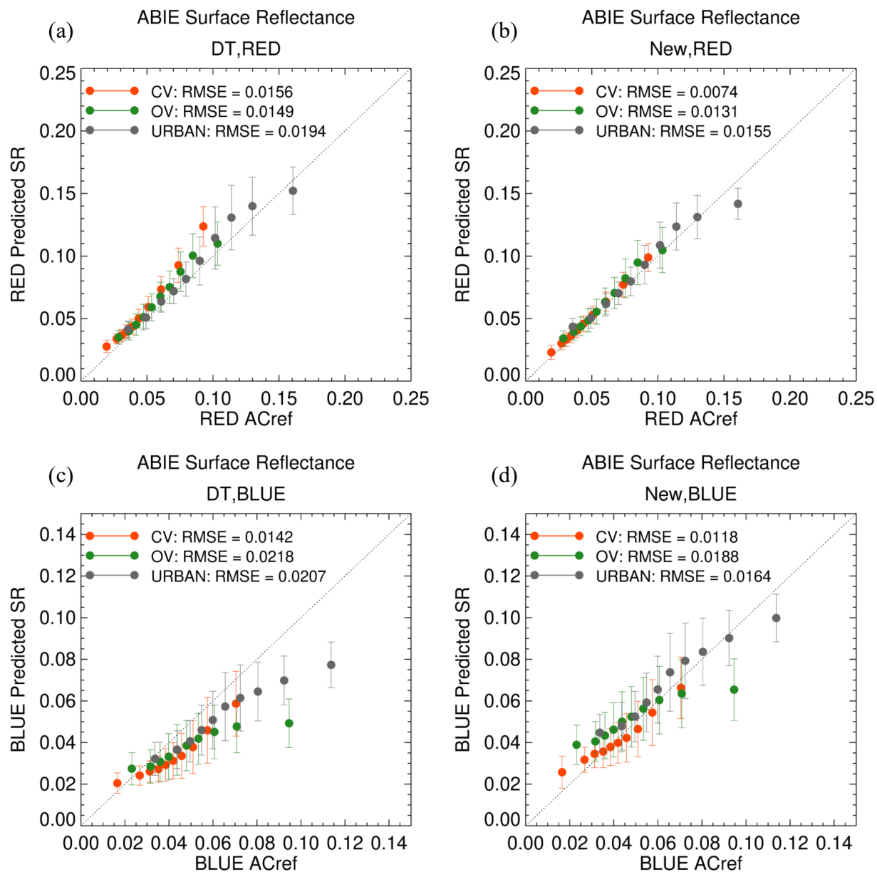
Figure 15 Comparisons between predicted surface reflectance and AC-ref for the (top) red and (bottom) blue channels. Left panels show the predicted surface reflectance achieved from the baseline DT SRP and the Right panels show the predicted surface reflectance using the new DT-Geo SRP. The predicted surface reflectance is sorted by AC-ref and equally divided into 10 bins. Symbol and vertical bar represent mean and standard deviation in each bin respectively, and color indicates land type: (red) CV, (green) OV, and (gray) Urban.
