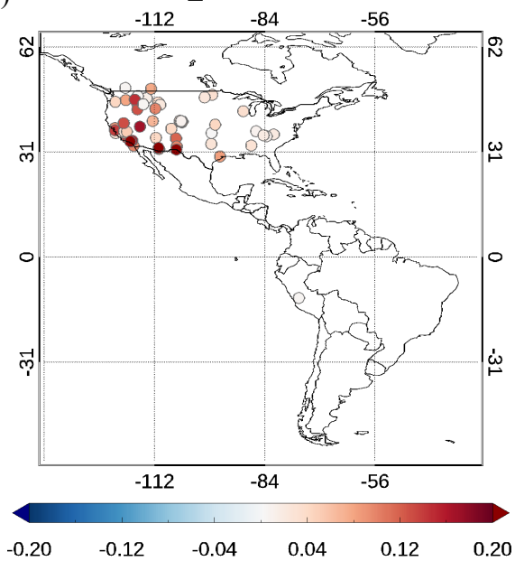
1005 Figure 18 Bias maps of (a, c) the baseline DT AOD and (b, d) the new DT AOD retrieved from (a, b) ABIE and (c, d) ABIW for August - September 2019. The bias represents the average of the absolute difference between DT AOD and AERONET AOD.
