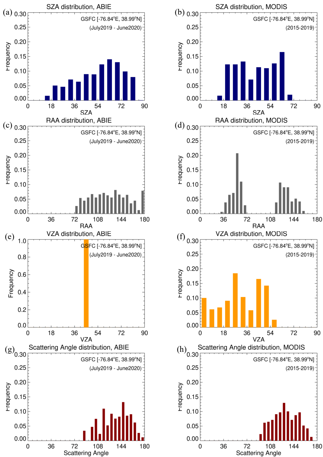
Figure 3 Frequency distributions of sun-and-sensor geometries for (left) ABIE and (right) MODIS measurements at GSFC AERONET site: (a, b) SZA, (c, d) RAA, (e, f) VZA, and (g, h) scattering angle.
