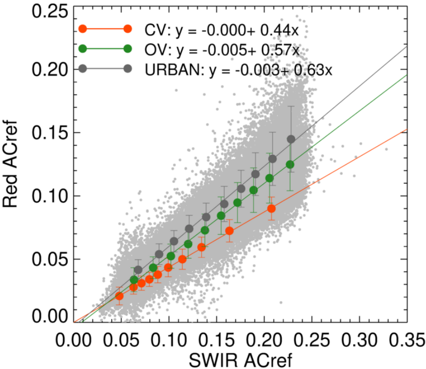
960 Figure 12 Linear regressions (a) between Red and SWIR AC-ref classified into three land cover types: Closed Vegetation (CV, Red), Open Vegetation (OV, Green) and Urban (Black). Each AC-ref group is divided equally into 10 bins and is displayed by mean (symbol) and standard deviation (vertical bar) of each bin. The gray dot represents a population of AC-ref, which is not distinguished by land type.
