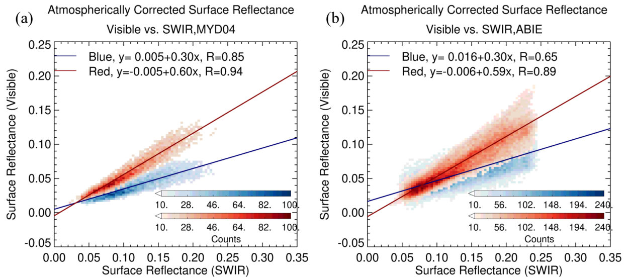
935 Figure 8 AC-ref in the visible (0.47 and 0.66 \mu\text{m} for MODIS and 0.47 and 0.63 \mu\text{m} for ABIE) compared with SWIR AC-ref (2.12 \mu\text{m} for MODIS and 2.24 \mu\text{m} for ABIE). The (a) MODIS AC-ref consists of 5 years of observations from 2015 to 2019 over the ABIE Field of View while the (b) ABIE AC-ref is for one year from July 2019 to June 2020. Blue and red indicate Red-SWIR and Blue-SWIR relationship, respectively.
