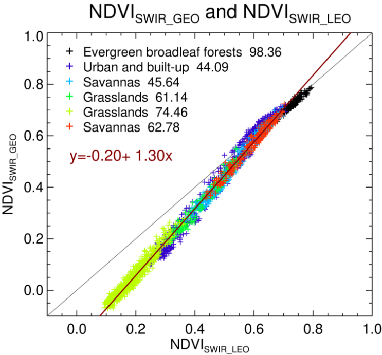
Figure A1 Comparison of NDVI GEO_SWIR and NDVI LEO_SWIR derived from MODIS (Aqua) TOA reflectance at six locations from Jan 2017 to June 2020. Color indicates the location. The names and numbers shown in the legend indicate the dominant land types and their occupancy at each location.
