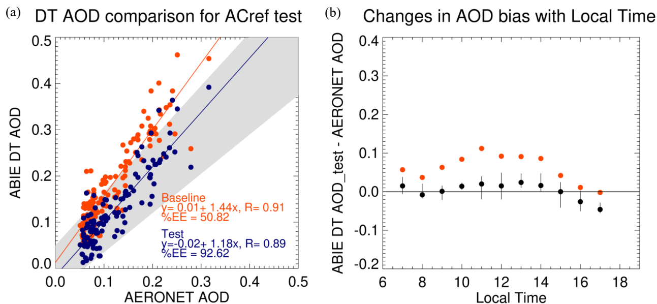
Figure 7 Validation of DT AOD retrieved from ABIE at GSFC in September 2019; (a) Scatter plots between ABIE AOD and AERONET AOD and (b) diurnal changes in the bias between them. Orange and black indicate different assumption in surface reflectance parameterization (SRP); Orange represents the DT AOD retrieved assuming the baseline DT SRPs but blue represents the tested AOD adopting the SRPs obtained from the AC-ref of ABIE (Fig. 6). The symbol indicates the median of the bias, and the vertical bars represent the first and the third quartiles.
