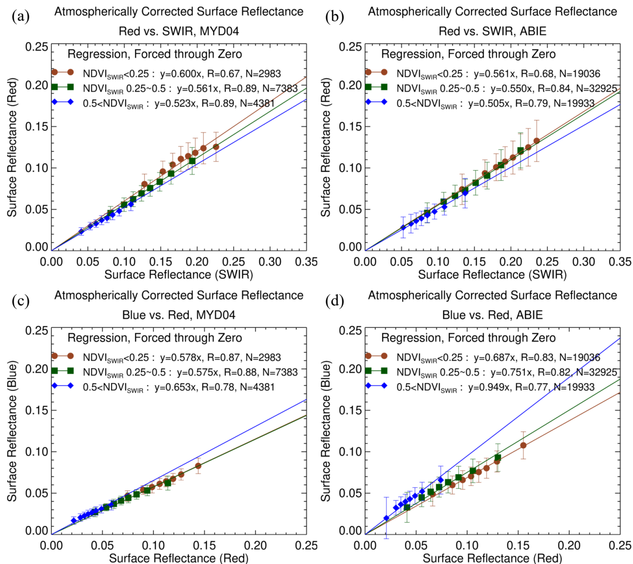
Figure 9 The AC-ref relationships (a, b) between red and SWIR and (c, d) between blue and red channel as a function of \text{NDVI}_{\text{SWIR}} . Left and Right columns indicate the relationships for MODIS and ABIE, respectively. The regression equation is forced through zero. Red refers to low \text{NDVI}_{\text{SWIR}} , green to medium and blue to high values. Each AC-ref group for \text{NDVI}_{\text{SWIR}} is divided equally into 8 bins and is displayed by mean (symbol) and standard deviation (vertical bar) of each bin.
