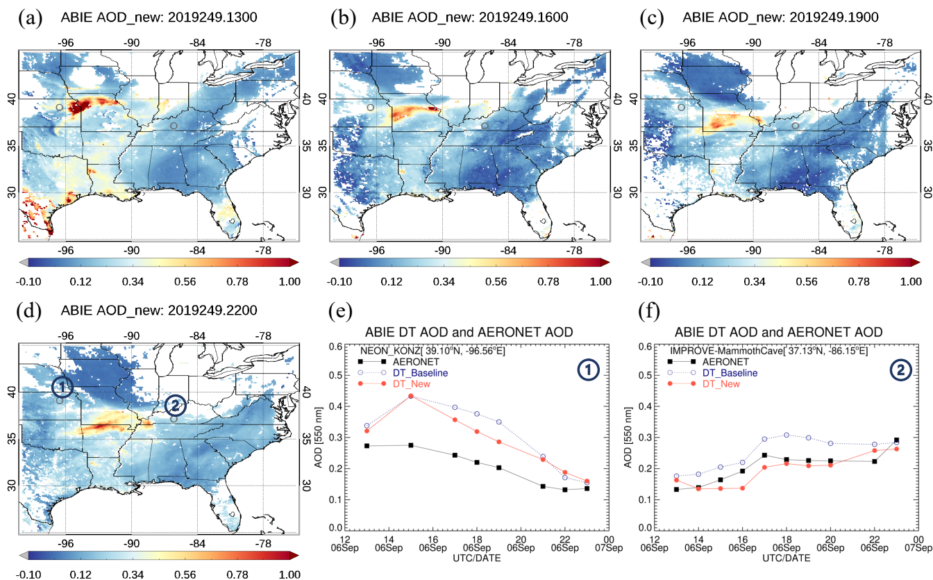
985 Figure 16 Three-hour interval map (a-d) displaying the new DT AOD retrieved from ABIE on September 6, 2019. A comparison is made between the new DT AOD and the baseline DT AOD as well as the AERONET AOD at two locations: (e) NEON_KONZ [39.10°N, -96.56°E] and (f) IMPROVE_MammothCave [37.13°N, -86.15°E]. A Black square indicates AERONET AOD [550 nm], a blue open circle represents the baseline DT AOD [550 nm], and a red closed circle denotes the new DT AOD [550 nm]. The AERONET sites are marked on the map with gray circle.
