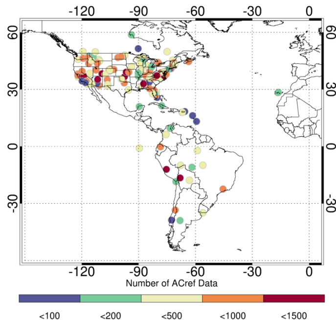
Figure 1 Map of AERONET which have available observation (AOD at 550 nm < 0.1, AE > 1.0) between July 2019 and June 2020, the time window for ABIE AC-ref calculation. The color represents number of valid observations which meet the criteria and applied to the AC_ref calculation.
