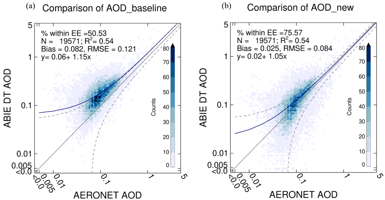
Figure 19 Comparison of the AEORNET AOD and the DT AOD retrieved from ABIE from August to September 2019 across all collocated AERONET stations within the sensors' disk scan. The DT AOD are retrieved by applying (a) the baseline and (b) the new SRP, respectively. The color indicates number density of scatter plot.
