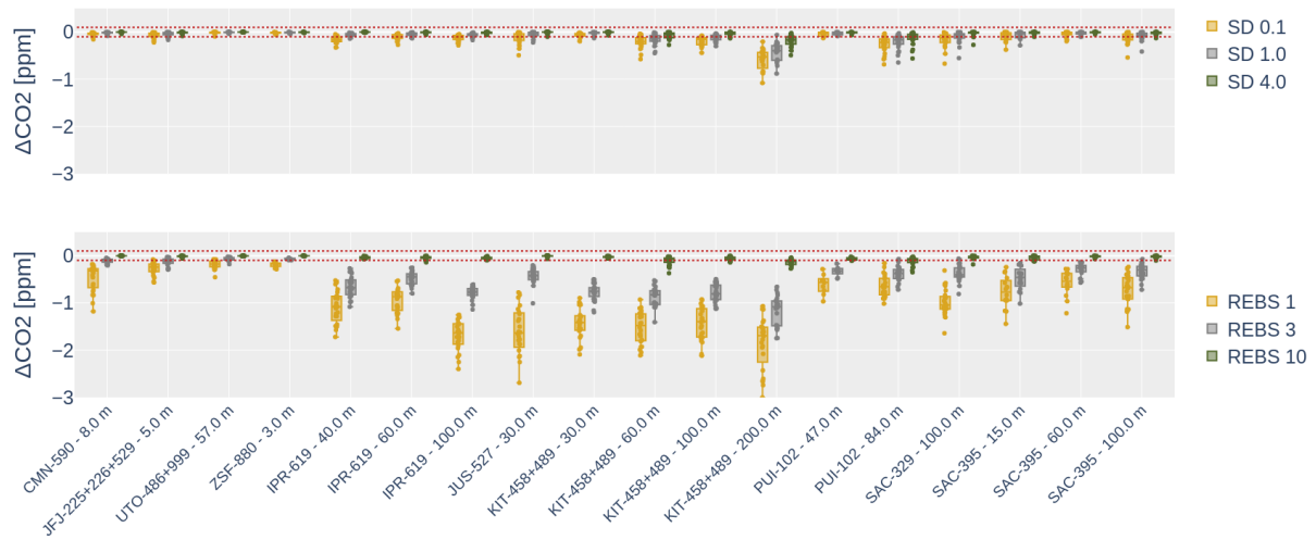
Figure 5: Boxplot differences ( \Delta\text{CO}_2 ) of the monthly mean \text{CO}_2 values between de-spiked and original dataset. The horizontal red lines represent the \pm 0.1 ppm WMO network compatibility goal. Each box represents the distribution of the differences for a combination of site and sampling height. The colour code indicates, for each algorithm, the adopted setting.
