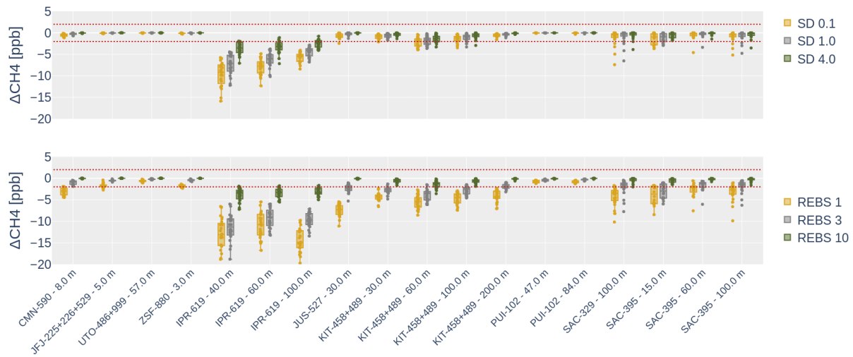
Figure 6: As Figure 4 but for CH 4 . The horizontal red lines represent the \pm 2 ppb WMO network compatibility goal.
