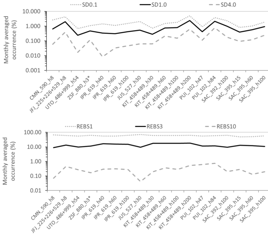
Figure 1: Percentages of the 1-minute CO 2 data selected as spike by SD (upper plot) and REBS (bottom plot) over the period 2018 - 2020 (for ZSF_880_h3, only 2021 was considered), for the different algorithm settings. For SD, \alpha was set to 0.1 (SD0.1), 1.0 (SD1.0) and 4.0 (SD4.0). For REBS, \beta was set to 1 (REBS1), 3 (REBS3) and 10 (REBS10). The codes reported as labels for the x-axis indicate the combination among site, instrument(s) ID and sampling height (m a.g.l.).
