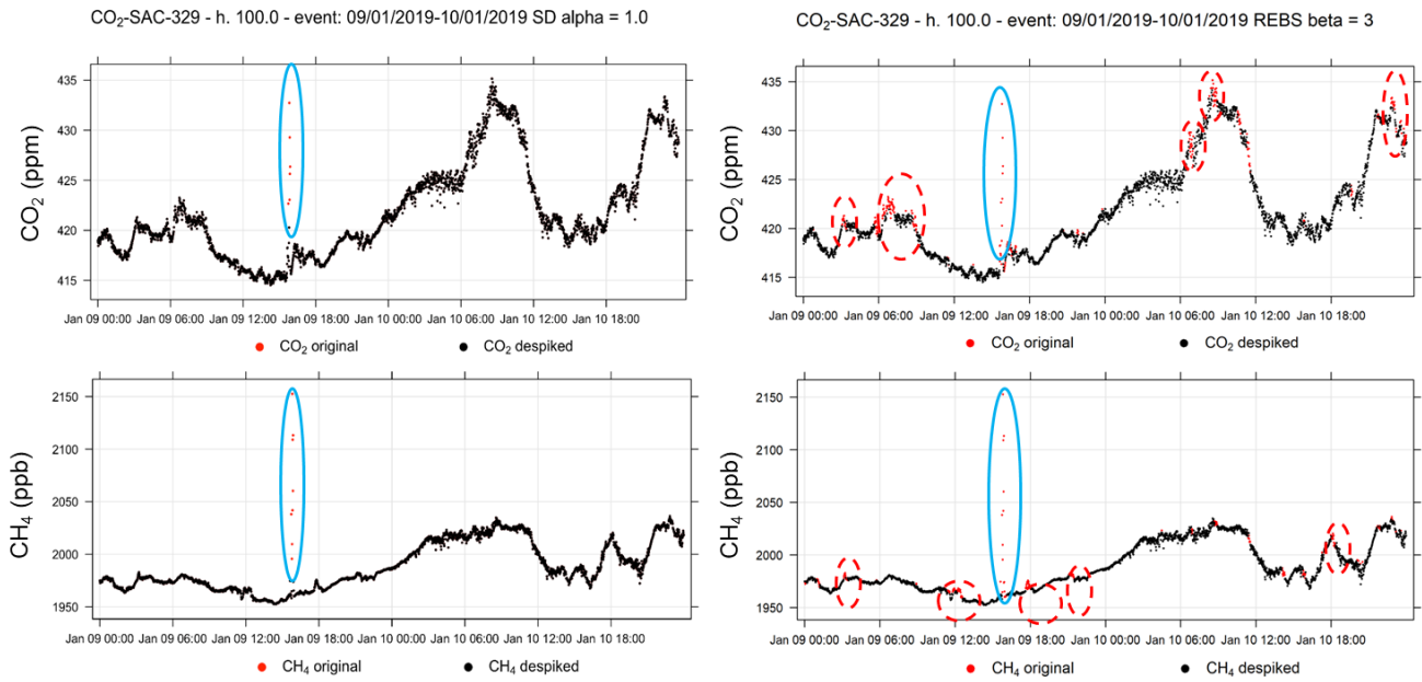
760 Figure 123: CO 2 and CH 4 observations at SAC (9-10 January 2019). No-spike data are reported by the black points (“despiked”); red points (“original”) denote the data flagged as spikes using SD (left) and REBS (right). Continuous (dotted) circles represent the spike attribution manually confirmed (not confirmed) by site PI.
