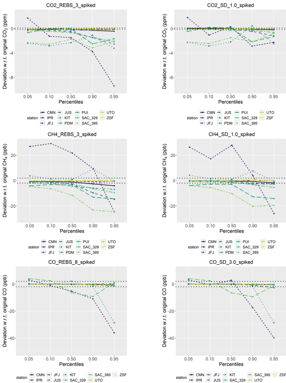
Figure 4: For the different sites (color code) the differences in the percentiles of hourly mean values between de-spiked and original dataset for the different species and methods are reported. The horizontal dotted lines represent the WMO network compatibility goal.
