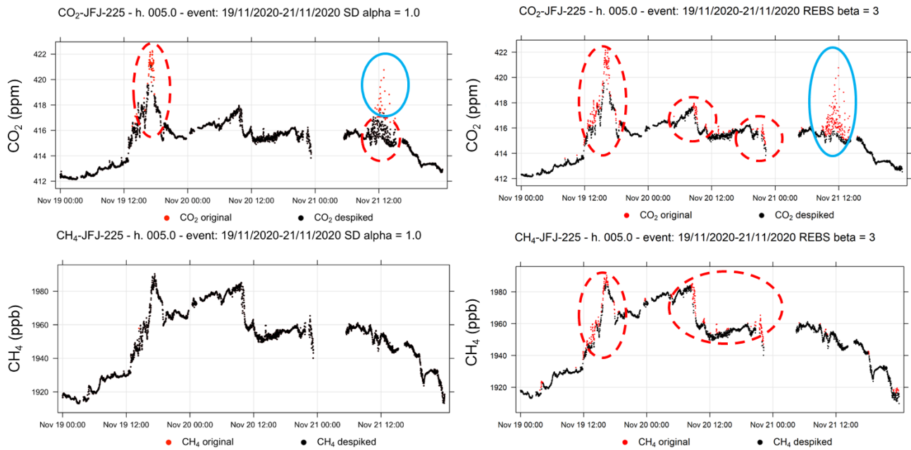
Figure 10 1 : CO 2 and CH 4 observations at JFJ (19-21 November 2020). No-spike data are reported by the black points (“despiked”); red points (“original”) denote the data flagged as spikes using SD (left) and REBS (right). Continuous (dotted) circles represent the spike attribution manually confirmed (not confirmed) by site PI.
