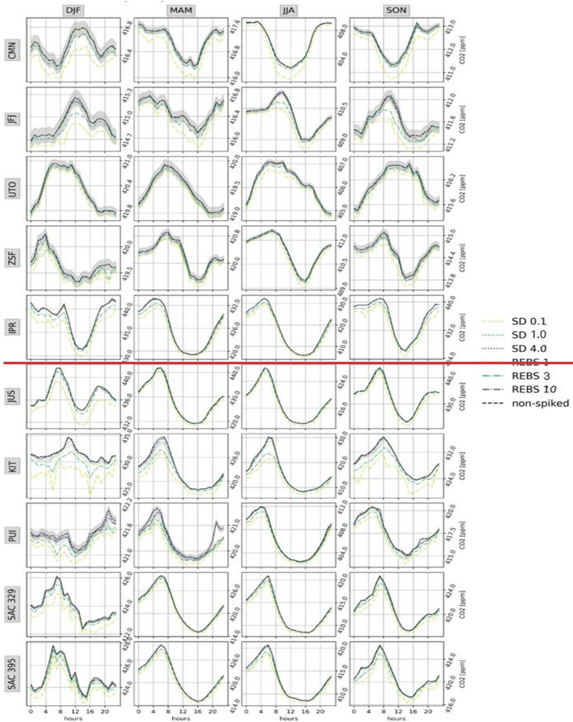
Figure 8: Mean seasonal diurnal cycles of CO 2 at selected sites and sampling heights for different data selection and sampling heights at ZSF, IPR and KIT: results for the original data are shown (“non-spiked”) together with those after de-spiking for SD
