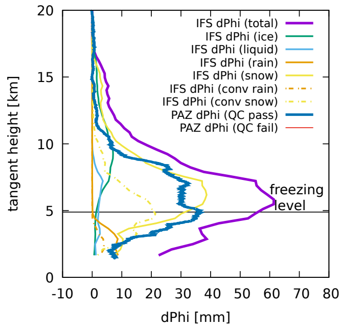
2019-10-30-MATMO-V06-fulldrift-0.125deg
