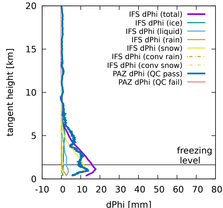
2021-01-09-AR-case-V06-fulldrift-0.125deg
