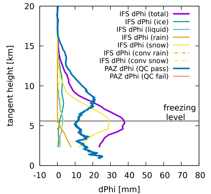
2021-10-12-KOMPASU-V06-fulldrift-0.125deg
