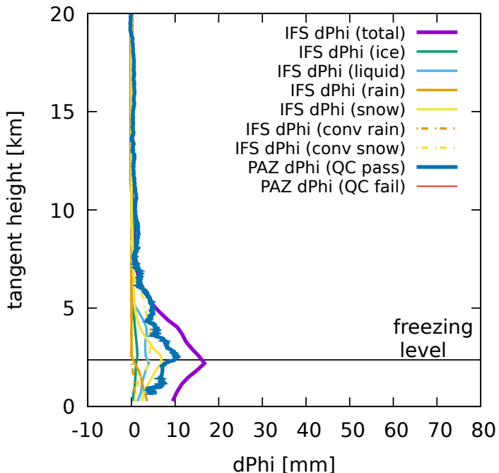
2021-01-10-AR-case-V06-fulldrift-0.125deg
