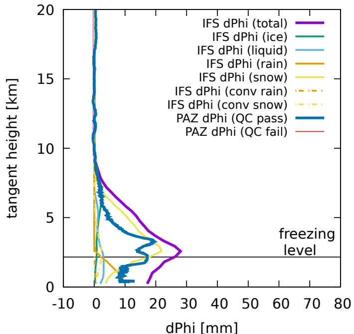
2021-01-14-AR-case-V06-fulldrift-0.125deg
