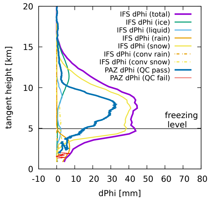
2021-09-06-LARRY-V06-fulldrift-0.125deg
