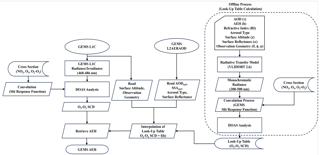
Figure 2. Flowchart of the AEH retrieval algorithm for GEMS satellite observation.
