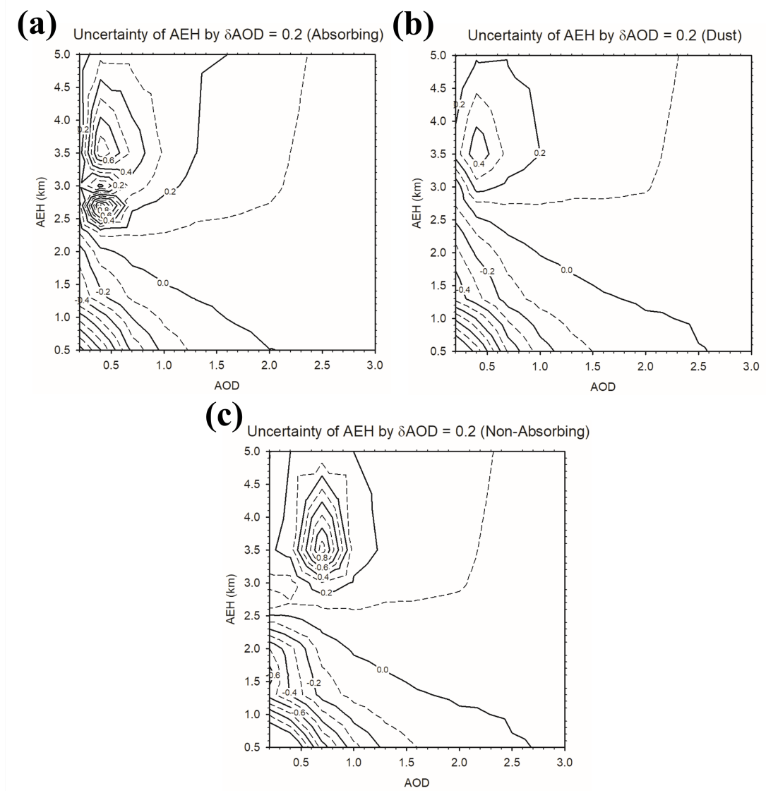
385 Figure 4. AEH retrieval uncertainty due to an the AOD error of 0.2 for cases with (a) 386 Absorbing, (b) Dust, and (c) Non-Absorbing aerosol types.
