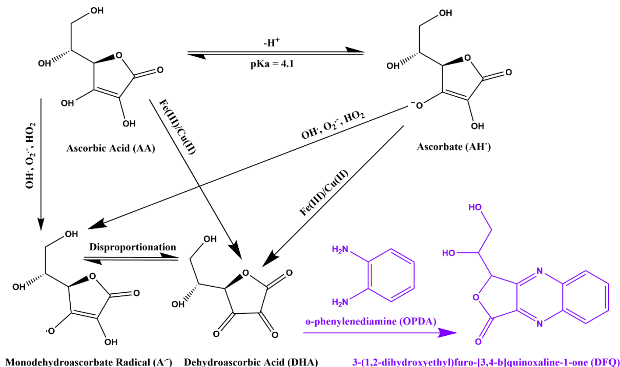
Figure 1 - Simplified reaction scheme describing AA and AH - oxidation by ROS and redox-active transition metals (black), and the condensation reaction with o -phenylenediamine (OPDA) to the fluorophore (1,2-dihydroxyethyl)-fluoro[3,4-b]quinoxaline-1-one (DFQ) (purple).
