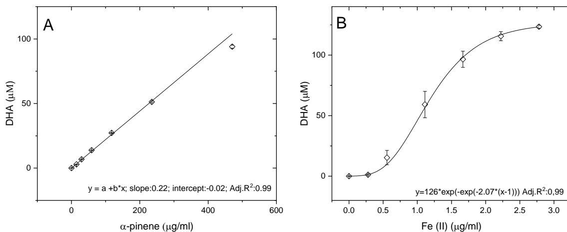
350 Figure 5: Response curves generated from (A) \alpha -pinene SOA from filter extracts and (B) from Fe(II)SO 4 solutions. The error bars represent the standard deviation of the spectrometer signal normalized to the DHA concentration during the 30 min measurement. The slope of the linear fits through the data and, therefore, the sensitivity is around 100 times higher for the iron sulphate than for SOA.
