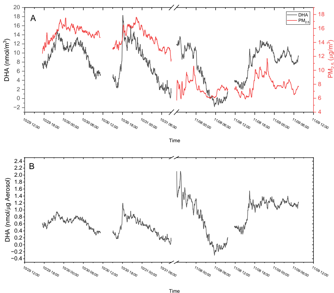
430 Figure 8 Ambient OOPAAI measurements in Basel (Switzerland) at Klingelbergstrasse 27, an urban background location in October and November 2022. (A) On the left x-axis, DHA in nanomole normalized to air volume and on the right x-axis PM 2.5 mass over time is plotted versus time. (B) DHA concentrations normalized to the mass of PM 2.5 at
