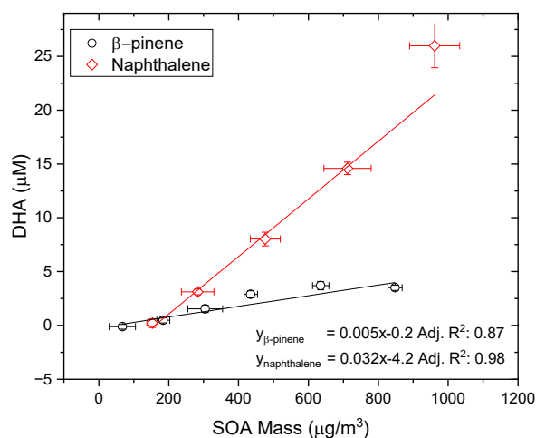
375 Figure 7 SOA was produced from an anthropogenic and biogenic precursor, respectively, at different mass concentrations using an organic coating unit (OCU, (Keller et al., 2022)). The OOPAAI signal shows a linear response for both SOA types as a function of particle mass with the anthropogenic SOA being much more reactive towards the
