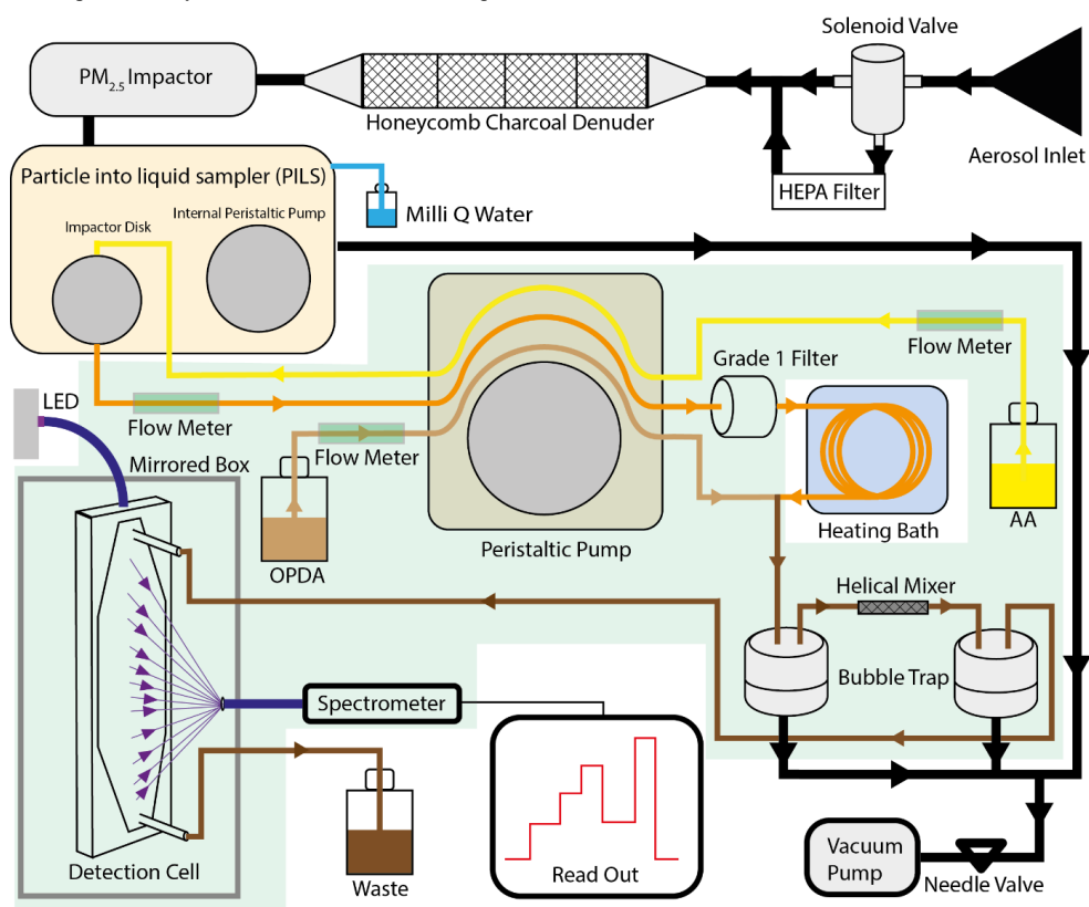
260 Figure 2 - Schematic overview of the OOPAAL. Black lines illustrate air flows where air gets pulled into the PILS via a denuder and an impactor. In the PILS the aerosol is collected with a wash flow containing ascorbic acid (yellow line) and pumped into a heating bath via a grade 1 filter (orange line). OPDA (light brown line) is then added, and the condensation reaction of DHA with OPDA to DFQ takes place (dark brown line). After a mixing piece and two bubble traps, the liquid is pumped into the detection cell, where DFQ is excited by an LED and the fluorescent emission is quantified by a spectrometer. All components are mounted in an aluminum and the components with a light green background are in the thermos-controlled compartment of the OOPAAL.
