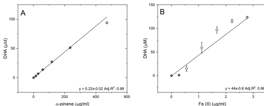
335 Figure 5: Response curves generated from (A) \alpha -pinene SOA from filter extracts and (B) from Fe(II)SO 4 solutions. The error bars represent the standard deviation of the spectrometer signal normalized to the DHA concentration during the 30 min measurement. The slope of the linear fits through the data and, therefore, the sensitivity is around 100 times higher for the iron sulphate than for SOA.
