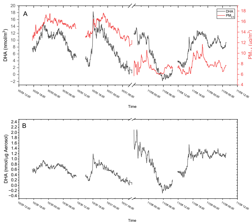
415 Figure 8 Ambient OOPAAI measurements in Basel (Switzerland) at Klingelbergstrasse 27, an urban background location in October and November 2022. (A) On the left x-axis, DHA in nanomole normalized to air volume and on the right x-axis \text{PM}_{2.5} mass over time is plotted versus time. (B) DHA concentrations normalized to the mass of \text{PM}_{2.5} at the same time. Gaps in the data are due to changing solutions in the OOPAAI or blank measurements. The LOD for ambient measurements is approximately 5 \mu\text{g}/\text{m}^3 .
