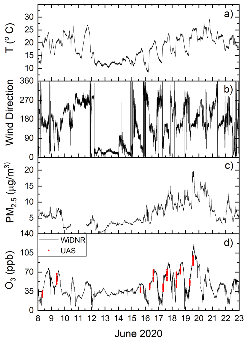
295 | Figure 23: June 8-22, 2020 a) temperature in °C b) wind direction, c) PM_{2.5} in \mu g/m^3 and d) O_3 as measured at the WIDNR ground station (black) and on the UAS via POM (red).
