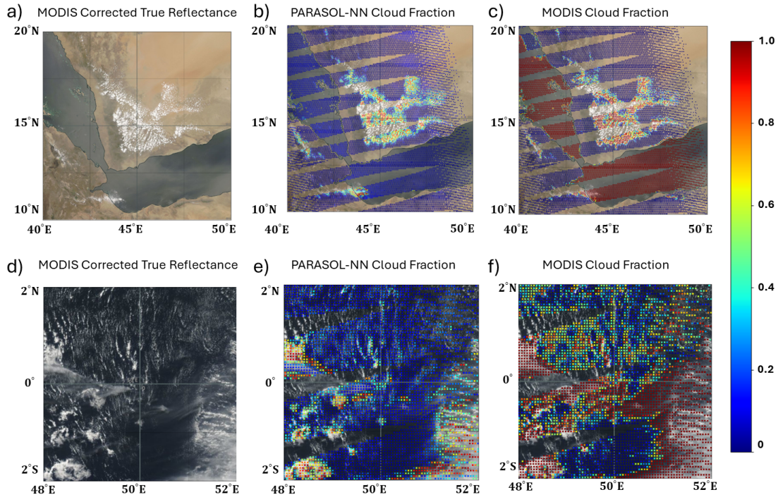
Figure 6. Cloud fraction around the Red Sea ( the upper row panel a-c ) and to the south of Somalia ( the lower row panel d-f ) on 1 July 2008. The left column ( panel a and d ) is the MODIS corrected true reflectance from the NASA worldview website . The middle column ( panel b and e ) shows the NN cloud fraction and the right column ( panel c and f ) is MODIS cloud fraction.
