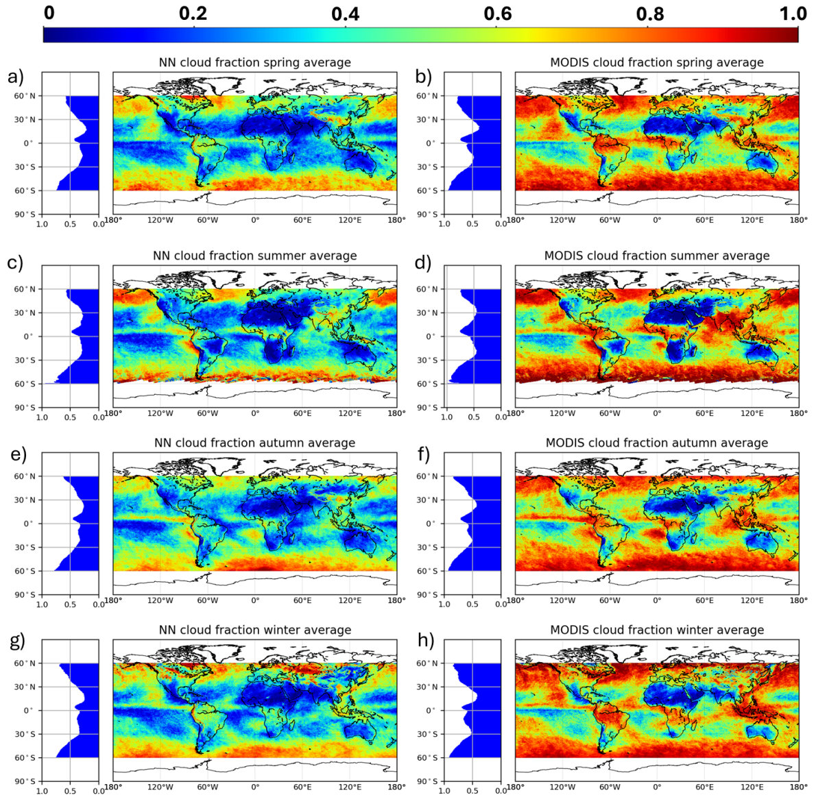
Figure 4. Seasonal cloud fraction average (on each \sim 6 \times 6 \text{ km}^2 PARASOL grid, shown in the colored world map. From the upper line to the lower line, winter (Dec-Feb) , spring (Mar-May, panel a and b) , summer (June-Aug) , panel c and d , autumn (Sep-Nov, panel e and f) , and winter (Dec-Feb, panel g and h) , and latitudinal distribution (cloud fraction average along each longitude as a function of latitude, shown in the histogram). The left subplot shows subplots (panel a, c, e, g) show the result from NN cloud fraction, and the right subplot subplots (panel b, d, f, h) is from MODIS cloud fraction.
