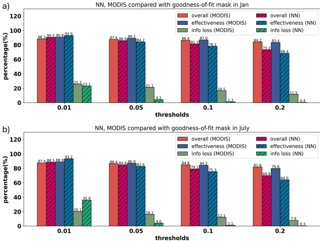
Figure 9. Comparison of the cloud masks with goodness-of-fit mask on 1 Jan 2008 and 1 July 2008. a) The upper-panel shows the comparison on 1 Jan, and the lower-panel is; b) The comparison on 1 July. The comparison between NN cloud mask and goodness-of-fit mask is shown in shaded bars, while the comparison between MODIS and goodness-of-fit mask is in unshaded bars. The red bars stand for overall agreement. The blue bars represent the effectiveness of masking out cloud, and the green bars are the information loss.
