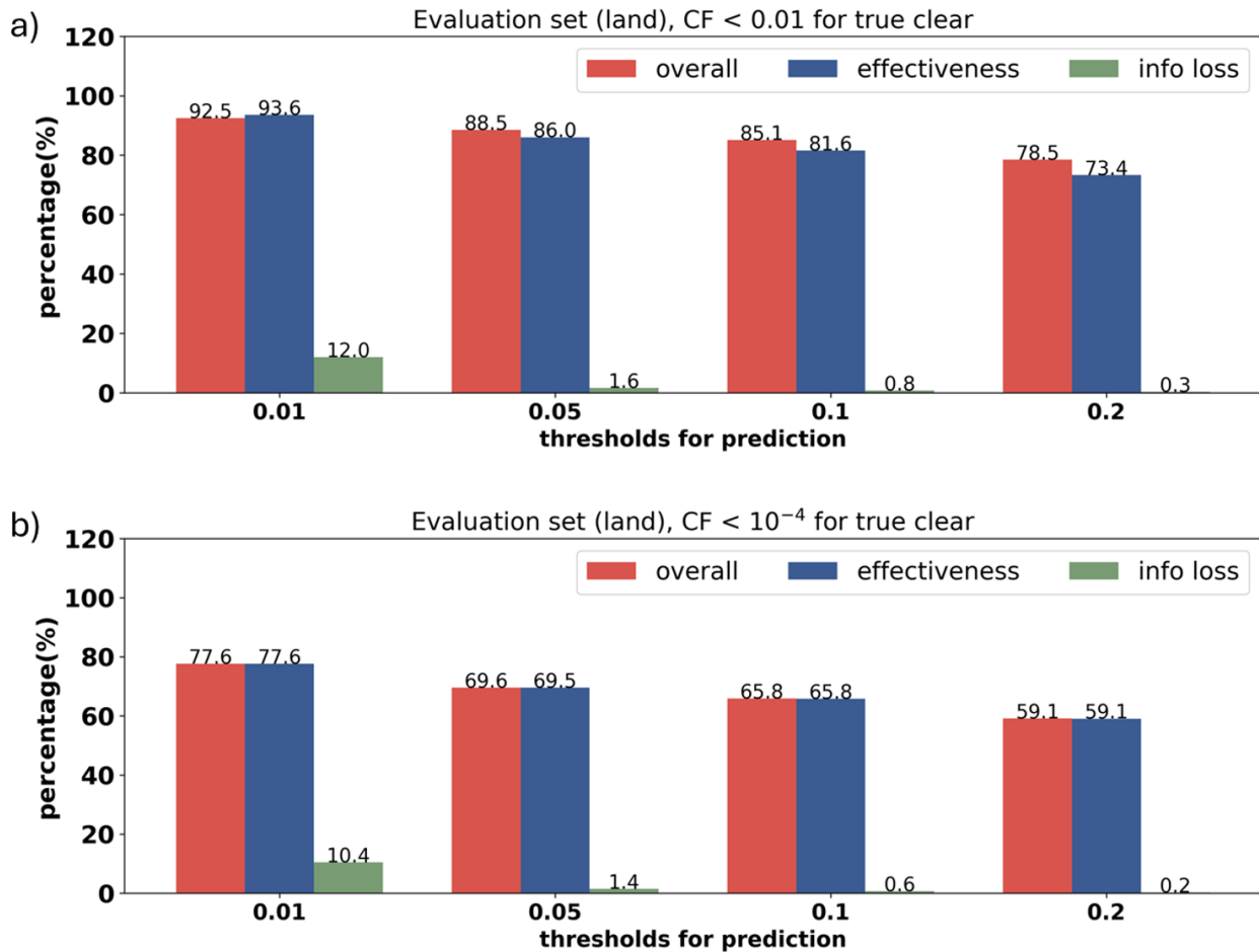
Figure 2. Performance of cloud mask over land on the synthetic test set for different thresholds. The upper panel uses a) "true" CF < 0.01 as truly clear while the lower panel uses b) CF < 10 -4 as truly clear. The red bar stands for overall agreement. The blue bar represents the effectiveness of masking out cloud, and the green bar is the information loss.
