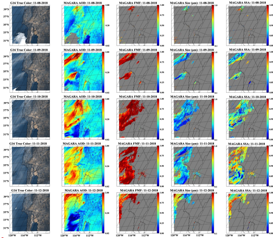
630 Figure 5) Context daily-averaged MAGARA retrievals over the Camp Fire region, Southwest United States, November 8 th -12 th , 2018. All panels, including the RGB images, are time-averaged for the entire day. Weights are also applied (0.0001 if not QA, 1 if 635 the retrieval passes QA) prior to the time averaging. Each row corresponds to a separate day (8 th for the top row and 12 th for the bottom row). The first column represents the weighted, temporally averaged RGB image for the entire day. The second column represents the weighted, temporally averaged 550 nm AOD. The third column represents the weighted, temporally averaged 550 nm fine-mode fraction. The fourth column represents the weighted, temporally averaged effective radius (in microns). The fifth column represents the weighted, temporally averaged 550 nm single-scattering albedo. AOD and particle property results are shown only if the temporal weight sum is > 1 for the day (at least 1 valid retrieval). Otherwise, they are masked as grey. Particle properties are only shown if AOD > 0.30, which represents the minimum we show for comparison to AERONET as well. Latitude labels are provided for the first column and longitude labels are provided for the last row.
