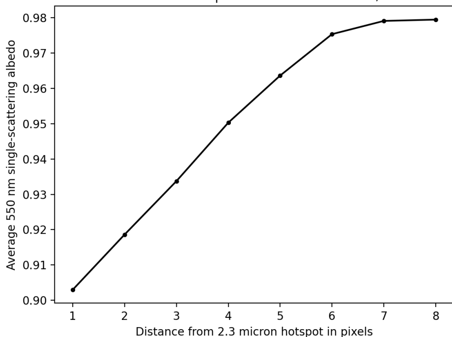
Figure 8) Comparison of average 550 nm single-scattering albedo (y-axis) vs distance from a 2.25 micron hotspot (x-axis) with a BRF > 0.99 for the Williams Flats Fire region, Pacific Northwest, August 3 rd -8 th , 2019. Averaging was done in AAOD and AOD space, prior to converting to single-scattering albedo, as this will minimize the impact of retrievals outside the smoke plume. In order to minimize the impact of clouds, only retrievals with cost < 20 were used in this analysis.
