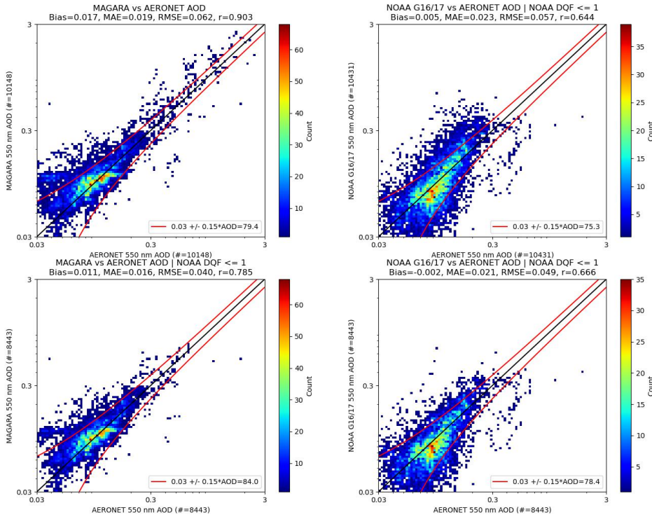
745 Figure 10) 2-D histograms of MAGARA and NOAA bias corrected 550 nm AOD retrievals vs AERONET 550 nm AOD. The upper left panel represents the MAGARA vs AERONET 550 nm AOD 2-D histogram with a 9 x 9 pixel spatial average. The upper right panel represents the NOAA GOES-16/17 bias corrected vs. AERONET 550 nm AOD 2-D histogram with a 9 x 9 pixel spatial average. The bottom rows represent the same as the top row, but with the requirement of at least 1 valid MAGARA and NOAA bias corrected pixel for each AERONET coincidence (apples-to-apples). A standard +/- (0.03 + 0.15 * AOD) uncertainty envelope is provided for reference, with the percent meeting that threshold indicated. Statistics for each panel are presented in the title.
