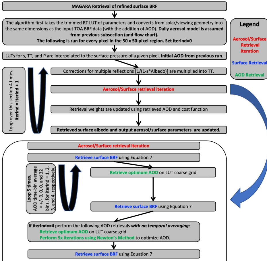
460 Figure 3) Flow chart of MAGARA refined surface BRF retrieval.
