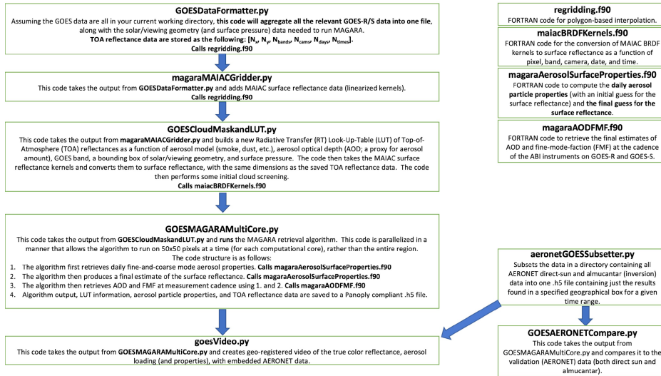
Figure 1) Algorithmic flow chart of MAGARA, from initial data formatting to video generation and validation. Four FORTRAN subroutines compiled and imported into the Python programming environment are shown in the upper right.
