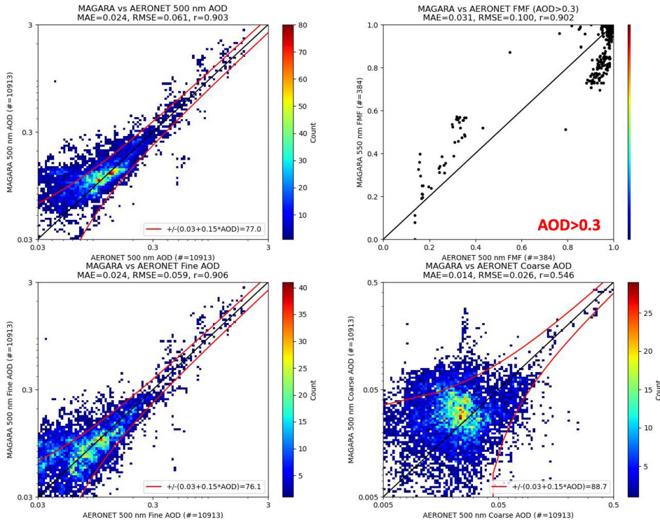
790 Figure 11) Over land comparison of MAGARA vs. AERONET AOD, fine-mode fraction, fine-mode AOD, and coarse-mode AOD. The upper-left panel represents a 2-D histograms of MAGARA vs AERONET 500 nm AOD. The upper-right panel is a scatterplot of MAGARA 550 nm fine-mode fraction vs AERONET 500 nm fine-mode fraction, for MAGARA retrieved 500 nm AOD > 0.3. The lower-left panel represents a 2-D histograms of MAGARA vs AERONET 500 nm fine-mode AOD. The lower-right panel represents a 2-D histograms of MAGARA vs AERONET 500 nm coarse-mode AOD. Statistics for each panel are presented in the title. For the comparisons of AOD, a standard \pm(0.03 + 0.15 \cdot \text{AOD}) uncertainty envelope is provided for reference, with the percent meeting that threshold indicated
