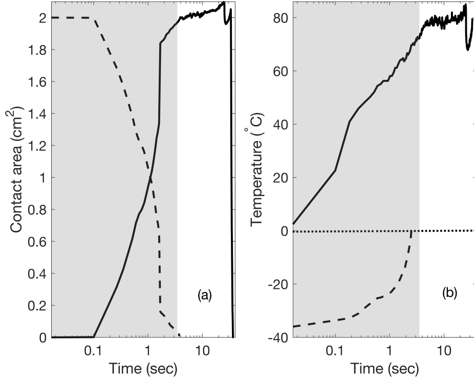
Figure 2. Observed melting and evaporation of a laboratory-made ice particle on the DEID hotplate. (a) Time series of the area of the ice particle, A_{ice}(t)
