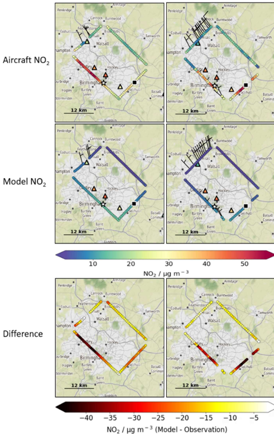
1210 Figure 17: Aircraft flight tracks coloured by NO 2 concentration (µg m -3 ) for the first (left, 11:23 to 11:43) and 1215 fourth (right, 12:33 to 12:52) circuit, at altitudes of 423 and 657 metres, respectively, around Birmingham during flight M296 on 1 st July 2021. Top row shows the aircraft data, middle row shows the model data and bottom row shows the difference between the model and observations. Observation data is from straight and wings level transects and all data is averaged over 10 second intervals. Wind barbs are only shown where the observed wind components exceed the measurement uncertainty. Data in triangles is the hourly surface level AURN NO 2 concentration for the circuit. Stars/squares show the location of the Birmingham supersite/airport, respectively Map tiles by Stamen Design, under CC BY 3.0. Data by OpenStreetMap, under ODbL.
