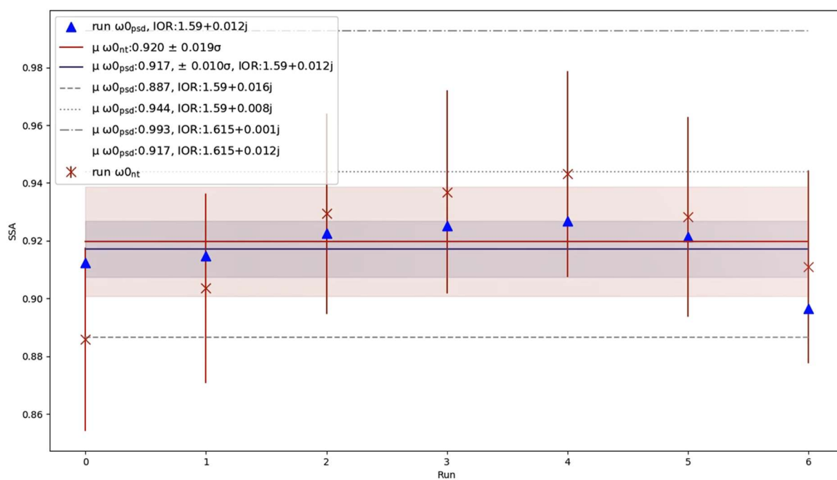
Figure B1: Empirically derived nephelometer and TAP single scattering albedo ( \omega_{nt} , red, crosses) and theoretically derived particle size distribution single scattering albedo ( \omega_{psd} , blue, triangles) for 7 straight and level runs for flight M270 on 15 th September 2021 north of Cambridge. Flight mean \omega_{nt} and \omega_{psd} with 1\sigma variance (solid lines and shaded areas in red and blue, respectively) are shown. Also shown are the mean \omega_{psd} derived using particle size distributions (PSD) corrected with the IOR which yielded \omega_{psd} that closely matches
