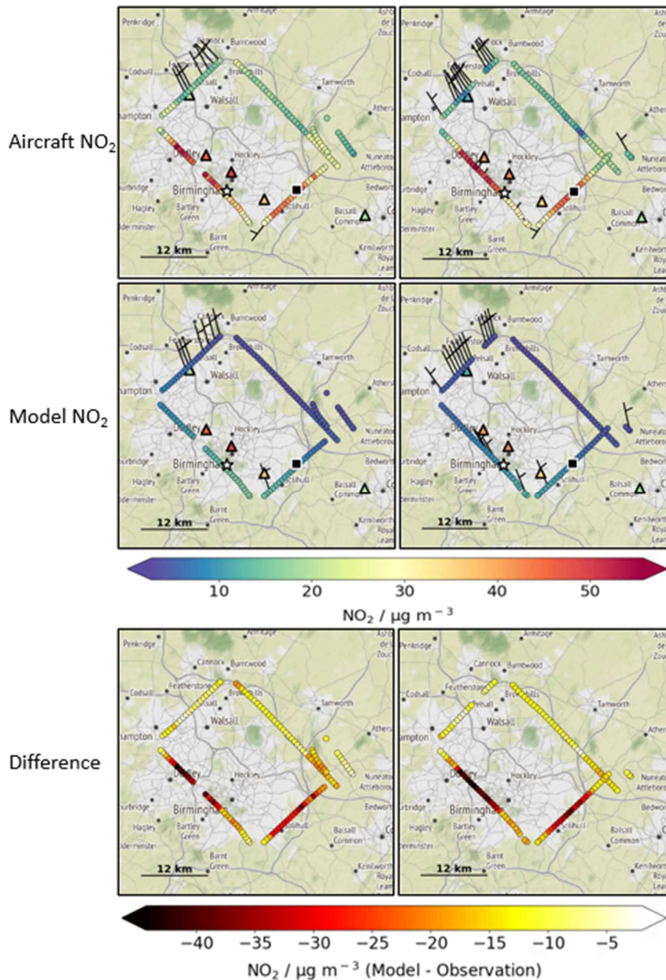
Figure D1: Aircraft flight tracks coloured by NO 2 concentration ( \mu\text{g m}^{-3} ) for the second (left, 11:43:00 to 12:10:00 and third (right, 12:10:00 to 12:33) circuit, at altitudes of 511 and 573 metres, respectively, around Birmingham during flight M296 on 1 st July 2021. Top row shows the aircraft data, middle row shows the model data and bottom row shows the difference between the model and observations. Observation data is from straight and wings level transects and all data is averaged over 10 second intervals. Wind barbs are only shown where the observed wind components exceed the measurement uncertainty. Data in triangles is the hourly surface level AURN NO 2 concentration for the circuit. Stars/squares show the location of the Birmingham supersite/airport, respectively. Map tiles by Stamen Design, under CC BY 3.0. Data by OpenStreetMap, under ODbL
