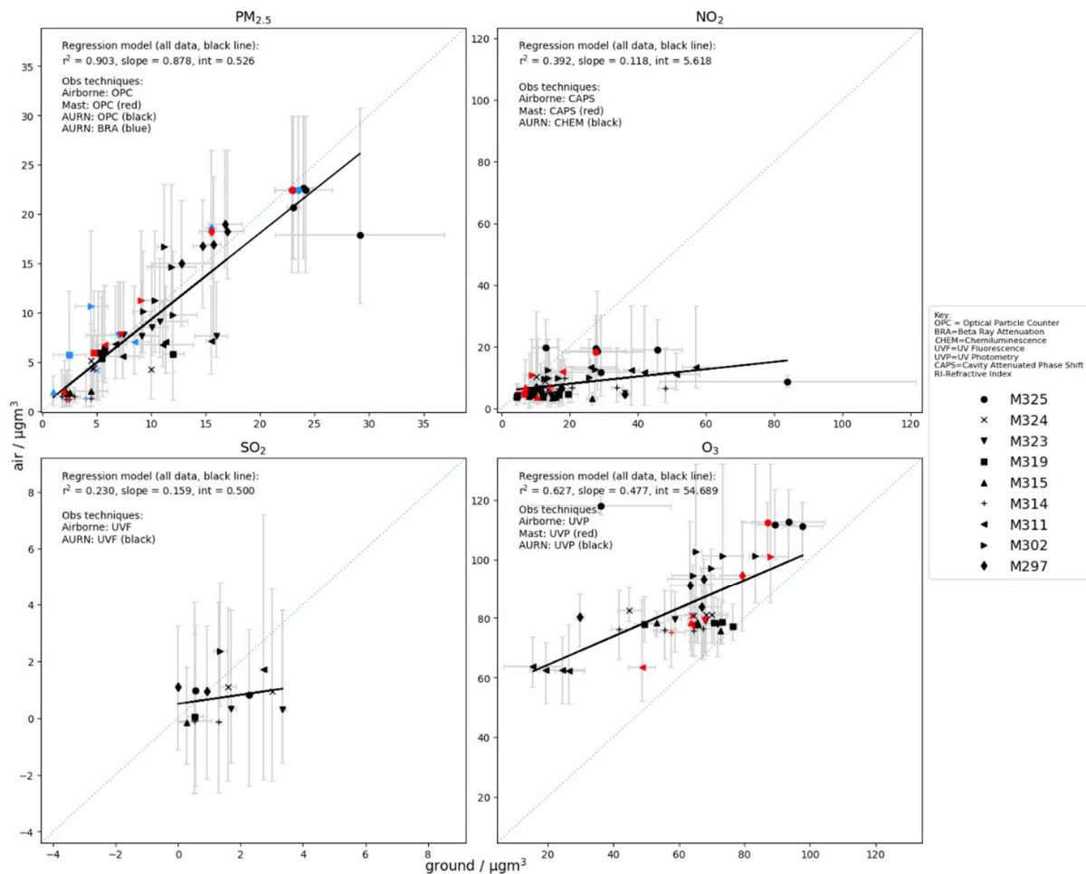
1180 Figure 12: Average airborne observations within a 12 km radius of ground site, against local ground site average, for PM 2.5 (top left), NO 2 (top right), SO 2 (bottom left) and O 3 (bottom right), for all available London IOP flights. Comparisons against OSCA mast data are shown in red and against AURN ground-sites in black. For PM 2.5 , blue markers identify those AURN sites that employ Beta Ray Attenuation technique (black employs an optical particle counter with conversion to mass technique). Linear regression between airborne and ground and mast-based data is shown in black. Error bars (grey) show the range of data and the 1-2-1 line, representative of a perfect linear relationship , is shown as a grey dotted line. 185
