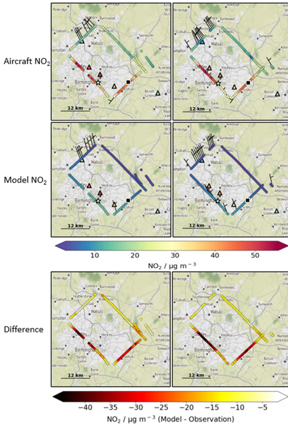
Figure D1: Aircraft flight tracks coloured by NO 2 concentration (µg m -3 ) for the second (left, 11:43:00 to 12:10:00 and third (right, 12:10:00 to 12:33) circuit, at altitudes of 511 and 573 metres, respectively, around Birmingham during flight M296 on 1 st July 2021. Top row shows the aircraft data, middle row shows the model data and bottom row shows the difference between the model and observations. Observation data is from straight and wings level transects and all data is averaged over 10 second intervals. Wind barbs are only shown where the observed wind components exceed the measurement uncertainty. Data in triangles is the hourly surface level AURN NO 2 concentration for the circuit. Stars/squares show the location of the Birmingham supersite/airport, respectively. Map tiles by Stamen Design, under CC BY 3.0. Data by OpenStreetMap, under ODbL
