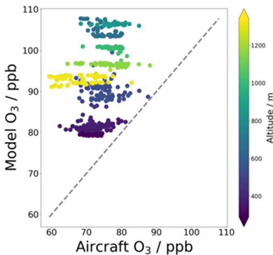
Figure 15: Correlation of model and aircraft O 3 concentrations. Data averaged over 10 second intervals. Markers coloured by altitude. Dashed grey line represents agreement between the two datasets. Data shown for (a) Flight M270 on 15 th September 2020, from 12:13:00 to 13:38:00 (the duration of the stacked level runs north of Cambridge) and (b) Flight M296 on 1 st July 2021 from 11:23:00 to 12:52:00 (the duration of the Birmingham city circuits).
