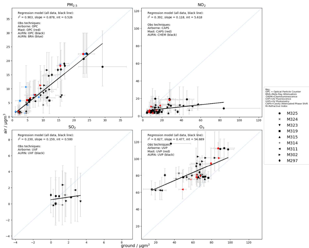
Figure 12: Average airborne observations within a 12 km radius of ground site, against local ground site average, for PM 2.5 (top left), NO 2 (top right), SO 2 (bottom left) and O 3 (bottom right), for all available London IOP flights. Comparisons against OSCA mast data are shown in red and against AURN ground-sites in black. For PM 2.5 , blue markers identify those AURN sites that employ Beta Ray Attenuation technique (black employs an optical particle counter with conversion to mass technique). Linear regression between airborne and ground and mast-based data is shown in black. Error bars (grey) show the range of data and the 1-2-1 line, representative of a perfect linear relationship, is shown as a grey dotted line.
