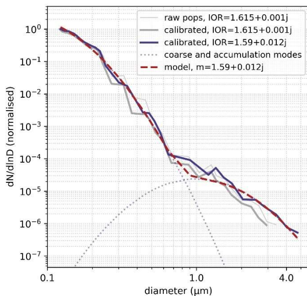
Figure 6: An example of raw, calibrated and calibrated with IOR-correction ( 1.59+0.012j ) particle size distributions, where the Y axis is normalised to 1. Overlaid are lognormal accumulation and coarse modes (dotted) plus the combination of these lognormal modes (dashed) fitted to the calibrated with IOR correction (blue solid line) size distribution.
