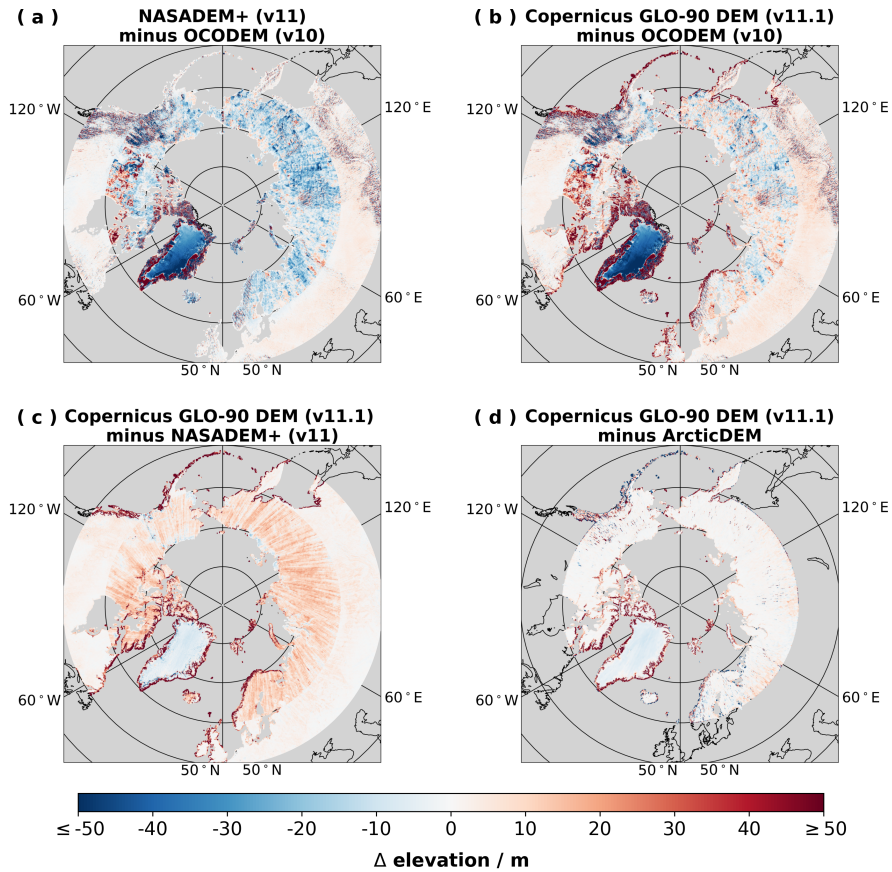
Figure 2. Maps of differences in elevation over northern high latitude region among the OCODEM, NASADEM+, ArcticDEM, and Copernicus GLO-90 DEM at 0.1^\circ \times 0.1^\circ resolution. Refer to Sect. 2.3 to 2.6 for descriptions of the DEM data.
