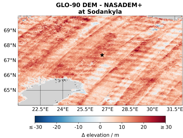
Figure 11. Map of the differences in elevation between the Copernicus GLO-90 DEM and NASADEM+ in the area around the TCCON site at Sodankylä, Finland (site location shown at the black star).
