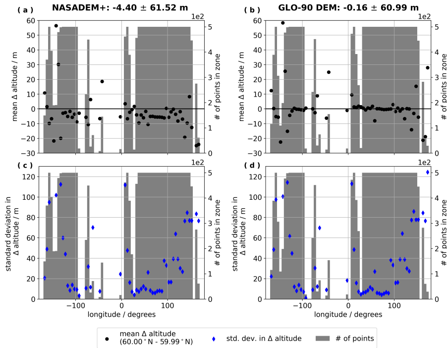
Figure 4. Shifts in DEM elevations crossing the 60° N parallel in the NASADEM+ and Copernicus-GLO-90 DEM. For these plots the average elevations are taken from each DEM within each 0.01° latitude by 5° longitude region and the difference is taken as the region north (60.00° N to 60.01° N) of 60° N minus the region south (59.99° N to 60.00° N) of 60° N. Left, (a) and (c), are the NASADEM+ and right, (b) and (d) are the Copernicus-GLO-90 DEM. Above each plot is the global average \pm one standard deviation of all zonal differences across this parallel for each DEM. Also shown are the number of DEM data points in each 5° zonal bin (i.e., there are fewer DEM data points where there is ocean). Some differences are a real result of topographical changes (commonly corresponding to higher standard deviations in altitude, shown in (c) and (d)), but one would not expect to see a global average difference when crossing this parallel.
