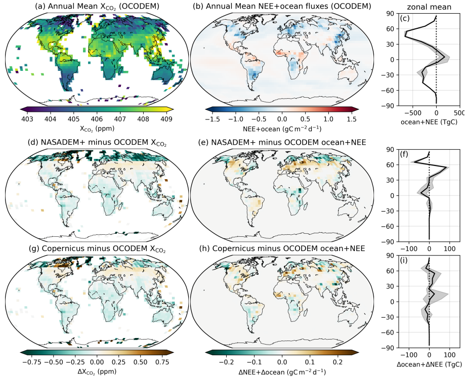
Figure 12. Surface \text{CO}_2 fluxes estimated from ACOS v10 data with the OCODEM, NASADEM+, and Copernicus-GLO-90 DEM. The top row shows results from the original v10 retrievals: (a) map of annual mean X_{\text{CO}_2} at 4^\circ \times 5^\circ resolution; (b) map of estimated annual mean NEE+ocean at 4^\circ \times 5^\circ resolution; (c) zonal mean of NEE+ocean fluxes with the spread due to different model priors shown as grey shading. The middle row shows the difference between results from v10 retrievals using the NASADEM+ (see Sect. 3.4) and the original v10 retrievals using the OCODEM: (d) map of \Delta X_{\text{CO}_2} = v10[\text{NASADEM+}] - v10[\text{OCODEM}] ; (e) map of \Delta \text{NEE+ocean} = v10[\text{NASADEM+}] - v10[\text{OCODEM}] ; (f) zonal mean of \Delta \text{NEE+ocean} . The bottom row shows the difference between results from v10 retrievals using the Copernicus-GLO-90 DEM and the original v10 retrievals using the OCODEM: (g) map of \Delta X_{\text{CO}_2} = v10[\text{Copernicus}] - v10[\text{OCODEM}] ; (h) map of \Delta \text{NEE+ocean} = v10[\text{Copernicus}] - v10[\text{OCODEM}] ; (i) zonal mean of \Delta \text{NEE+ocean} .
