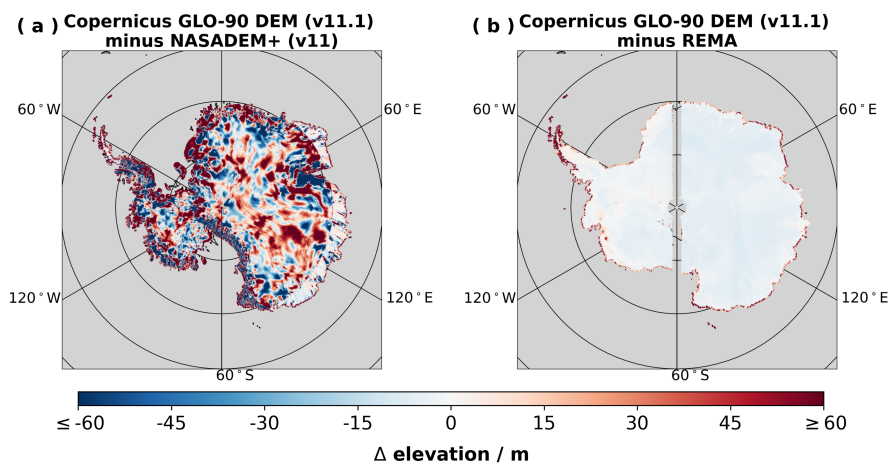
Figure 3. Maps of differences in elevation over Antarctica among the NASADEM+, Copernicus GLO-90 DEM, and REMA at 0.1^\circ \times 0.1^\circ resolution. The NASADEM+ collection utilized the older RAMPv2 DEM data in Antarctica.
