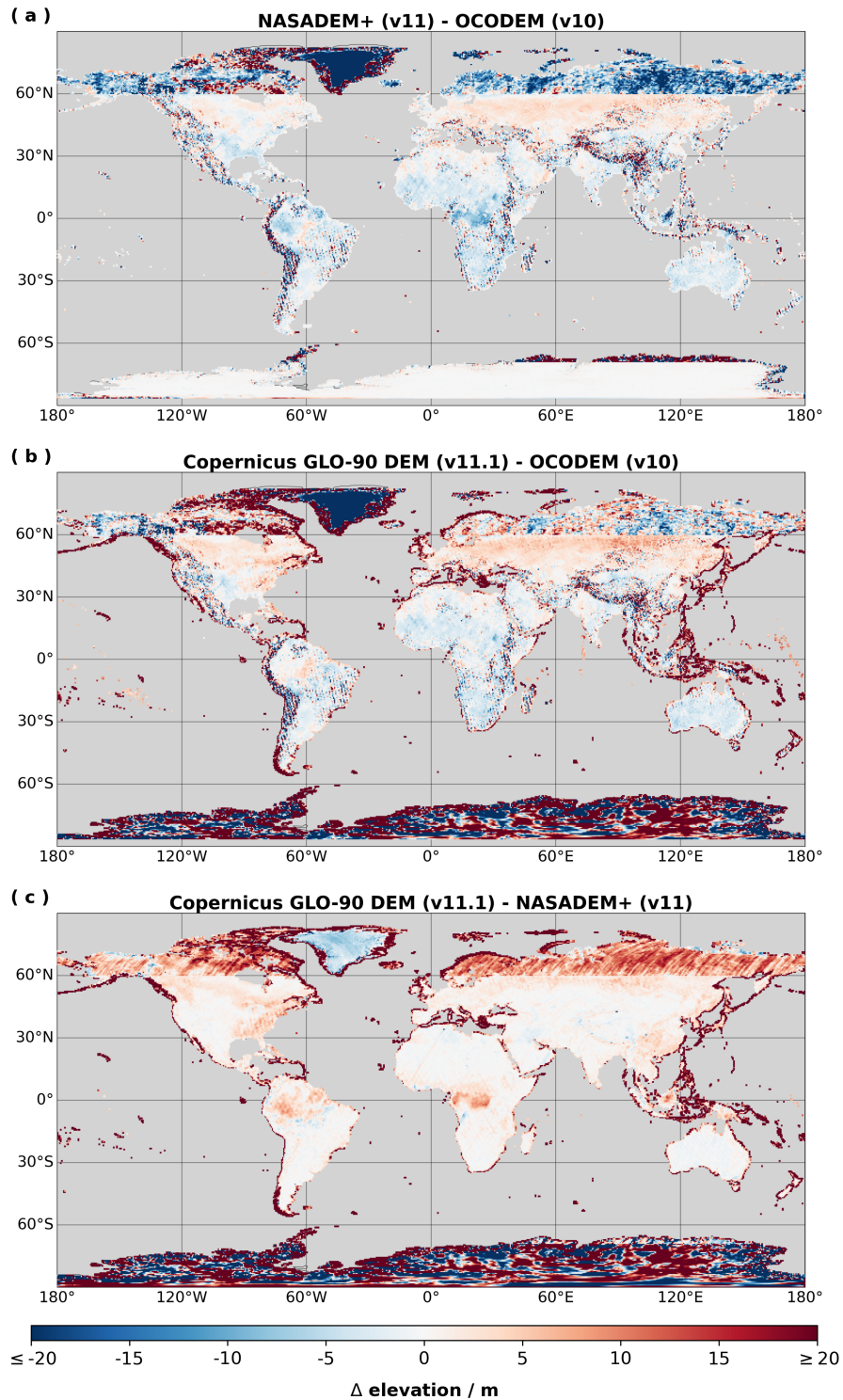
Figure 1. Global map of differences in elevation among OCODEM, NASADEM+, and Copernicus-GLO-90 DEM at 0.5^\circ \times 0.5^\circ resolution. The NASADEM+ collection utilized the older RAMPv2 DEM data in Antarctica, and the ASTER GDEMv3 data in most areas north of 60^\circ\text{N} .
