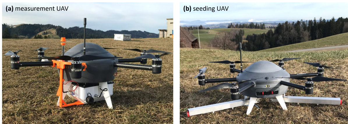
Figure 1. Images of the two UAVs: (a) the measurement UAV, a Metadrone equipped with a Portable Optical Particle Spectrometer (white box) and an extended inlet (orange-capped tube), and (b) the seeding UAV, a Metadrone with two attached burn-in-place seeding flares.
