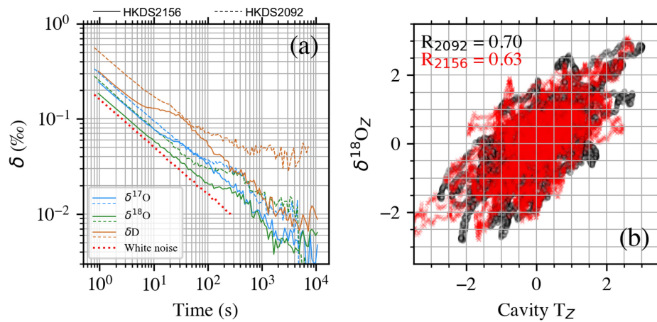
795 Figure 8: 10 hours analysis of the same water vapor source using two water isotope analyzers (HKDS2092, HKDS2156). (a) Allan Deviations of the two analyzers showing “bumps” at different averaging times for the two instruments. The Allan deviation of white noise is reported as a red dotted line for reference. (b) Z-scores of \delta^{18}\text{O} vs z-scores of cavity temperature of the two instruments (HKDS2092 in black, HKDS2156 in red). Standard deviations of \delta^{18}\text{O} are 0.02‰ and 0.01‰ for HKDS2092 and HKDS2156, respectively. Standard deviations of cavity temperature are 0.002 and 0.001 K for HKDS2092 and HKDS2156, respectively.
