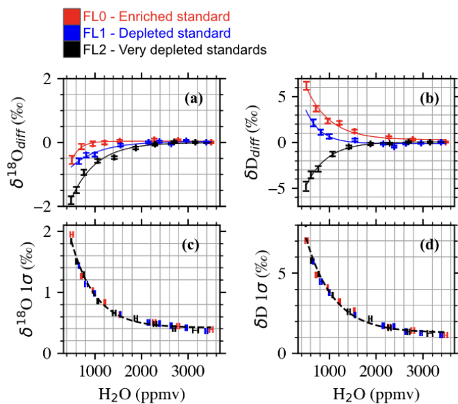
790 Figure 7: Humidity-isotope characterization of the HKDS2092 analyzer between 500-3500 ppmv using three different isotopic standards. (a) and (b) humidity - isotope dependency for for \delta^{18}\text{O} and \delta\text{D} , respectively. Dependency reported as the difference between the isotopic composition at 3500 ppmv and isotopic composition for each humidity step. Error bars are standard errors of the mean. Lines are exponential decay models that best fit the observations of each isotope standard. (c) and (d) standard deviation of \delta^{18}\text{O} and \delta\text{D} for each humidity step and different standards. Error bars on the horizontal axis are standard deviations. For all panels, results of the best fits are reported in supplementary material Table S5.
