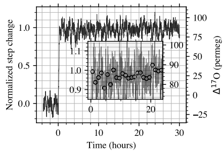
810 Figure 10: Calibrated and normalized step change for \Delta^{17}\text{O} . Black line is a 15-minute window moving average. Inset plot: detail of the 0-24h region. Grey line is the same as in the main plot. Circles are 1-hour averaged sample mean.
