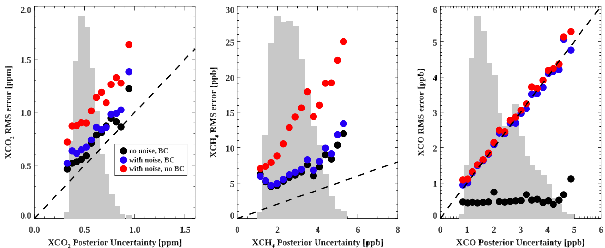
Figure 9. Baseline retrieval actual errors in target gas column fractions plotted vs. the posterior uncertainty. Shown are the noiseless errors with bias correction (black), with noise with bias correction (blue), and with noise without bias correction (red).
