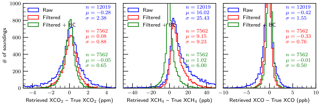
Figure 13. Same as figure 6 but with imperfect knowledge of polarization.
