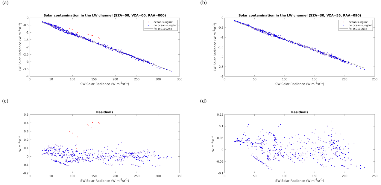
Figure 3. Solar contamination in the LW channel. Represented here is the contamination for (a) the nadir view of the BBR for a sunglint geometry (SZA=0°, VZA=0°, RAA=0°), (b) the off-nadir view for a non-sunglint geometry (SZA=30°, VZA=55°, RAA=90°), (c) the residuals of the fit for the nadir view in (a) and (d) residuals for the off-nadir view in (b).
