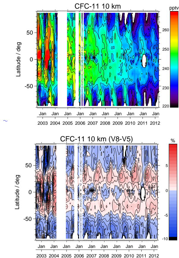
Figure 10. Latitude-time cross sections of the previous version, V5, of CFC-11 at 10 km altitude (top), and relative difference between V8 and V5 of CFC-11 at 10 km (in terms of (V8 - V5)/V5 \cdot 100 ) (bottom). For details, see Fig. 5.
