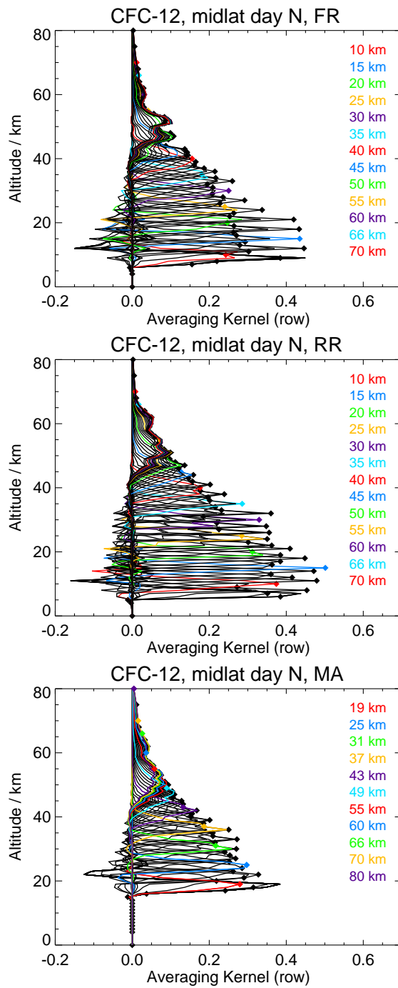
Figure 3. Averaging kernels of northern midlatitude day CFC-12 FR (top), RR (middle), and MA (bottom) measurements. These averaging kernels refer to limb sequences recorded at 46.1°N, 155.1°W, on 14 January 2003 (top), 48.4°N, 116.4°W, on 4 January 2009 (middle), and 48.0°N, 179.65°E, on 11 January 2009 (bottom). Every fifth averaging kernel row is marked by color, and the diamonds mark the altitude of the retrieval grid point.
