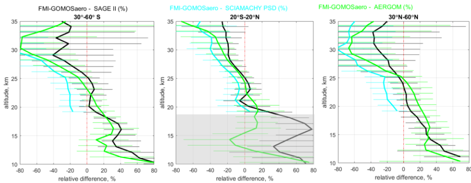
390 Figure 8. Median (solid lines) and 16th and 84th percentiles (horizontal bars) of relative differences between FMI-GOMOSaero and other datasets, for latitudes 30°-60°S (left), 20°S-20°N (center), and 30°-60°N (right). Comparison with SAGE II and SCIAMACHY PSD are for 525 nm. In comparison with AERGOM, data at 550 nm are used. The gray shading shows the region of tropical troposphere.
