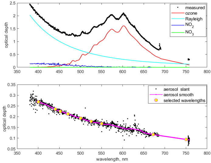
Figure 2. Illustration of the GOMOS aerosol retrieval algorithm. Top: measured optical depth spectrum (black) and contributions due to ozone (red), Rayleigh scattering (cyan), \text{NO}_2 (blue) and \text{NO}_3 (green). Bottom: original (black) and smoothed (magenta) residuals.
