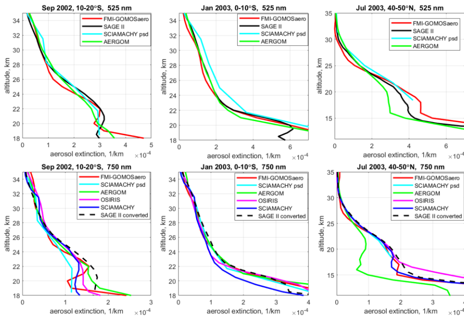
325 Figure 6. Comparison of new GOMOS retrieved profiles with data from several satellite instruments. Top panels: comparisons for the wavelength 525 nm, bottom panels: comparisons for the wavelength 750 nm. The datasets are specified in the legend. The dates and latitudes are indicated in the panel titles.
