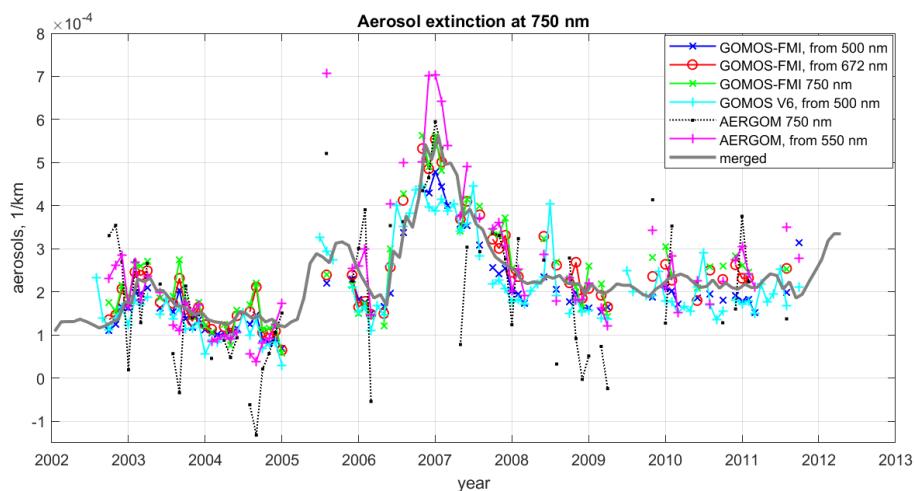
Figure 13. GOMOS aerosol extinction at 750 nm computed by different methods: GOMOS-FMI retrieved at 750 nm (green), GOMOS-FMI converted from 672 nm (red), GOMOS-FMI converted from 500 nm (blue), GOMOS IPF v6 converted from 500 nm (cyan) and AERGOM retrieved at 750 nm (black) and converted from 550 nm (magenta). Thick grey line indicates merged aerosol extinction. All time series are for the latitude bin 0-10°N and altitude 22 km. AERGOM data are shown only for the same times that are present in FMI-GOMOSaero data.
