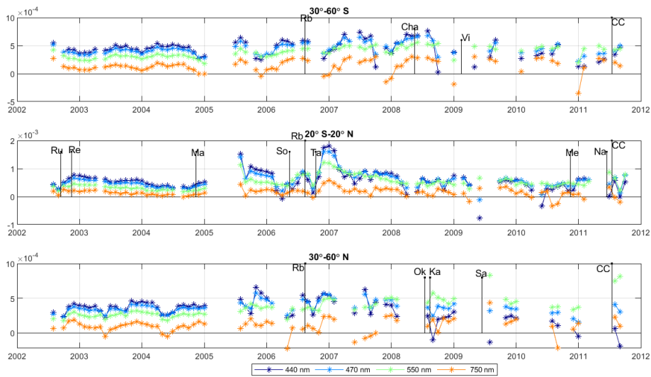
465 Figure 12. As Figure 11, but for AERGOM v.4 aerosol extinction. AERGOM data are shown only for the same latitude bins and times that are present in FMI-GOMOSaero data.
