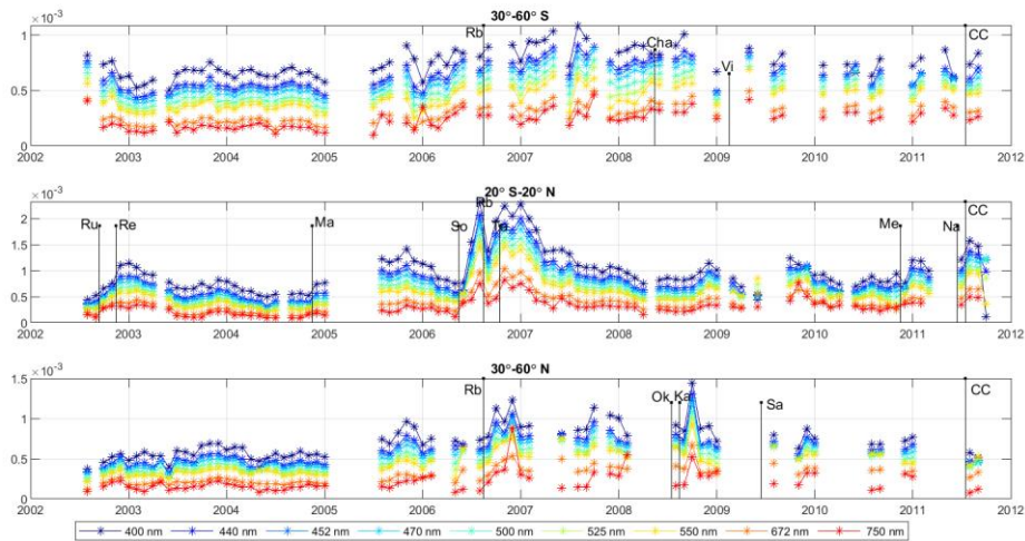
445 Figure 11. Time series of GOMOS-FMI aerosol extinction (1/km) at 20 km in the latitude zones 30°-60° S (top), 20°S-20°N (center) and 30°-60° N (bottom). The wavelengths are indicated in the figure legend. The volcanoes are indicated by black bars with the length proportional to volcanic explosivity index (VEI). Volcanoes with VEI \geq 5 are shown for all latitude zones, and with VEI > 3 in the corresponding latitude zones.
