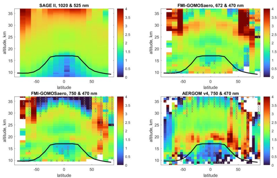
305 Figure 5 Average Ångström exponent in 2003-2004 computed using SAGE II, FMI-GOMOSaero and AERGOM data. Wavelength combinations and instruments are indicated on the panels. The data with average estimated uncertainty exceeding 100% are marked with grey crosses. Black lines indicate mean tropopause. Empty boxes for AERGOM correspond to negative aerosol extinction data, for which Ångström exponent has not been evaluated. SAGE II data are cloud filtered.
