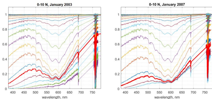
Figure 1. Examples of GOMOS averaged transmittance spectra in the equatorial region 0-10°N, in January 2003 (background aerosols) and in January 2007 (after volcanic eruptions), from 100 km down to the lowest altitude. Red thick lines highlight transmittances at 20 km. For visibility, the transmittance spectra are plotted with the vertical step of 3 km. The lowest altitude is 8 km on the left panel and 14 km on the right panel.
