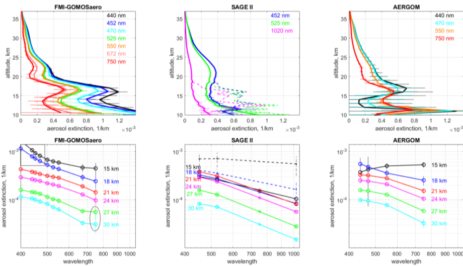
Figure 4 Top: monthly mean aerosol profiles at several wavelengths, September 2002, 10°-20° S for FMI-GOMOSAero (left), SAGE II (center) and AERGOM v4. The wavelengths are specified in the legend. For SAGE II, profiles with (solid lines) and without cloud filtering (dashed lines) are shown. Bottom: aerosol extinction spectra at selected altitudes specified on the panels. For visual aid, colored stars on bottom middle panel indicate 750 nm aerosol extinction computed using SAGE II extinctions at 525 and 1020 nm. Oval and rectangle in the bottom left panel indicate problematic regions, which are discussed in the text.
