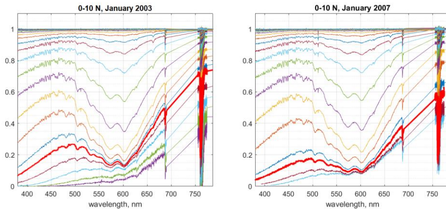
115 Figure 1. Examples of GOMOS averaged transmittance spectra in the equatorial region 0-10°N, in January 2003 (background aerosols) and in January 2007 (after volcanic eruptions), from 100 km down to the lowest altitude. Red thick lines highlight transmittances at 20 km. For visibility, the transmittance spectra are plotted with the vertical step of 3 km. The lowest altitude is 8 km on the left panel and 14 km on the right panel.
