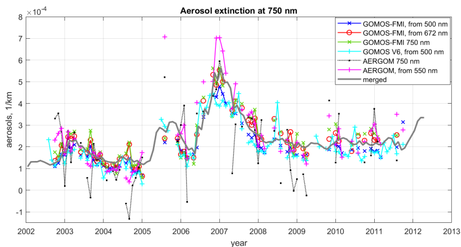
385 Figure 13. GOMOS aerosol extinction at 750 nm computed by different methods: GOMOS-FMI retrieved at 750 nm (green), GOMOS-FMI converted from 672 nm (red), GOMOS-FMI converted from 500 nm (blue), GOMOS IPF v6 converted from 500 390 nm (cyan) and AERGOM retrieved at 750 nm (black) and converted from 550 nm (magenta). Thick grey line indicates merged aerosol extinction. All time series are for the latitude bin 0-10°N and altitude 22 km. AERGOM data are shown only for the same times that are present in FMI-GOMOSaero data.
