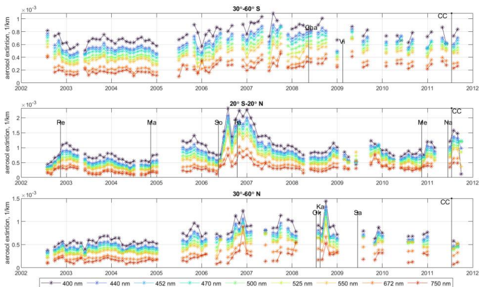
Figure 11. Time series of GOMOS-FMI aerosol extinction (1/km) at 20 km in the latitude zones 30°-60° S (top), 20°S-20°N (center) and 30°-60° N (bottom). The wavelengths are indicated in the figure legend. The volcanoes are indicated by black bars with the length proportional to volcanic explosivity index (VEI). Volcanos with VEI \geq 5 are shown for all latitude zones, and with VEI \geq 3 in the corresponding latitude zones.
