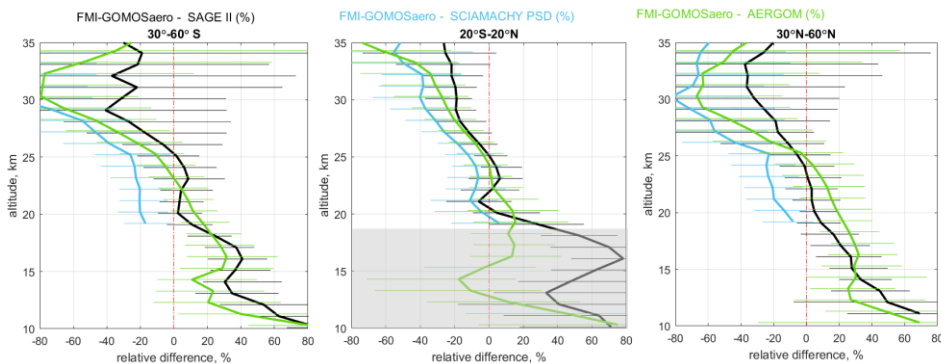
310 Figure 8. Median (solid lines) and 16th and 84th percentiles (horizontal bars) of relative differences between FMI-GOMOSaero and other datasets, for latitudes 30°-60°S (left), 20°S-20°N (center), and 30°-60°N (right). Comparison with SAGE II and SCIAMACHY PSD are for 525 nm. In comparison with AERGOM, data at 550 nm are used. The gray shading shows the region of tropical troposphere.
