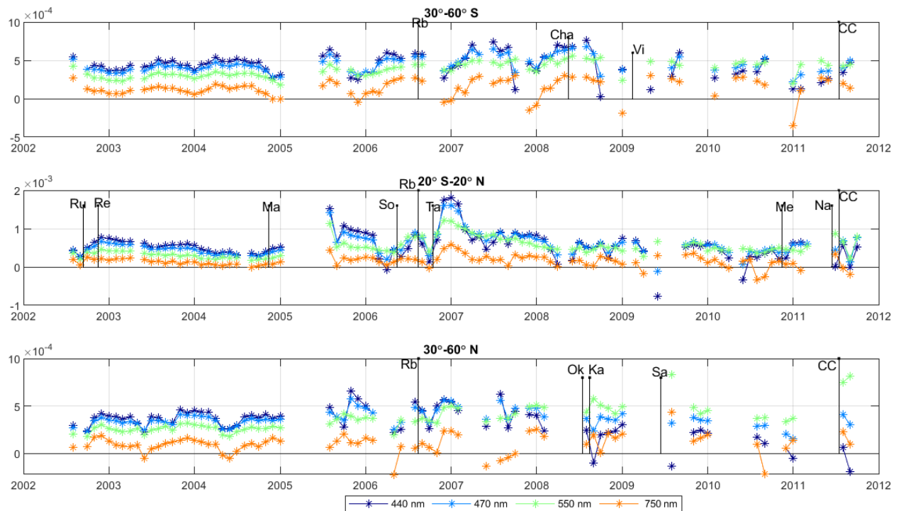
375 Figure 12. As Figure 11, but for AERGOM v.4 aerosol extinction. AERGOM data are shown only for the same latitude bins and times that are present in FMI-GOMOSAero data.
