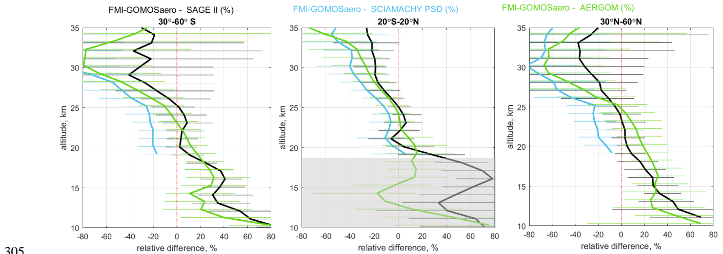
Figure 8. Median (solid lines) and 16th and 84th percentiles (horizontal bars) of relative differences between FMI-GOMOSaero and other datasets, for latitudes 30°-60°S (left), 20°S-20°N (center), and 30°-60°N (right). Comparison with SAGE II and SCIAMACHY PSD are for 525 nm. In comparison with AERGOM, data at 550 nm are used. The gray shading shows the region of tropical troposphere.
