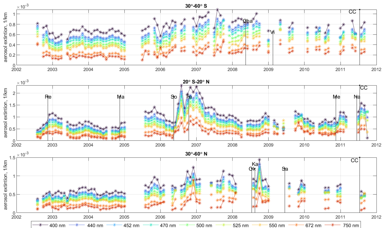
355 Figure 11. Time series of GOMOS-FMI aerosol extinction (1/km) at 20 km in the latitude zones 30°-60° S (top), 20°S-20°N (center) and 30°-60° N (bottom). The wavelengths are indicated in the figure legend. The volcanoes are indicated by black bars with the length proportional to volcanic explosivity index (VEI). Volcanoes with VEI \geq 5 are shown for all latitude zones, and with VEI > 3 in the corresponding latitude zones.
