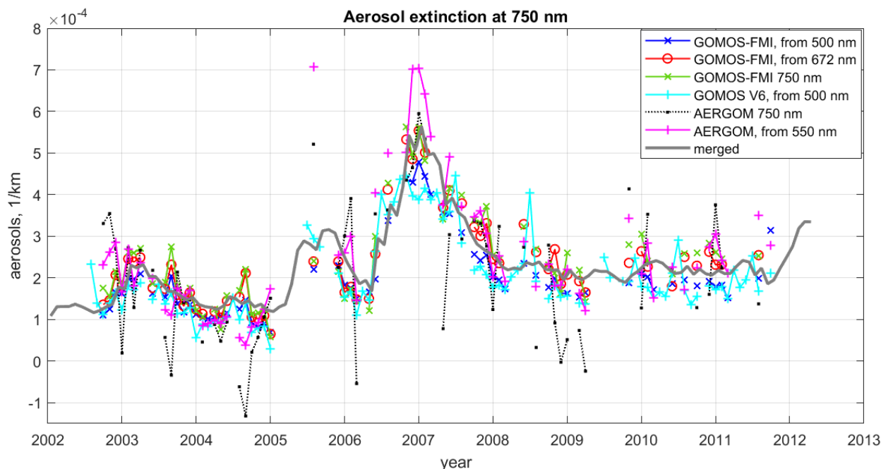
380 Figure 13. GOMOS aerosol extinction at 750 nm computed by different methods: GOMOS-FMI retrieved at 750 nm (green), GOMOS-FMI converted from 672 nm (red), GOMOS-FMI converted from 500 nm (blue), GOMOS IPF v6 converted from 500 nm (cyan) and AERGOM retrieved at 750 nm (black) and converted from 550 nm (magenta). Thick grey line indicates merged aerosol extinction. All time series are for the latitude bin 0-10°N and altitude 22 km. AERGOM data are shown only for the same times that are present in FMI-GOMOSaero data.
