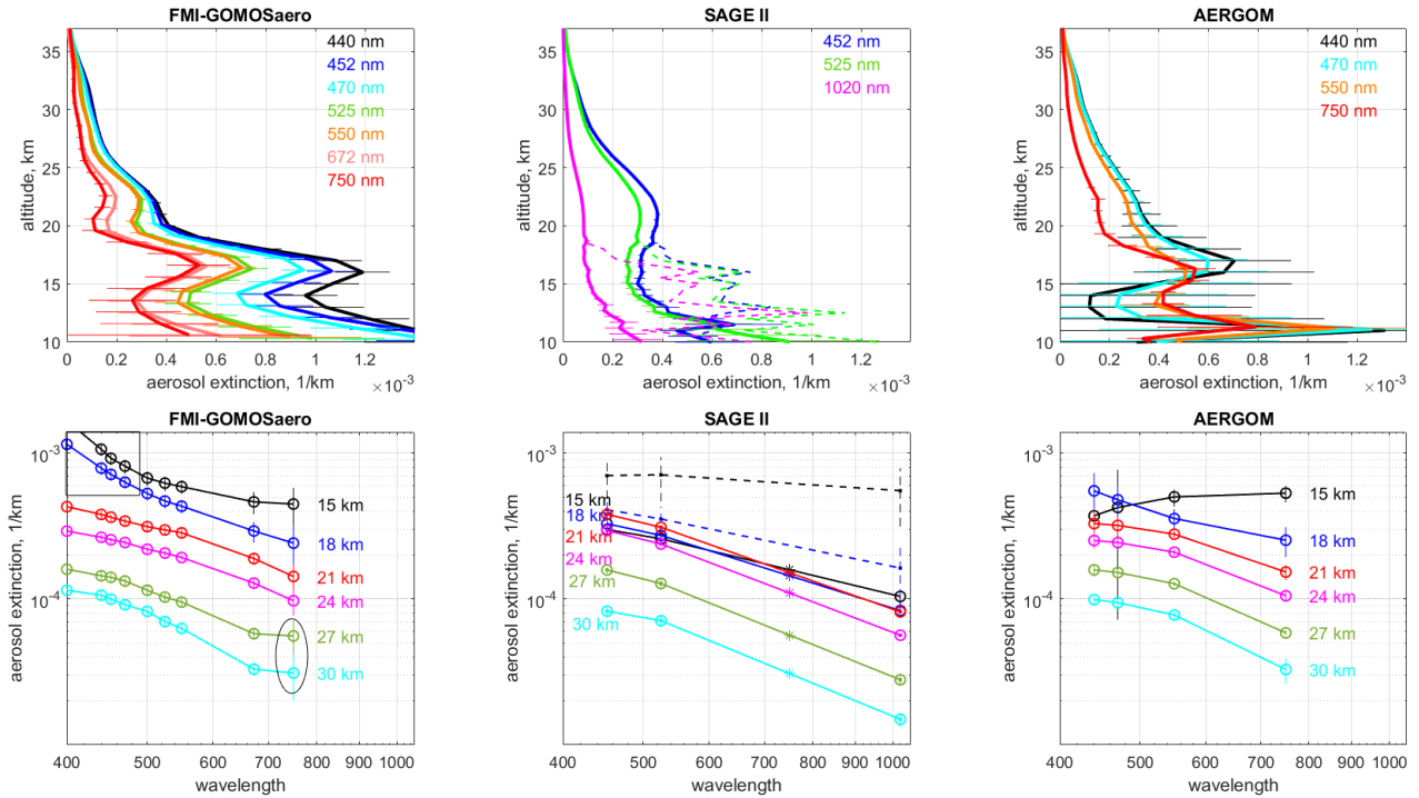
205 Figure 4 Top: monthly mean aerosol profiles at several wavelengths, September 2002, 10°-20° S for FMI-GOMOSaero (left), SAGE II (center) and AERGOM v4. The wavelengths are specified in the legend. For SAGE II, profiles with (solid lines) and without cloud filtering (dashed lines) are shown. Bottom: aerosol extinction spectra at selected altitudes specified on the panels. For visual aid, colored stars on bottom middle panel indicate 750 nm aerosol extinction computed using SAGE II extinctions at 525 and 1020 nm. Oval and rectangle in the bottom left panel indicate problematic regions, which are discussed in the text.
