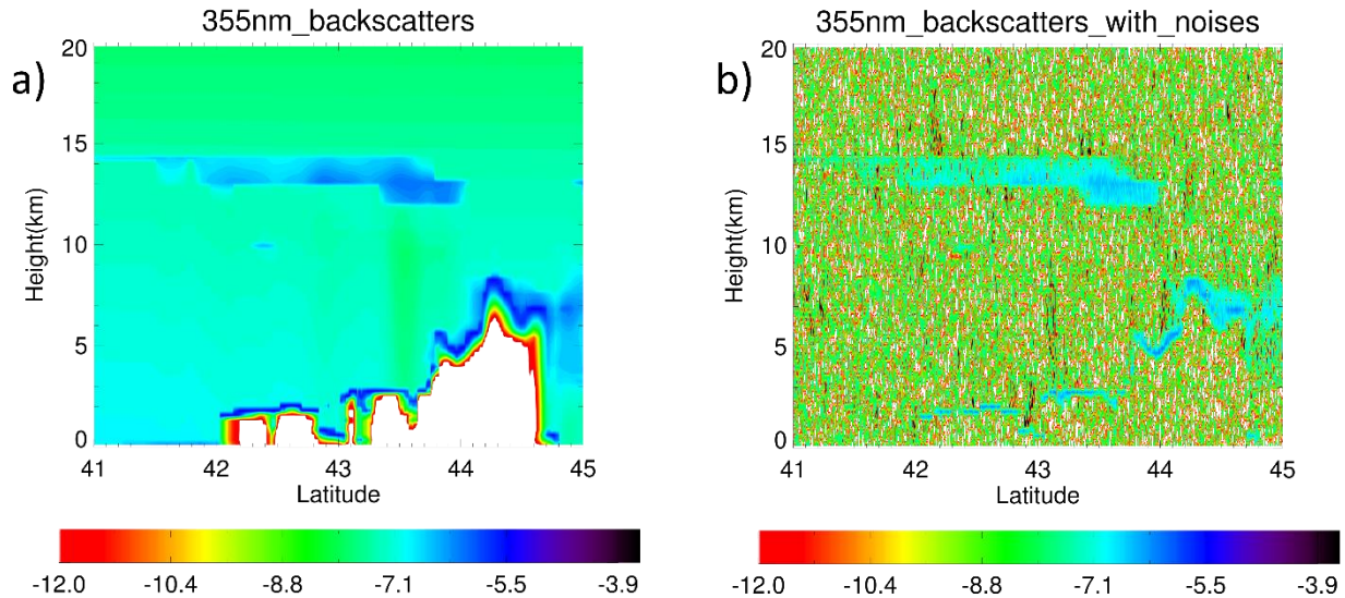
Figure 8. Examples of 355 nm total attenuated backscattering coefficients of ATLID of the standard product (a) and with random noise (b). The contour is a log scale of backscattering coefficients ( \text{m}^{-1}\cdot\text{str}^{-1} ).
