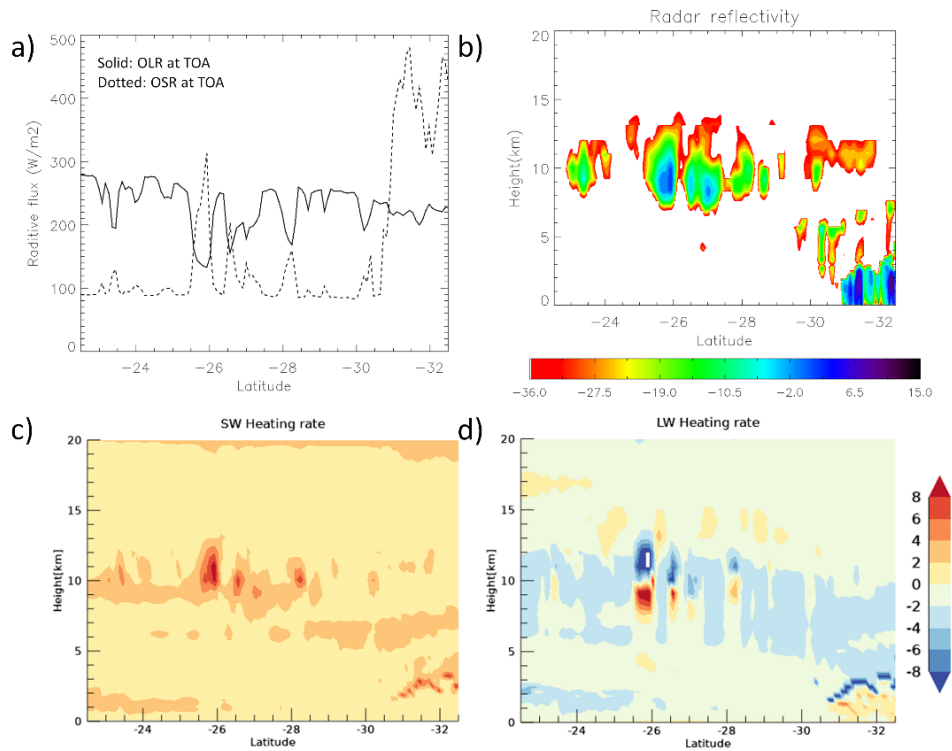
Figure 12. Examples of BBR simulations (a) and corresponding CPR signals (b). Short-wave (c) and long-wave (d) radiative heating rates are also provided as JAXA L1 data for use in validation.
