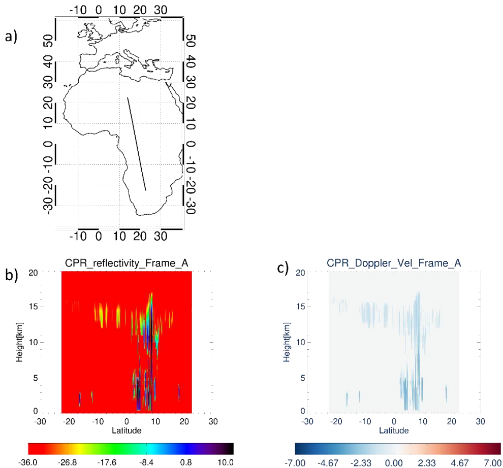
Figure 3. CPR data of the JAXA L1 data for Frame A over the African continent (a), with radar reflectivities (b) and Doppler velocities (c).
