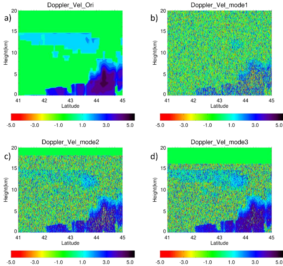
170 Figure 6. Examples of Doppler velocity for the standard L1 data using a 20 km observation window (a), high mode (b), 18 km observation window and middle mode (c), and 16 km observation window and low mode (d).
