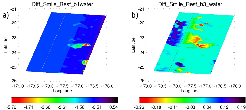
255 Figure 11. Examples of differences between MSI signal with the response function on the nadir and with the smile effect for the 0.67 \mu\text{m} (Band 1) (a) and 1.65 \mu\text{m} (Band 3) (b) channels over the ocean, for the descending mode where the satellite is moving southwestward. The base is the MSI signal with the response function on the nadir. The solid line is the location of the nadir.
