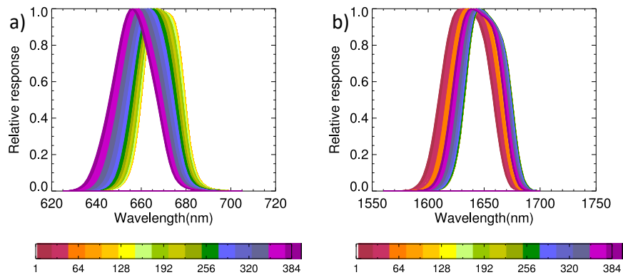
Figure 10. Response functions of MSI (considered the SMILE effect) for the 0.67 \mu\text{m} channel (Band 1) (a) and the 1.65 \mu\text{m} channel (Band 3) (b). Colors indicate MSI pixel numbers.
