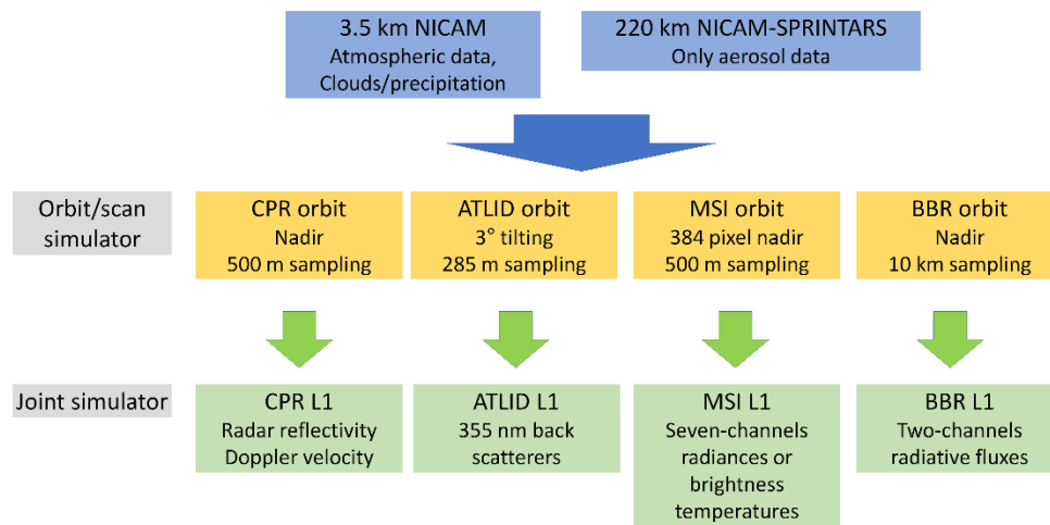
Figure 2. Flowchart for production of JAXA L1 data.
