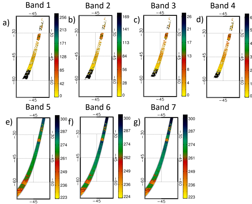
225 Figure 9. Examples of MSI data over the ocean for Frame F for seven channels at 0.67 (a), 0.865 (b), 1.65 (c), 2.21 (d), 8.80 (e), 10.8 (f), and 12.0 \mu\text{m} (g). The contours of the upper panels are radiance ( \text{W}\cdot\text{m}^{-2}\cdot\text{str}^{-1}\cdot\mu\text{m}^{-1} ) and those in the bottom panels are temperatures (K).
