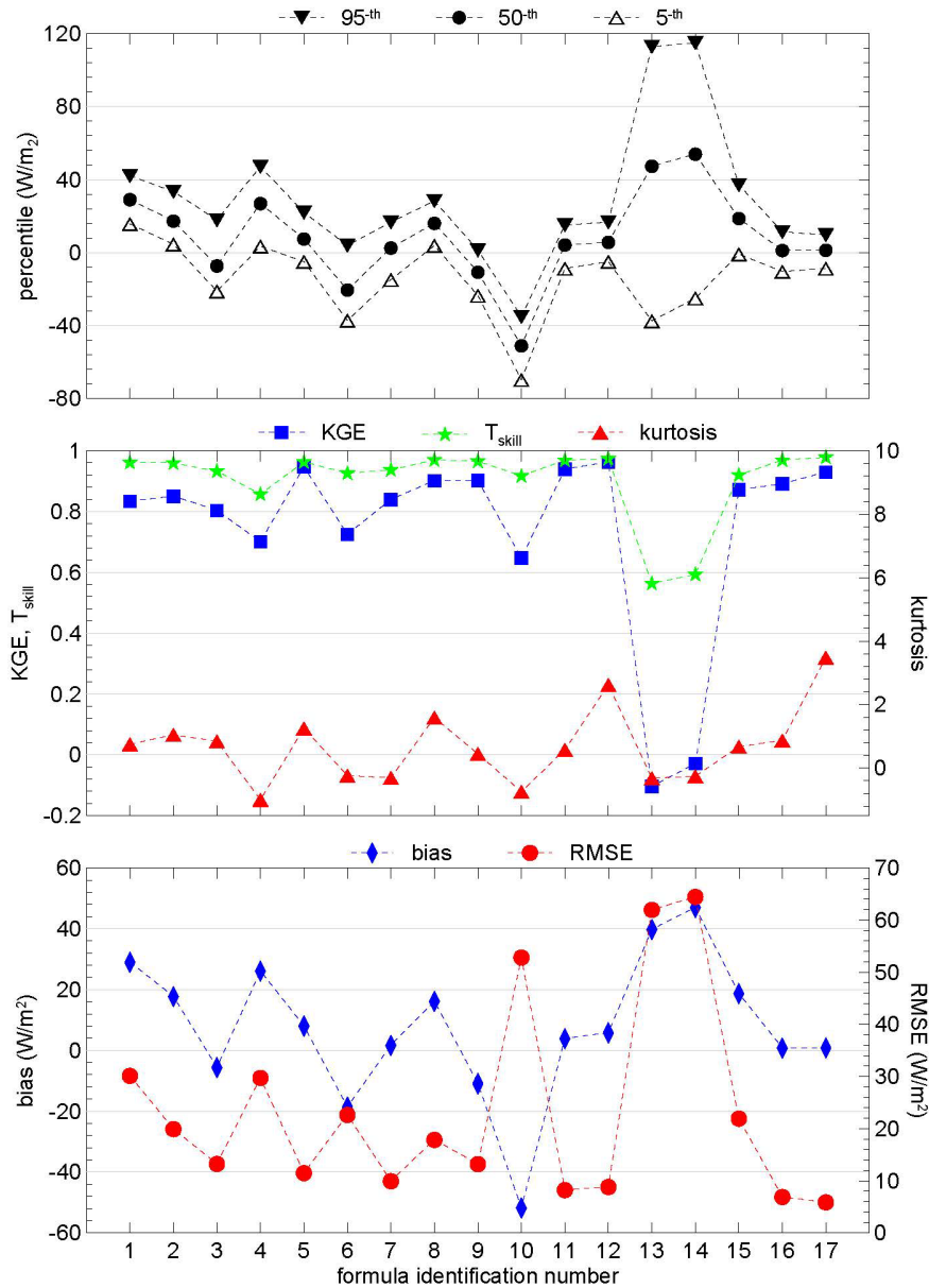
305 Figure 4. Performance parameters of the different formulas for DLI listed in Table 1, tested using 2017 THAAO data: the upper panel shows 95 th , 50 th , and 5 th percentiles (filled triangles, filled circles and empty triangles, respectively) of the differences between estimated and measured values of DLI; the middle panel shows KGE (blue squares, left Y-axis), T skill (green stars, left Y-axis), and
