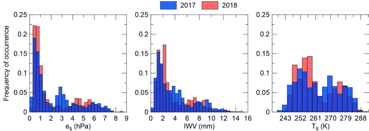
Figure 3. Annual frequency of occurrence of the measured values of e_s , IWV, and T_s at THAAO in 2017 and 2018.
