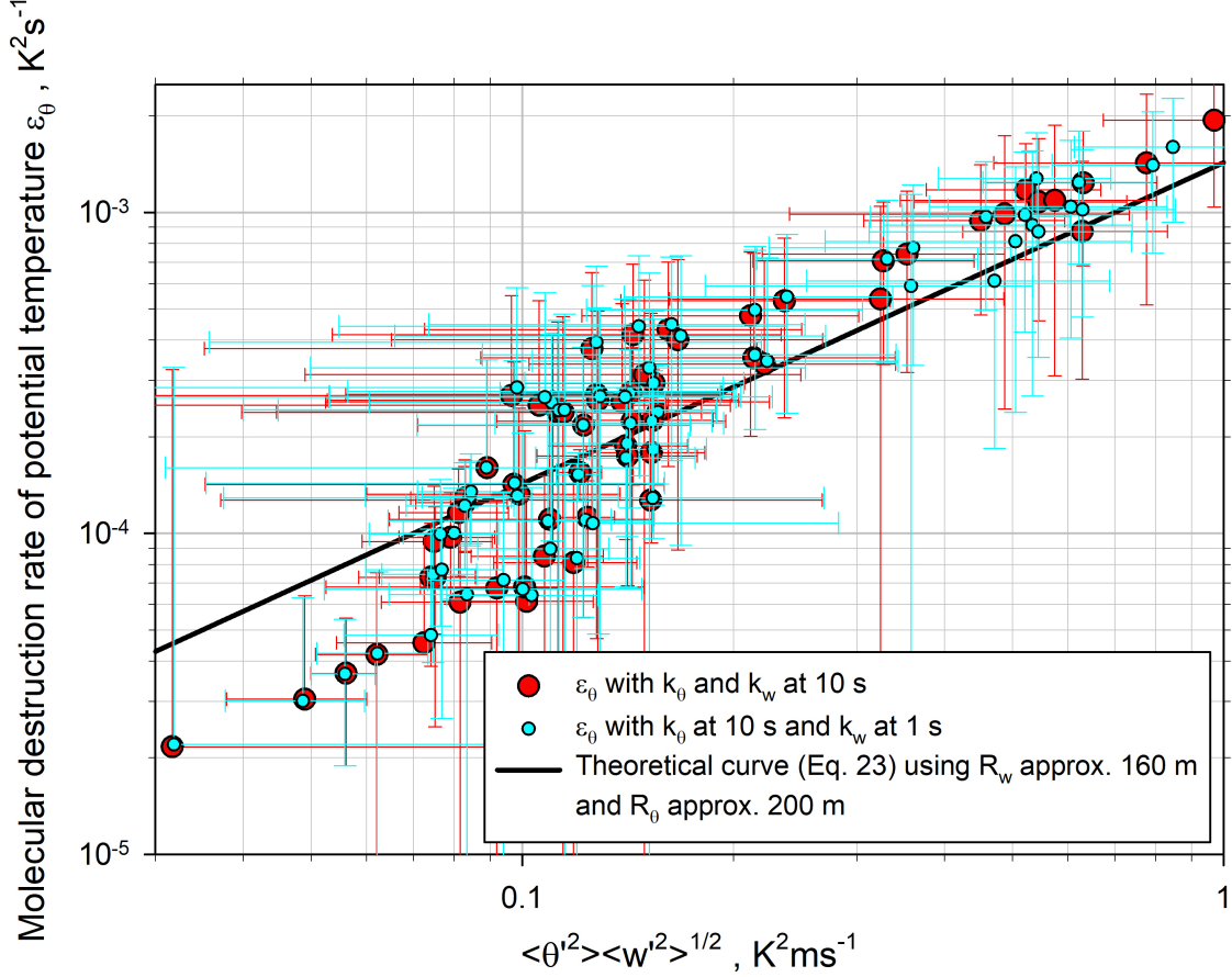
Figure 24. Small cyan circles: \epsilon_\theta derived with k_\theta at 10 s and k_w at 1-s resolutions. Large red circles: \epsilon_\theta derived with k_\theta and k_w at 10-s resolutions. Solid black line: Fit using Eq. 23 combining all data and using mean spatial integral length scales of \mathcal{R}_w \simeq 160 \text{ m} and \mathcal{R}_\theta \simeq 200 \text{ m} .
