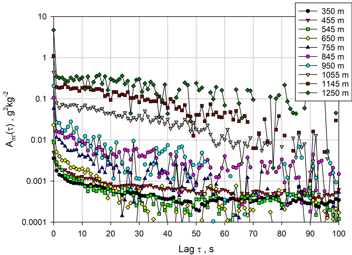
Figure 9. A_{m'}(\tau) for a variety of heights using Eq. 6. Please note that the ACFs are shown on a logarithmic scale in order to capture the large dynamic range of the WVMR variances in dependence of height.
