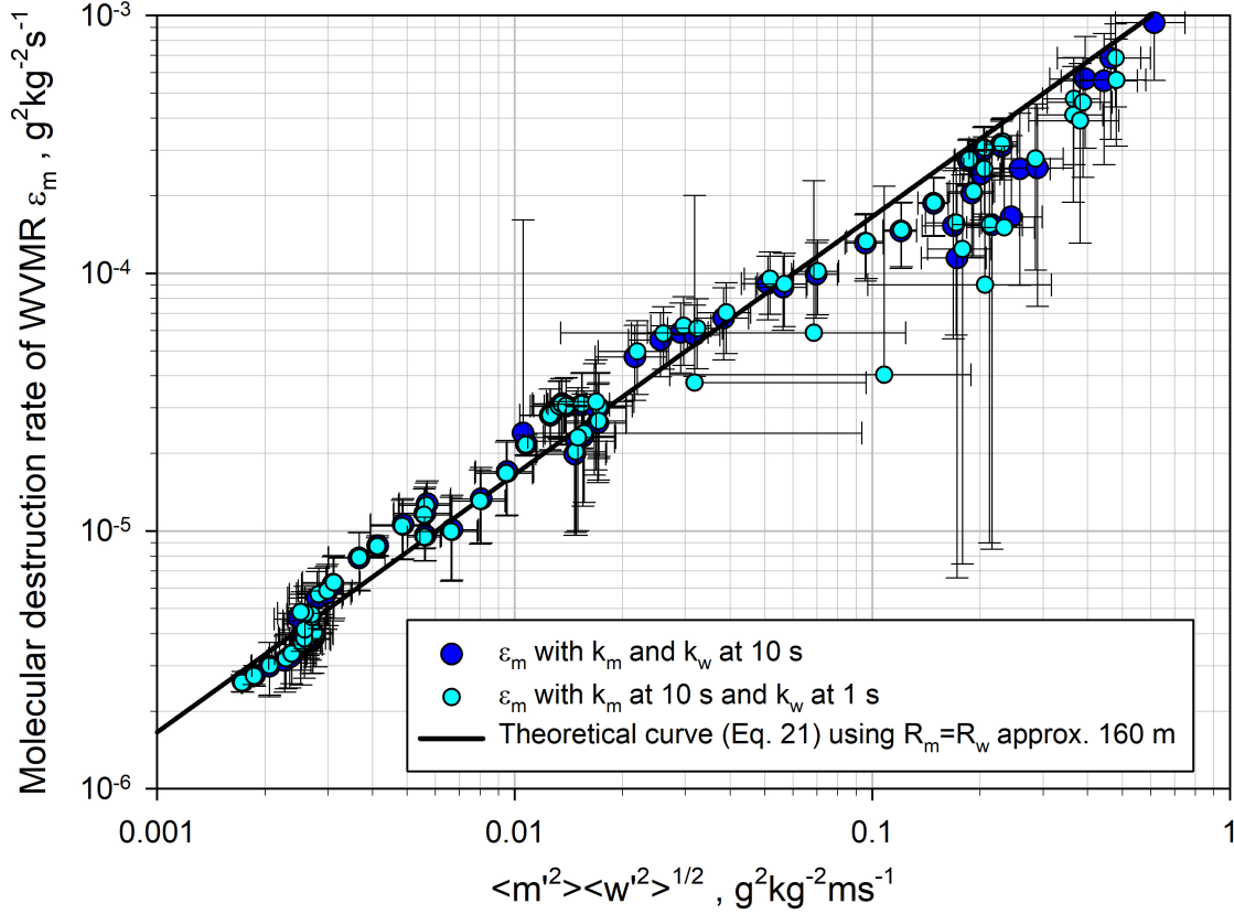
Figure 22. Small cyan circles: \epsilon_m derived with k_m at 10 s and k_w at 1-s resolutions. Large blue circles: \epsilon_m derived with k_m and k_w at 10-s resolutions. Fit using Eq. 21 combining all data and using a mean spatial integral length scales of \mathcal{R}_m = \mathcal{R}_w \simeq 160 \text{ m} .
