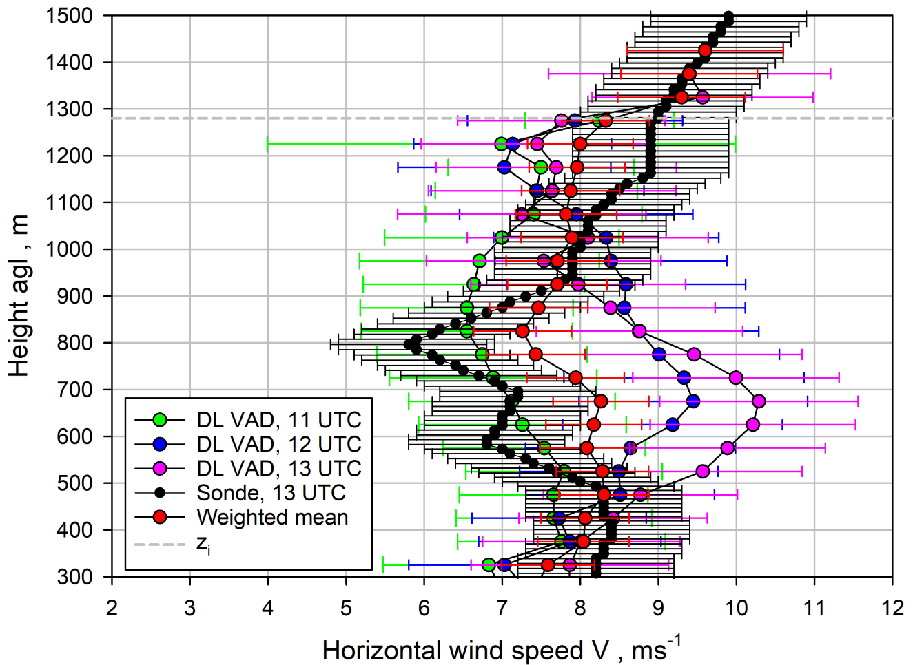
Figure 1. Horizontal wind profiles determined from a radiosonde launch at 13 UTC and three conical DL scans. For the soundings (black bullets), an error of 1 \text{ m s}^{-1} was assumed. The errors in the DL profiles were derived by error propagation of the uncertainty in radial velocities. The red bullets show the weighted average of these profiles, which was used for the derivation of turbulence profiles. The grey dashed line indicates z_i .
