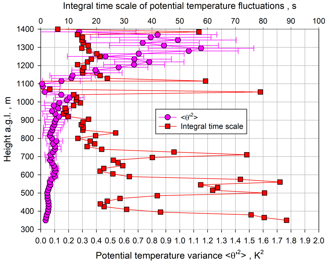
Figure 16. Pink circles: Profiles of the variance of the potential temperature fluctuations for 10-s data. Red squares: The corresponding results for the integral time scale.
