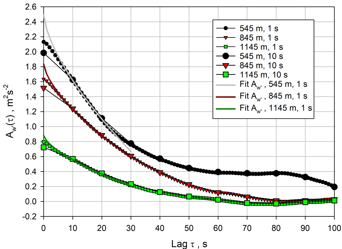
Figure 7. Comparison of A_{w'} using 1 s or 10 s resolutions of the vertical wind speed data. Large symbols: 10 s resolution, smaller symbols: 1 s resolution. Colored solid lines: Fits of the theoretical shapes of the ACFs using the 1-s data.
