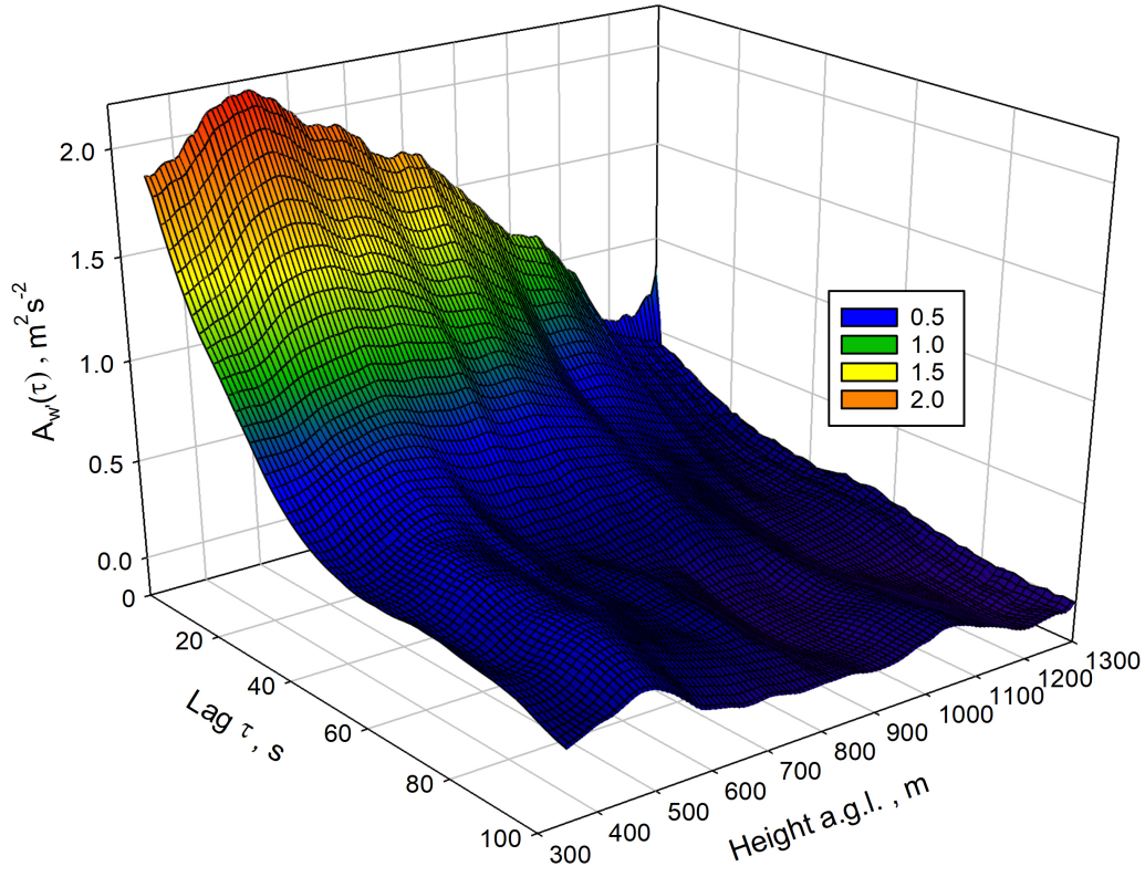
Figure 4. 3D plot of A_{w'}(\tau, z) based on the 1-s data.
