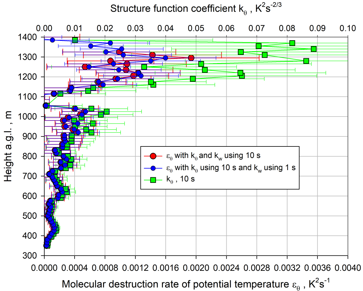
Figure 23. Small blue and large red circles: Profiles of \epsilon_\theta using Eq. 22 derived with k_\theta at 10 s resolution and k_w at 1 s and 10 s resolutions, respectively. Green squares: Corresponding profiles of the ACF coefficients k_\theta with 10 s resolution.
