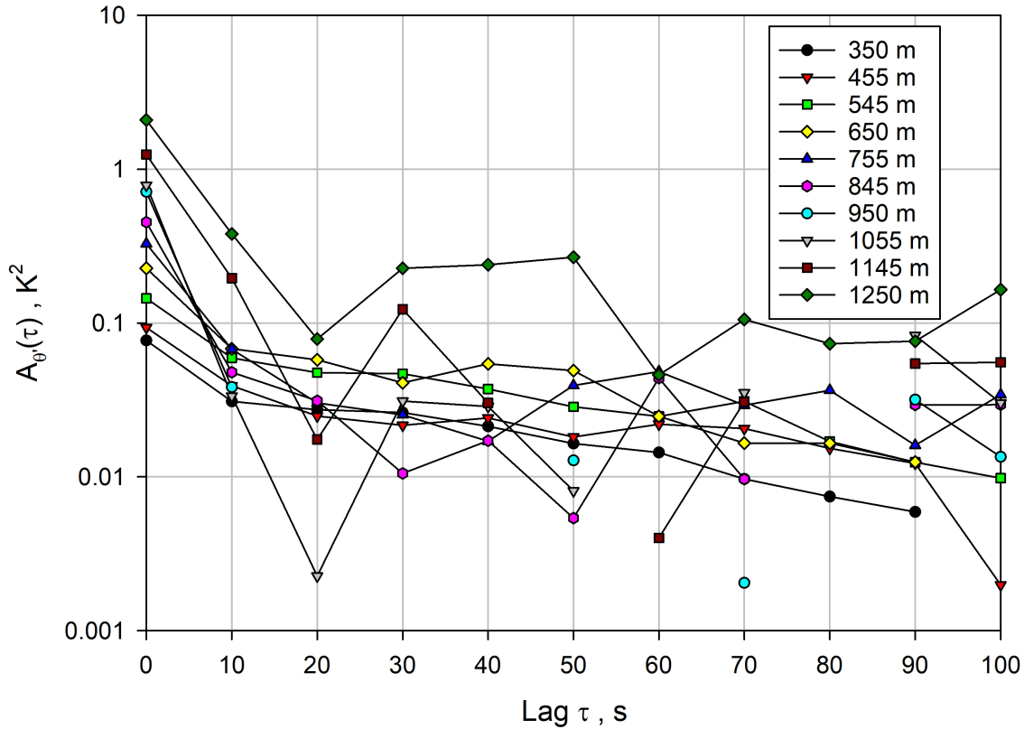
Figure 13. A_{\theta'}(\tau) for a variety of heights using using Eq. 7 at a resolution of 10 s.
