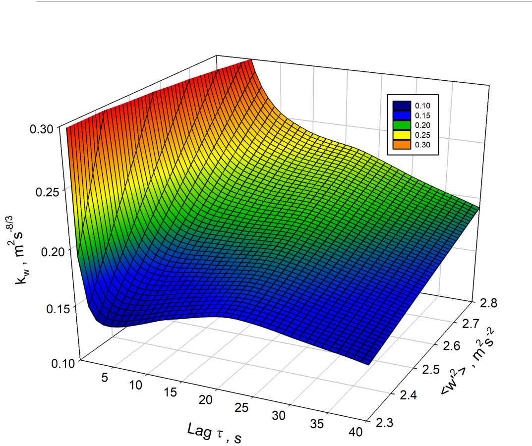
Figure 5. Example of the evaluation of the range of suitable lags according to Eq. 11 at a height of 545 m.
