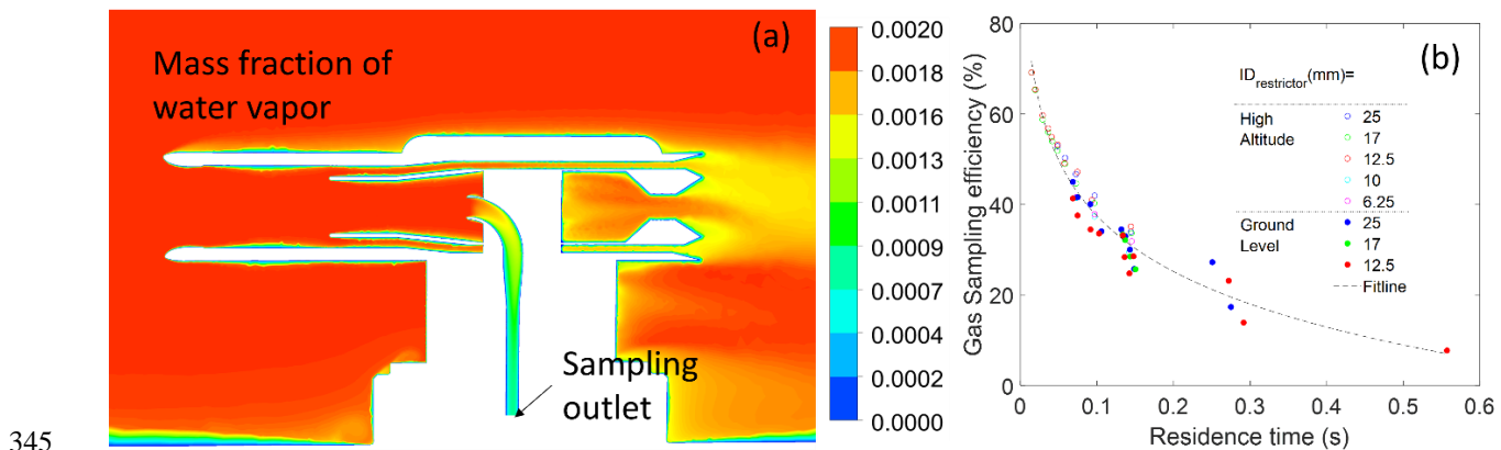
345 Figure 6: (a) contour plot of mass fraction of water vapor of the inlet for 25mm restrictor with freestream velocity of 180\text{m s}^{-1} , freestream turbulence intensity of 3%, and angle of attack of 3^\circ . (b) correlation between residence time inside the sampling tube and the overall gas sampling efficiency at the sampling outlet for all restrictors under different altitudes, freestream velocities and sampling velocities.
