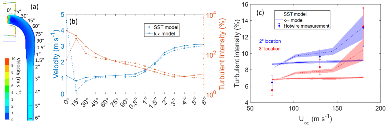
285 Figure 4: Simulation results inside sampling tube for ground level conditions in Table 1 (180 m s -1 , 25mm restrictor, 3% freestream turbulence, 3° angle of attack). (a) Contour of velocity magnitudes in the center plane of the sampling tube, with different locations relevant for (b) labelled. (b) Surface weighted average of turbulent intensities and velocities along the length of the sampling tube. (c) Comparisons of turbulent intensity measured and simulated inside the sampling tube. The simulated sampling flow rate is Q_{\text{sampling}} \approx 19 \text{ SLPM} ; the shading reflects varying TI_{\infty} from 0.5% to 3% in the models. The hotwire measurements show average 290 values for 15 and 20 SLPM sampling flowrate; error bars represent the range of measurements at the two sampling flow rates.
