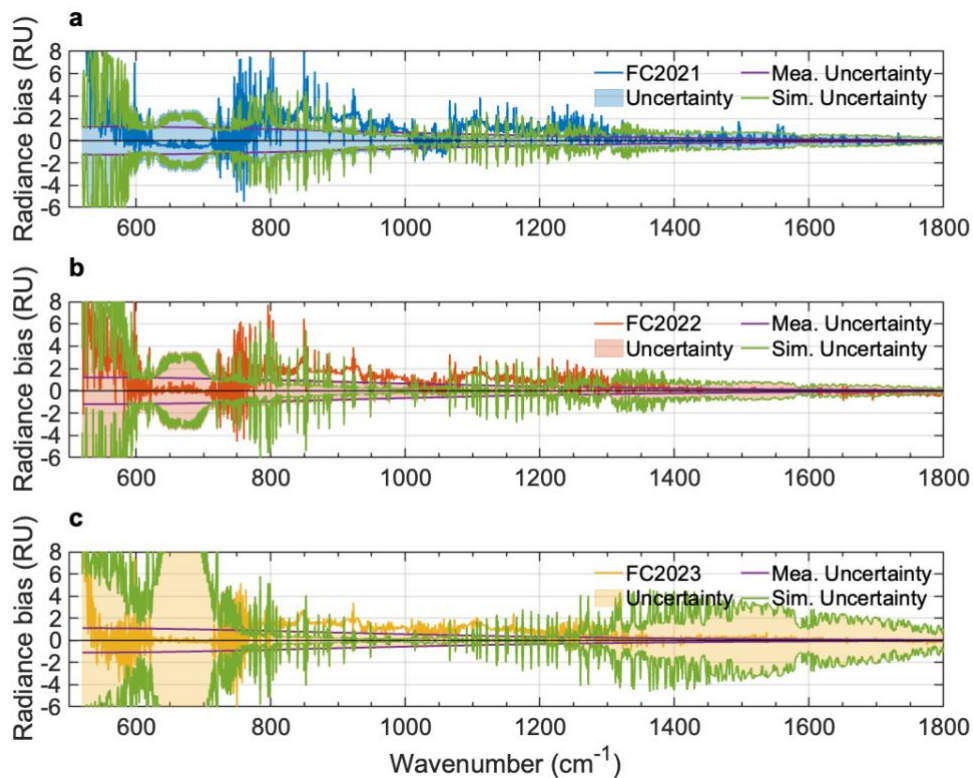
255 Figure 6. AERI radiative closure test results. Each panel represents one field campaign. The blue line in panel a, the orange line in panel b, and the yellow line in panel c represent the DLR bias between 10-min averaged AERI-observed and LBLRTM-simulated spectra. The purple lines and the green lines represent the AERI measurement uncertainty and LBLRTM simulation uncertainty, respectively. The shadings represent the total DLR bias uncertainty. (RU: Radiance Units; 1 RU = 1 mW/[m 2 sr cm -1 ])
