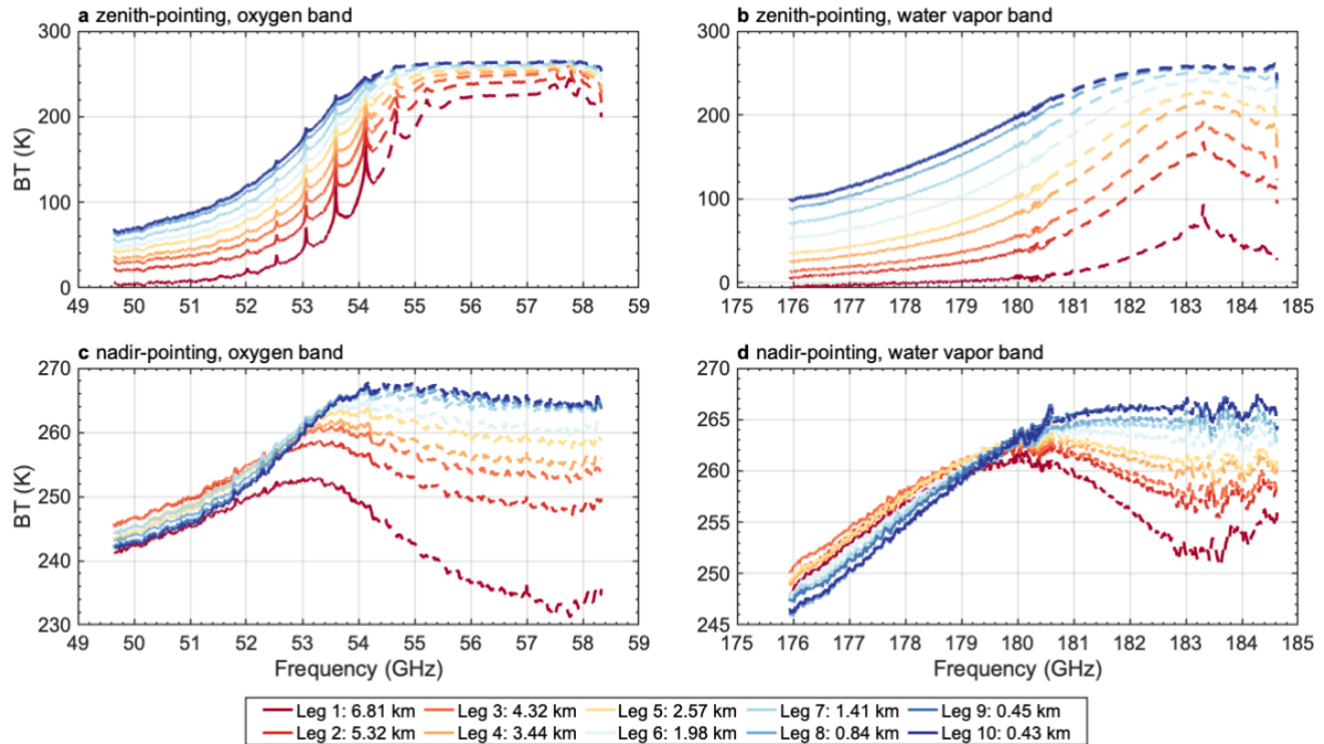
175 Figure 5. HiSRAMS-observed spectra during FC2023 flights at different altitudes. Solid lines are for FFT0 measurements and dashed lines are for FFT1 measurements. (a, b) Zenith-pointing and (c, d) Nadir-pointing spectra in the oxygen and the water vapor band, respectively.
