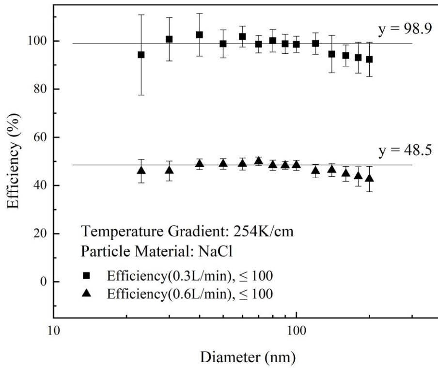
450 Figure 8. The measured TPAE particle collection efficiency as a function of the NaCl particle size for the sampling flow rate of 0.3 and 0.6 L/min.
