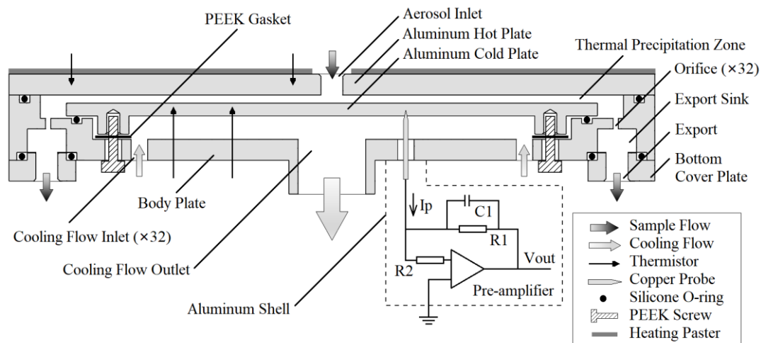
100 Key Figure: Schematic diagram of the prototype Thermal Precipitation Aerosol Electrometer (TPAE)
