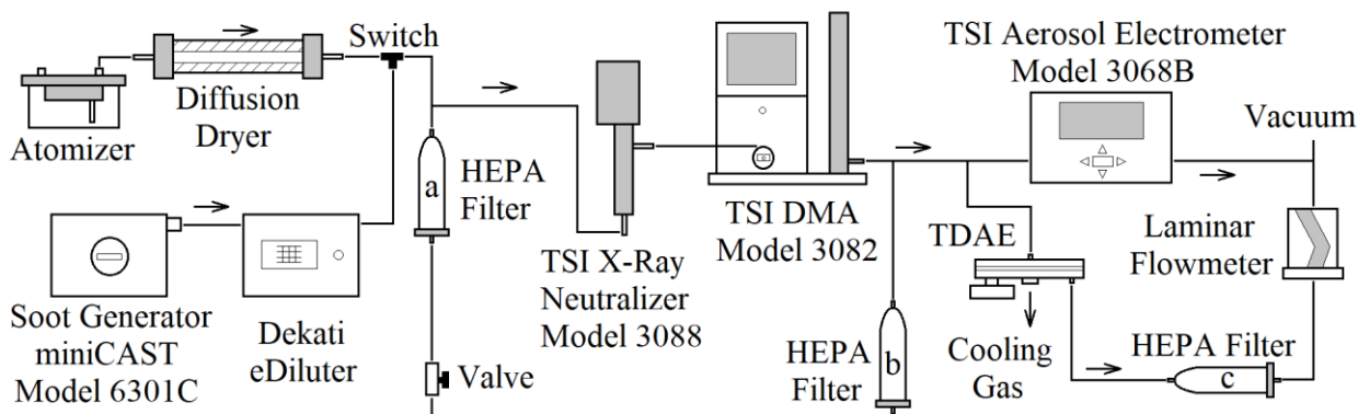
425 Figure 2. Schematic diagram of experimental setup for the TPAE performance evaluation.
