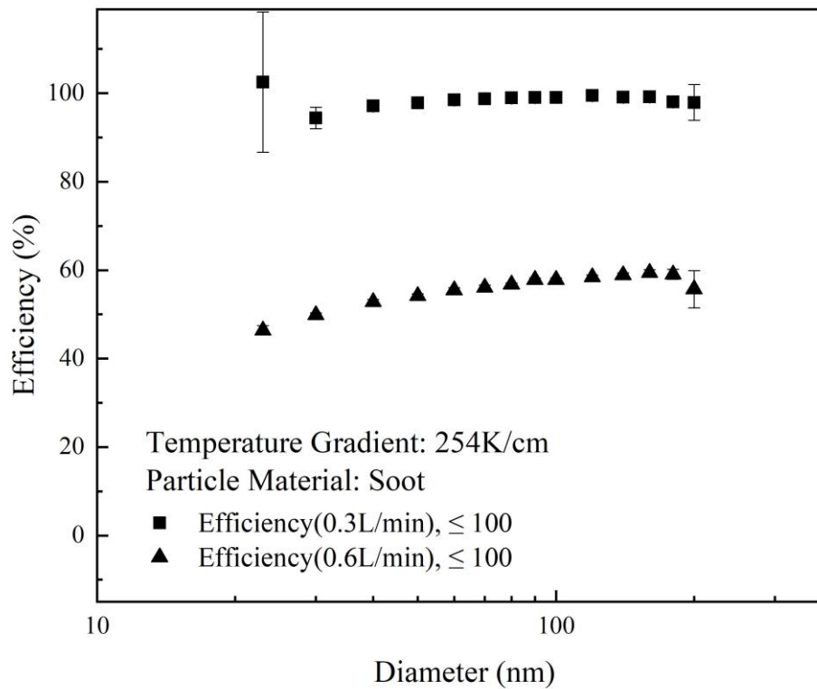
Figure 9. The measured TPAE particle collection efficiency as a function of the soot particle size for the sampling flow rate of 0.3 and 0.6 L/min.
