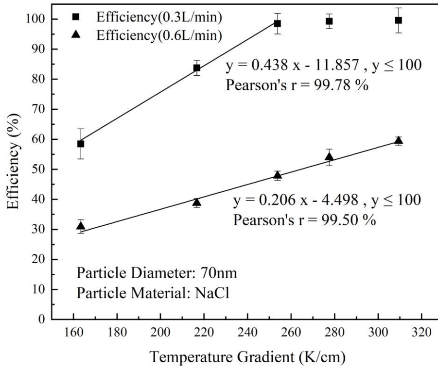
440 Figure 6. Calibration of collection efficiency and temperature gradient.
