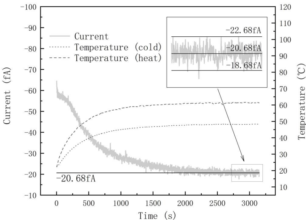
Figure 3. The readout of TPAE during the warm-up process (particle-free air was used).
