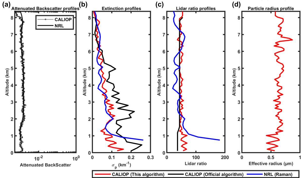
461 Figure 9. 532 nm and 1064 nm attenuated backscatter profiles measured by CALIOP (black solid line with 462 circle marker) and NRL (remodeling, black solid line) on 20 August 2006 in logarithmic scale in horizontal 463 direction (a); (b, c, d) show the extinction profiles, lidar ratio profiles and particle radius profiles, respectively, 464 provided by our inversion algorithm (red), CALIOP operational level 2 product (black) and EARLINET level 465 2 product (blue).
