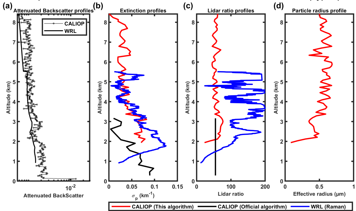
495 Figure 18. 532 nm and 106 nm attenuated backscatter profiles measured by CALIOP (black solid line with 496 circle marker) and WRL at the Warsaw station (remodeling, black solid line) on 20 August 2006 in 497 logarithmic scale in horizontal direction (a); (b, c, d) show the extinction profiles, lidar ratio profiles and 498 particle radius profiles, respectively, provided by the modified inversion algorithm (red), CALIOP level 2 499 (black) and EARLINET level 2 (blue).
