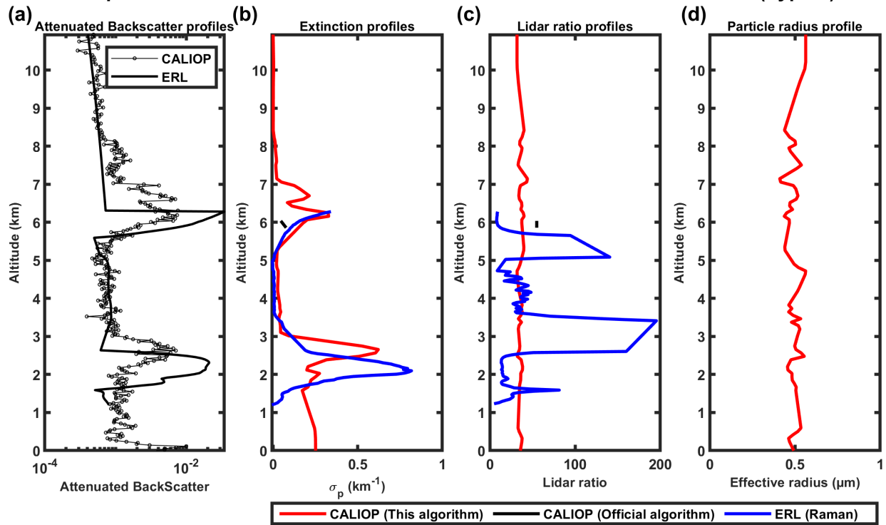
483 Figure 15. 532 nm and 106 nm attenuated backscatter profiles measured by CALIOP (black solid line with 484 circle marker) and ERL at the Evora station (remodeling, black solid line) on 20 August 2006 in logarithmic 485 scale in horizontal direction (a); (b, c, d) show the extinction profiles, lidar ratio profiles and particle radius 486 profiles, respectively, provided by the modified inversion algorithm (red), CALIOP level 2 (black) and 487 EARLINET level 2 (blue).
