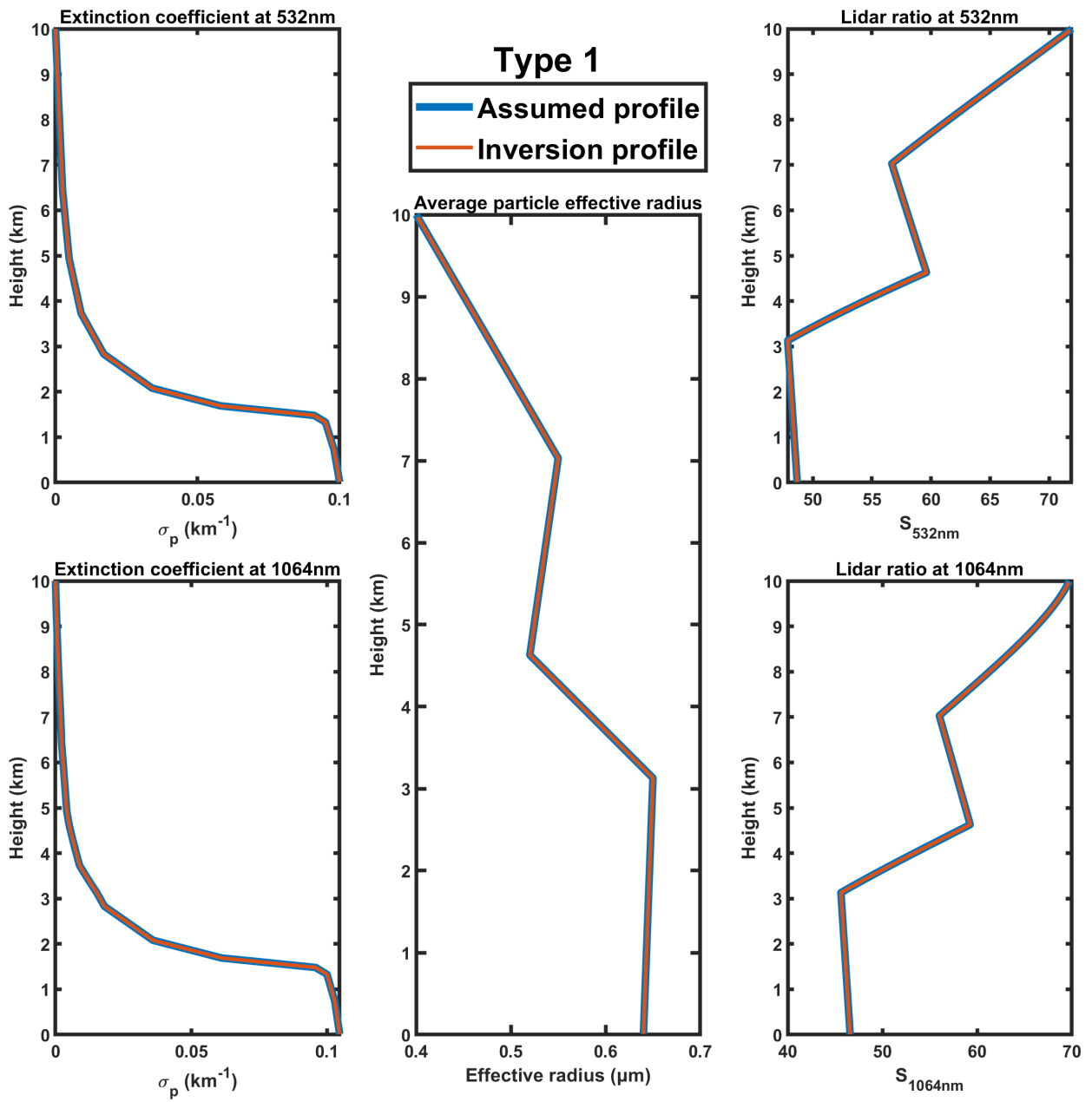
445 Figure 4. The result of the inversion algorithm using the synthetic data shown in Figure 3.
