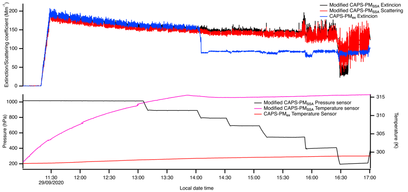
Figure 6. \sigma_{\text{ext}} measured by CAPS-PM ext at 630 nm, and \sigma_{\text{ext}} and \sigma_{\text{sca}} measured by CAPS-PM SSA at several pressures; the temperature changes were applied to the CAPS-PM SSA .
