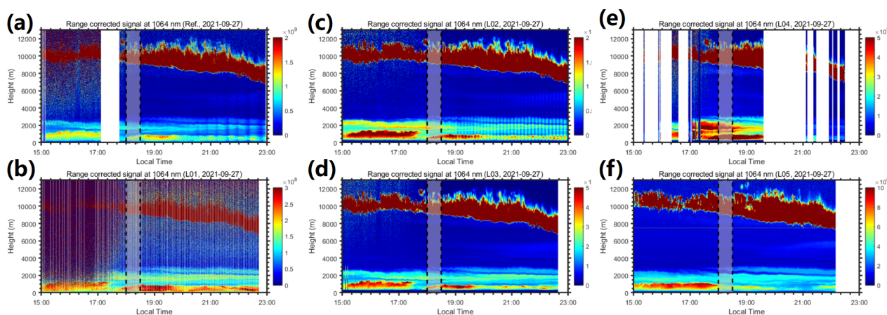
Figure 5. Quick looks of aerosol loading observation from different lidar measurements on 27 September 2021 between 15:00 and 23:00 CST. The grey rectangle shadows indicate the selected periods for single profile inter-comparison between 18:30 and 19:00 CST. The RCS at 1064 nm were taken from (a) reference lidar system, (b) L01 lidar system, (c) L02 lidar system, (d) L03 lidar system, (e) L04 lidar system (the multiple interruptions were caused by the operation issue during the measurement) and (f) L05 lidar system. All data was sampled in 1 min temporal resolution and to 15 m range resolution.
