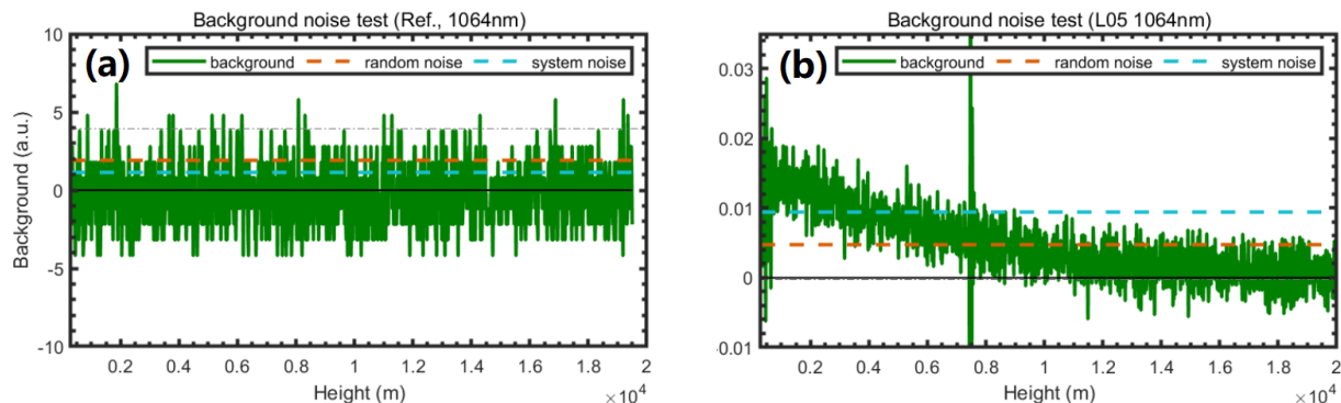
Figure 8. The background noise test results of the photon counting SPAD and analog APD detectors. The green lines indicate the background noise directly collected by lidar system. The orange dash lines was the standard deviation of background noise, which was defined as random noise. The sky blue dash lines was the maximum deviation of the mean background noise within a 500 m range widow to the mean background noise of all data points, which was defined as system noise. The horizontal black lines indicate the value of zero. (a) the test result from lidar No.Ref., (b) the test result from lidar No.L05.
