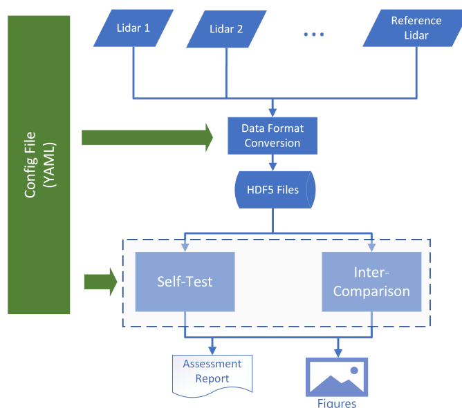
Figure 2. Software structure of Atmospheric Lidar Evaluation program for 1064 nm atmospheric lidar inter-comparison, in which "YAML" standards for human-readable data-serialization language and was widely used for cross-platform software configurations. "HDF5" stands for Hierarchical Data Format, which was commonly used for atmospheric data storage.
