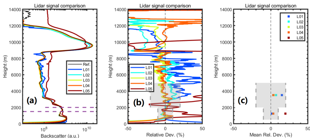
Figure 6. The inter-comparison results for RCSs from all the lidar systems in the periods of 18:30 and 19:00 CST on 27 September 2021. The horizontal dash lines indicate the adopted normalization window for each RCSs. The vertical dash lines in the middle indicate zero relative deviation. The rectangle shadows indicate 10 % of relative deviation within 500-2000 m and 20 % of relative deviation within 2000-5000 m. (a) normalized RCS profiles, (b) the profiles of relative deviations of lidar No.L01-L05 with the No.Ref., (c) the mean relative deviations of lidar No.L01-L05 with No.Ref..
