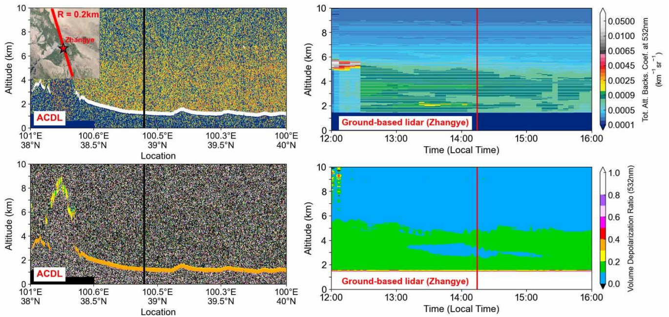
480 Figure 4: Vertical structure of atmospheric aerosols and clouds observed via the ACDL and ground-based lidar on a clear day on 24 July 2022. The closest distance between the ACDL track and the ground-based lidar is 0.2 km. The ACDL overpass time is 14:24 LT.
