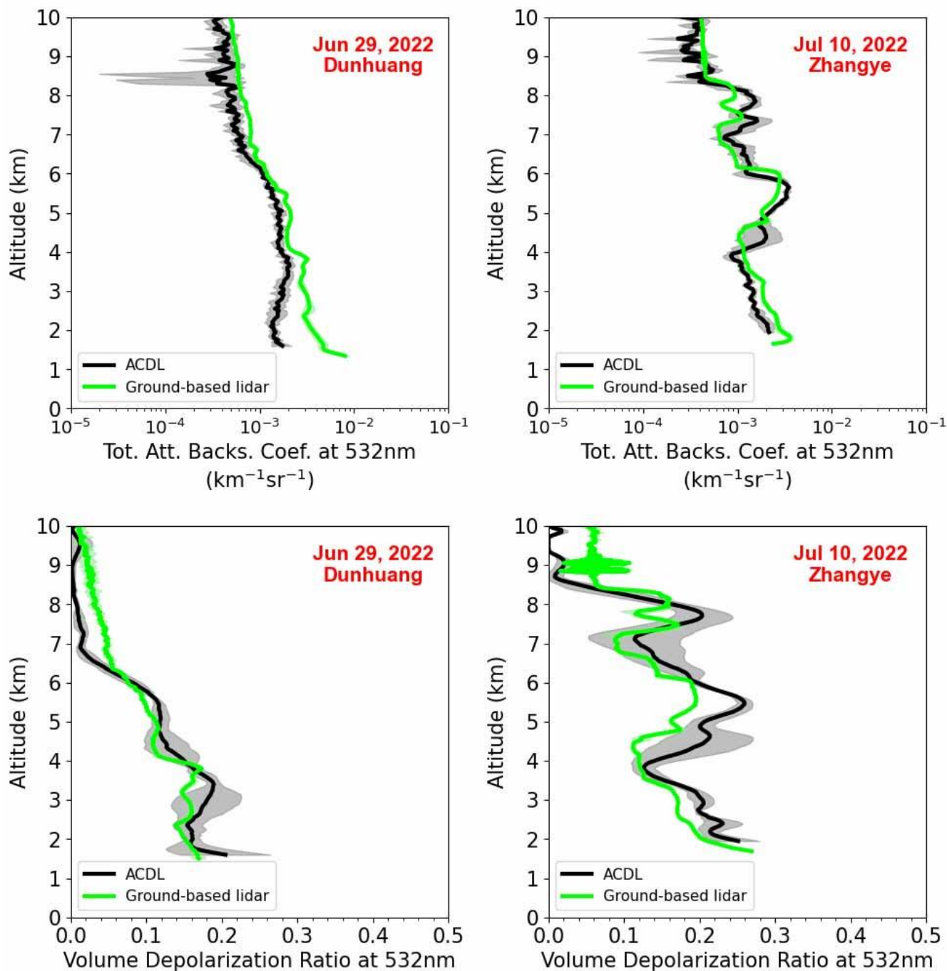
500 Figure 8: Comparison between the TABC and VDR profiles at 532 nm measured by the ACDL and ground-based lidar on 29 June 2022 and 10 July 2022 respectively. The shaded envelope represents the standard deviation.
