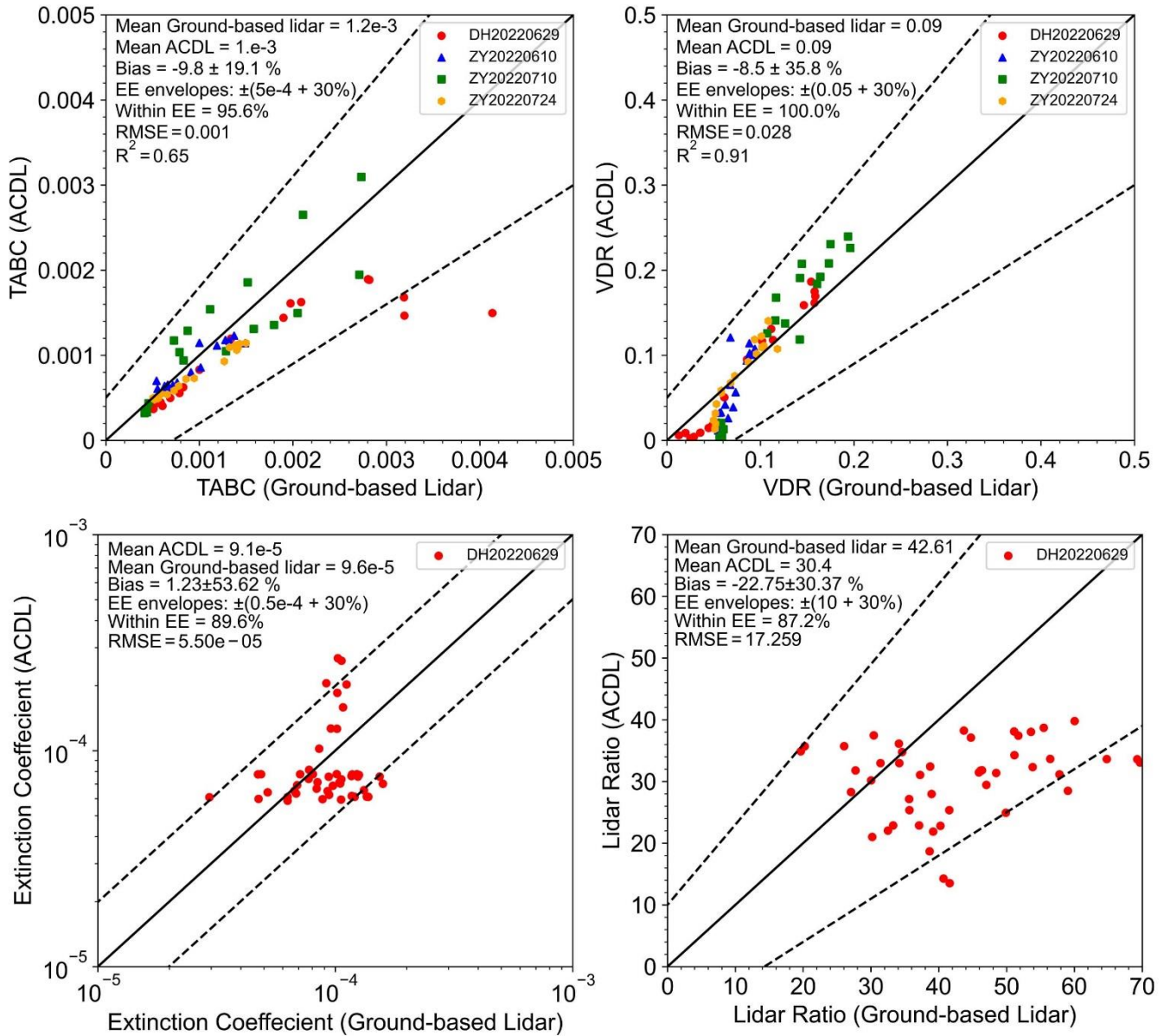
520 Figure 13: Scatterplots of the ground-based lidar retrieved TABC (upper left) and VDR (upper right) versus ACDL measurement under cloud-free conditions. The solid line refers to the 1:1 line; the dashed line refers to the expected error envelope; EE = \pm(0.0005 + 0.3 \times \text{TABC}_{\text{Ground}}) ; EE = \pm(0.05 + 0.3 \times \text{VDR}_{\text{Ground}}) . The two panels below the figure show the comparison between the extinction coefficient and lidar ratio obtained from ACDL and ground-based lidar retrieval under the dust case on June 29th. The solid line refers to the 1:1 line; the dashed line refers to the expected error envelope; EE = \pm(0.5 \times 10^{-4} + 0.3 \times \text{Ext}_{\text{Ground}}) ; EE = \pm(10 + 0.3 \times \text{LR}_{\text{Ground}}) .
