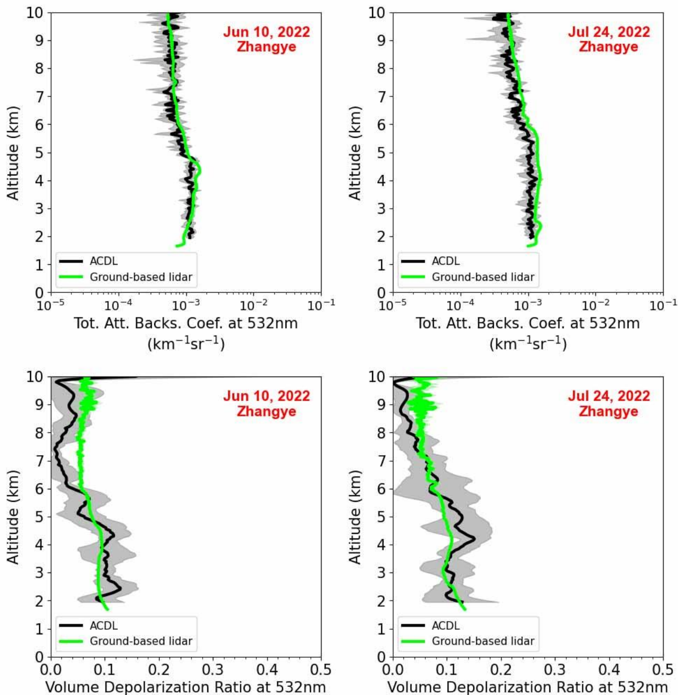
485 Figure 5: Comparison between the TABC and VDR profiles at 532 nm measured by the ACDL (black solid line) and ground-based lidar (lime solid line) on 10 June 2022 and 24 July 2022. The shaded envelope represents the standard deviation.
