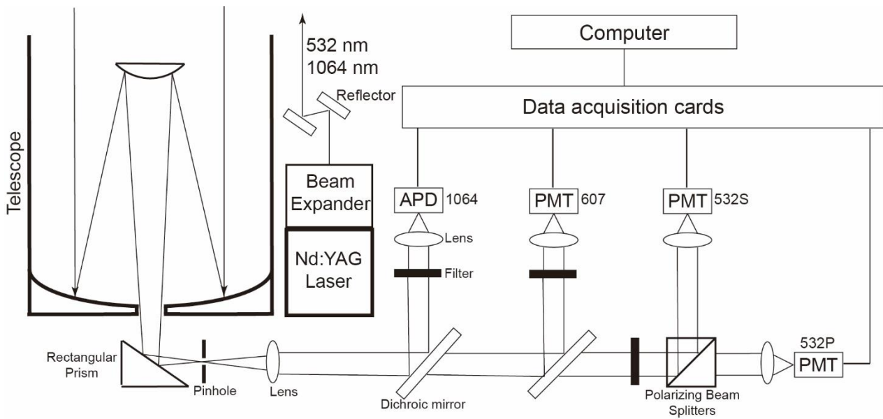
465 Figure 1: Schematic diagram of the developed ground-based lidar system of the BR-lidarnet employed in the present investigation.
