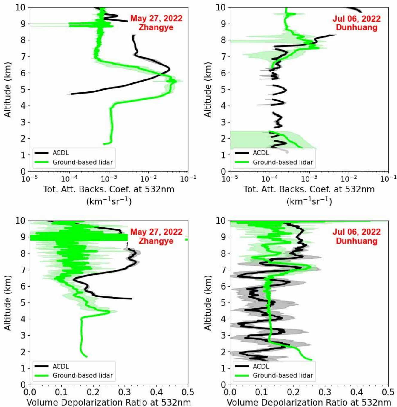
515 Figure 12: Comparison between the TABC and VDR profiles at 532 nm measured by the ACDL (black solid line) and ground-based lidar (lime solid line) on 27 May 2022 and 6 July 2022 respectively. The shaded envelope represents the standard deviation.
