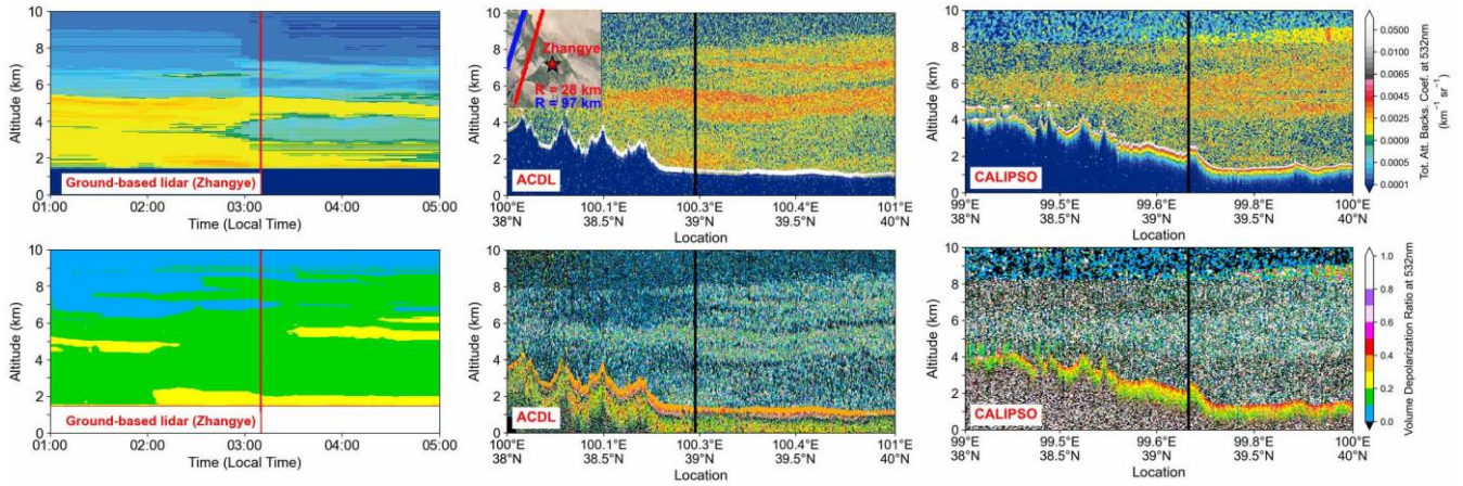
495 Figure 7: Vertical structure of atmospheric aerosols and clouds observed via the ground-based lidar (left), ACDL (centre), and CALIPSO (right) on July 10, 2022. The closest distance between the ACDL track (red line) and the Zhangye lidar site is 28 km. The ACDL overpass time is 3:16 LT. The closest distance between the ACDL track and the CALIPSO track (blue line) is 68.65 km.
