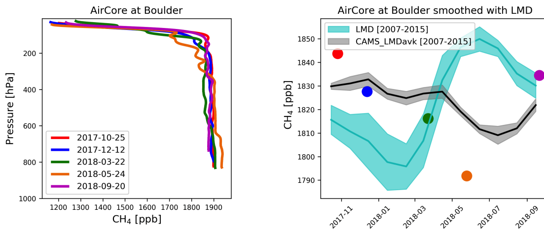
Figure 22. Left: the AirCore \text{CH}_4 profiles at Boulder between October 2017 and September 2018. Right: the time series of the \text{mtCH}_4 derived from the AirCore measurements with the smoothing correction using LMD weighting function, together with the \text{mtCH}_4 seasonal variation derived from LMD measurements between July 2007 and June 2015 with a constant shift using the mean of the 5 AirCore measurements. CAMS_LMDavk corresponds with CAMS model data at Boulder smoothed by the LMD weighting function.
