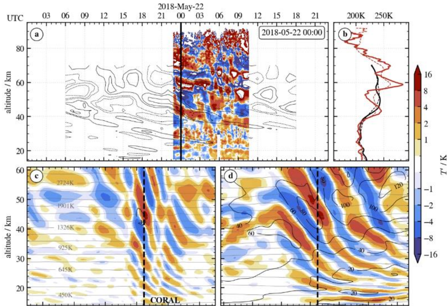
a) Temperature perturbations observed by CORAL on the night of 21-22 May 2018. Contour lines indicate temperature perturbations from ERA5. b) Obtained CORAL (red) and ERA5 (black) temperature profiles at 00UTC. c) Zonal crosssection of ERA5 temperature perturbations. d) Meridional crosssection of ERA5 temperature perturbations. Dashed lines in c) and d) mark the CORAL location.
