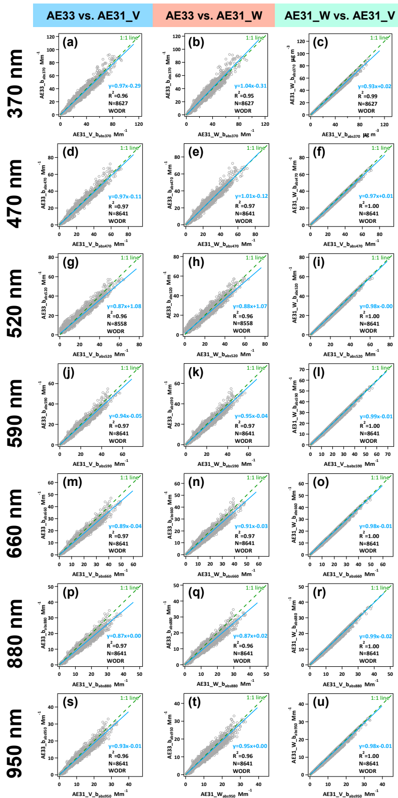
Figure 3. Comparison of hourly light absorption coefficient between AE33 and AE31 at 370, 470, 520, 590, 660, 880 and 950 nm. AE31_V_b abs and AE31_W_b abs represent light absorption coefficients of
