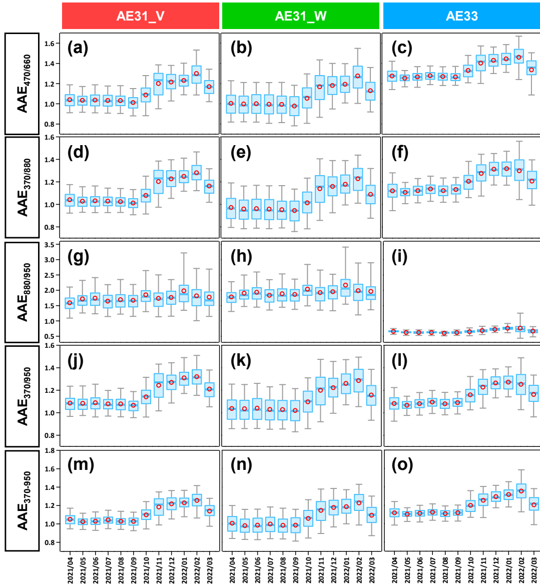
930 Figure 6. Monthly variations of different AAE values (AAE 470/660 , AAE 370/880 , AAE 880/950 , AAE 370/950 and AAE 370-950 ) calculated using 1-hr data from AE31_V, AE31_W and AE33.
