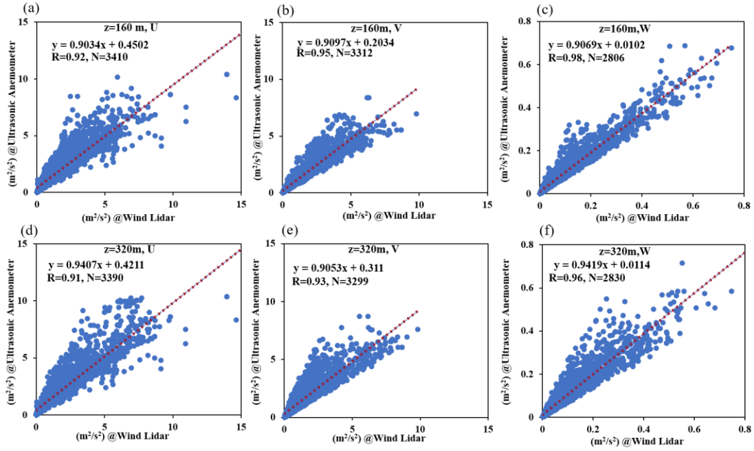
Figure 11. Correlation between the turbulent kinetic energy obtained with the wind lidar and three-dimensional ultrasonic anemometer in the U , V , and W directions at the heights of 160 m (a)–(c) and 320 m (d)–(f).
