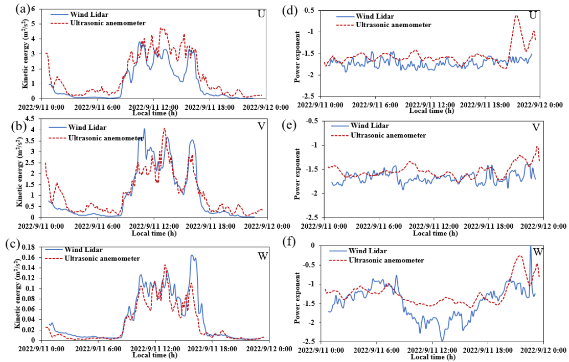
Figure 7. Comparison of the turbulent kinetic energy obtained by the wind lidar and three-dimensional ultrasonic anemometer on September 11, 2022 in the (a) U , (b) V , and (c) W directions and the power-law exponent distribution in the (d) U , (e) V , and (f) W directions.
