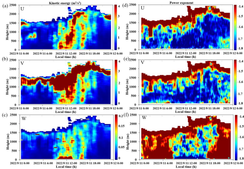
Figure 6. Temporal and spatial variations of the turbulent kinetic energy obtained by wind lidar on September 11, 2022 in the (a) U , (b) V , and (c) W directions and the power-law exponent distribution in the (d) U , (e) V , and (f) W directions.
