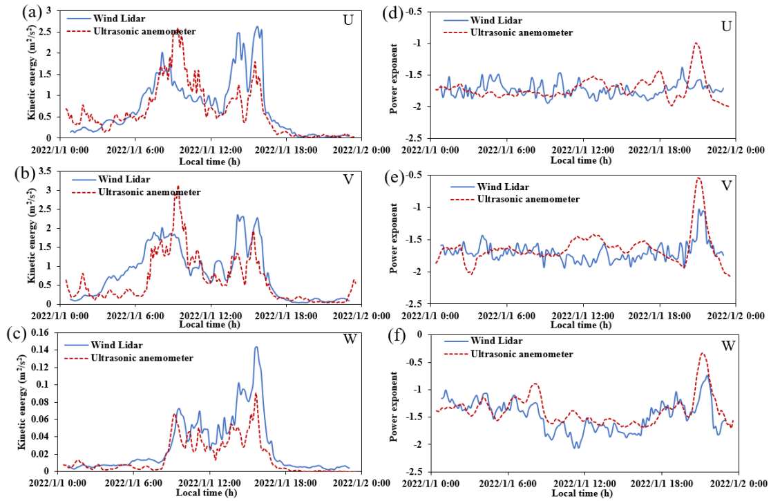
245 Figure 3. Comparison of the turbulent kinetic energy obtained from the wind lidar and three-dimensional ultrasonic anemometer on January 1, 2022 in the (a) U , (b) V , and (c) W directions and the power-law exponent distribution in the (d) U , (e) V , and (f) W directions.
