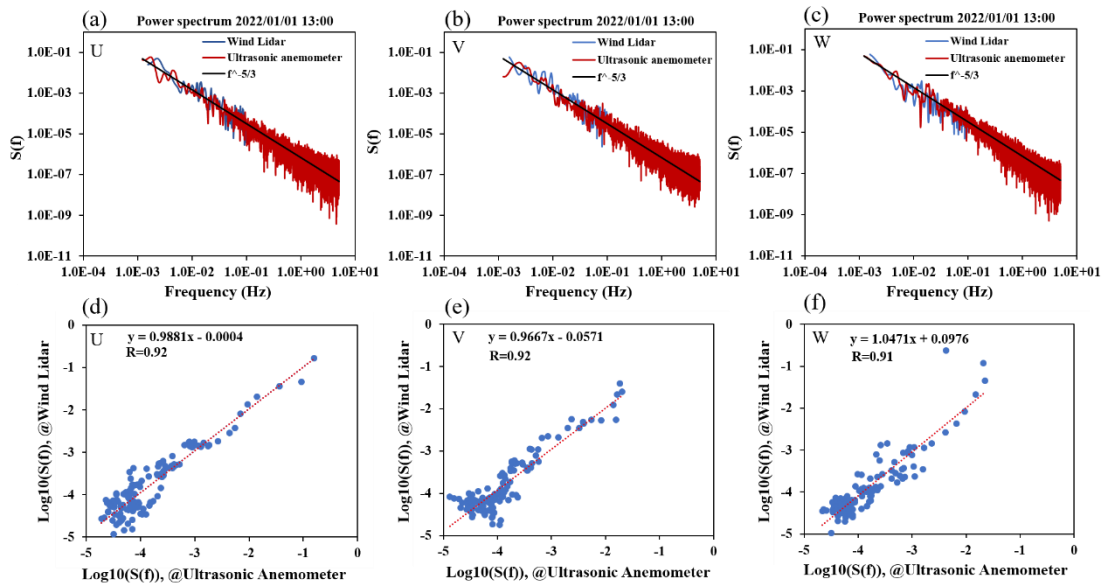
210 Figure 2. Comparison of the turbulence spectra obtained with the wind lidar and the ultrasonic anemometer in three directions: (a) U , (b) V , and (c) W , and the corresponding correlations (d), (e), and (f).
