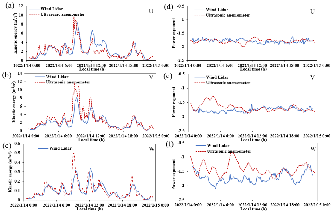
Figure 9. Comparison of turbulent kinetic energy obtained by the wind lidar and three-dimensional ultrasonic anemometer on January 14, 2022 in the (a) U , (b) V , and (c) W directions and the power-law exponent distribution in the (d) U , (e) V , and (f) W directions.
