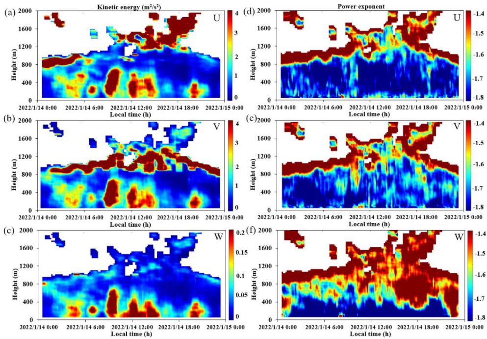
Figure 8. Temporal and spatial variations of the turbulent kinetic energy obtained by wind lidar on January 14, 2022 in the (a) U , (b) V , and (c) W directions and the power-law exponent distribution in the (d) U , (e) V , and (f) W directions.
