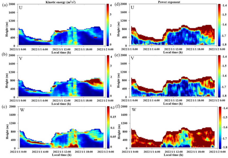
Figure 4. Temporal and spatial variations of the turbulent kinetic energy obtained by wind lidar on January 1, 2022 in the (a) U , (b) V , and (c) W directions and the power-law exponent distribution in the (d) U , (e) V , and (f) W directions.
